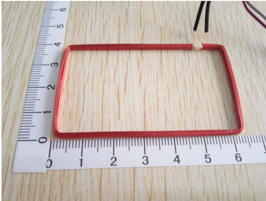
Antenna for 125KHz
