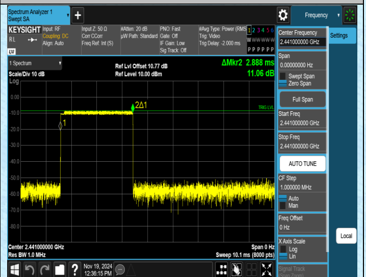
2DH5-Ant1-Hop-PASS
