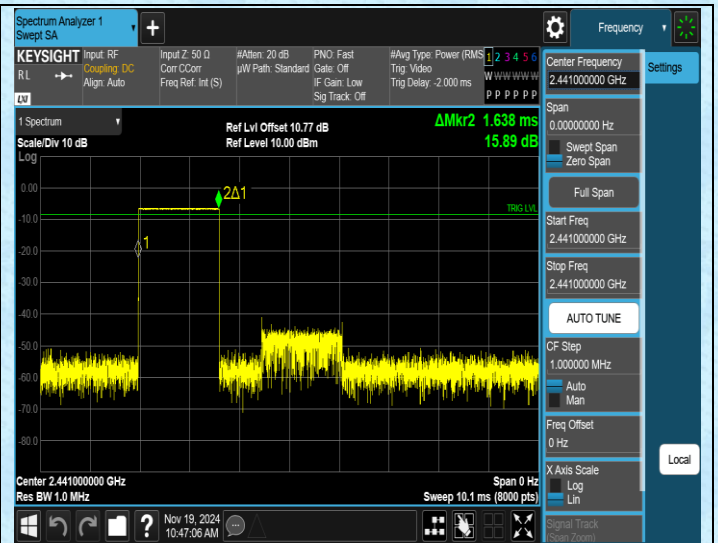
DH3-Ant1-Hop-PASS
