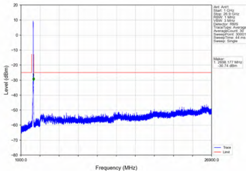
n41_30kHz_SISO_NTNV_50MHz_DFT-s-OFDM_QPSK_2664.99MHz_Inner_1RB_Right
