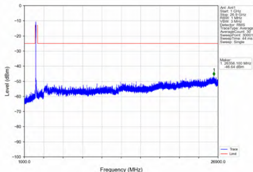
n41_30kHz_SISO_NTNV_60MHz_CP-OFDM QPSK_2526MHz_Outer_Full
