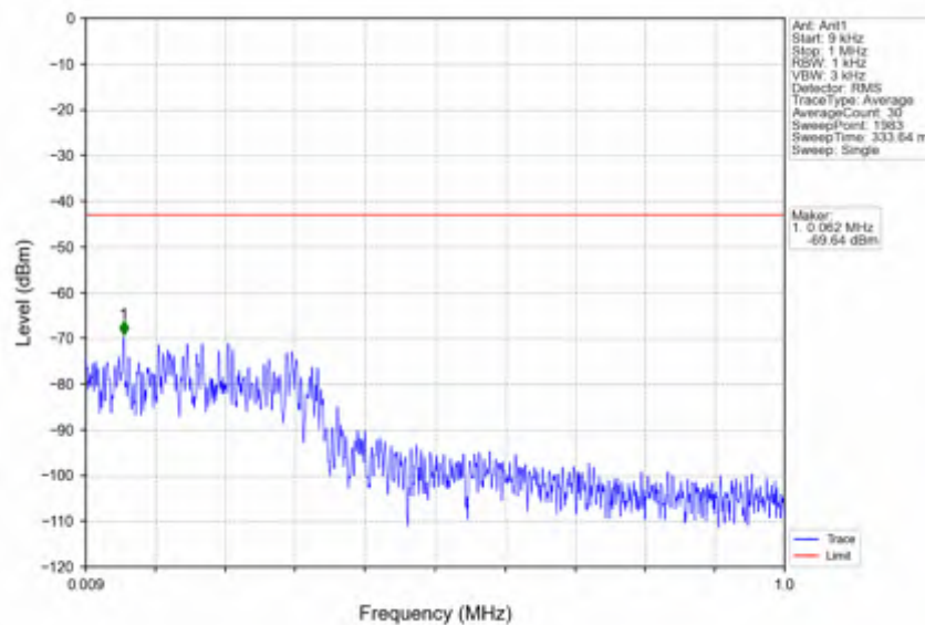
n41_30kHz_SISO_NTNV_90MHz_DFT-s-OFDM QPSK_2592.99MHz_Edge_1RB_Left
