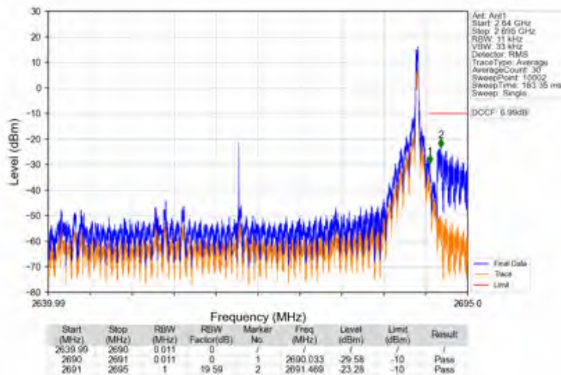
n41_30kHz_SISO_NTNV_50MHz_DFT-s-OFDM_QPSK_2664.99MHz_Inner_1RB_Right
