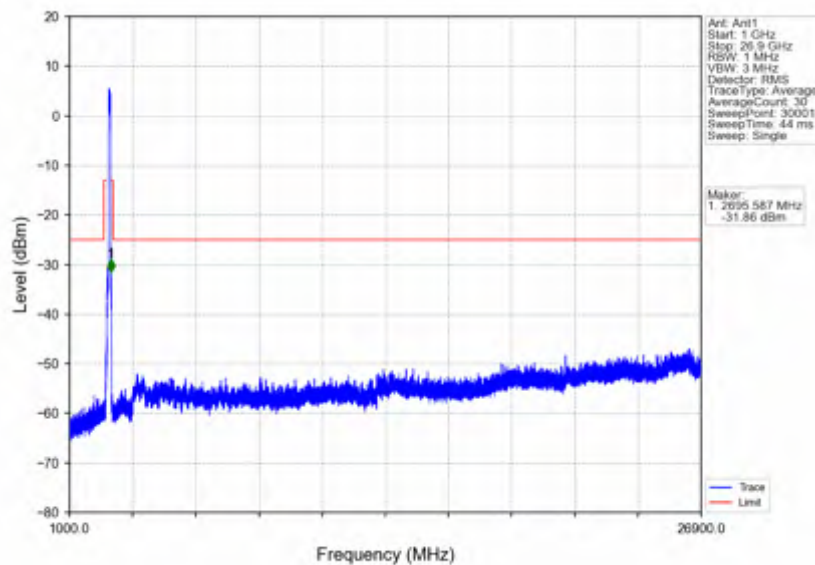
n41_30kHz_SISO_NTNV_90MHz_DFT-s-OFDM_QPSK_2644.98MHz_Inner_1RB_Right
