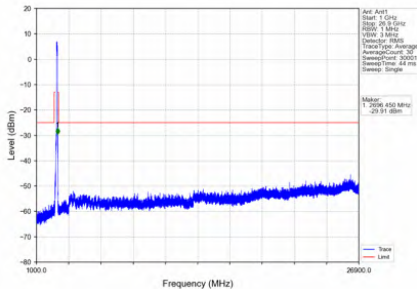
n41_30kHz_SISO_NTNV_80MHz_CP-OFDM QPSK_2649.99MHz_Outer_Full
