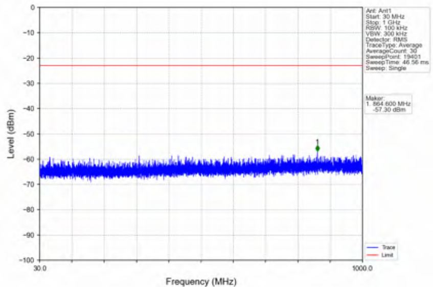
n41_30kHz_SISO_NTNV_50MHz_DFT-s-OFDM QPSK_2592.99MHz_Edge_1RB_Left
