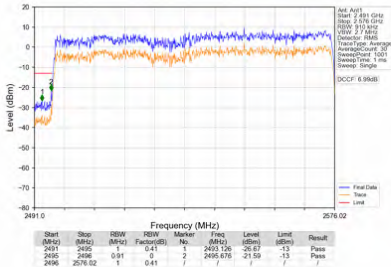
n41_30kHz_SISO_NTNV_80MHz_CP-OFDM_QPSK_2536.02MHz_Outer_Full
