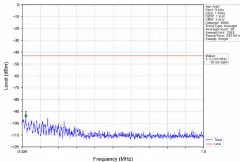
n41_30kHz_SISO_NTNV_50MHz_CP-OFDM QPSK_2664.99MHz_Inner_1RB_Right
