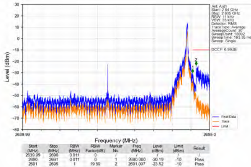
n41_30kHz_SISO_NTNV_50MHz_CP-OFDM QPSK_2664.99MHz_Inner_1RB_Right
