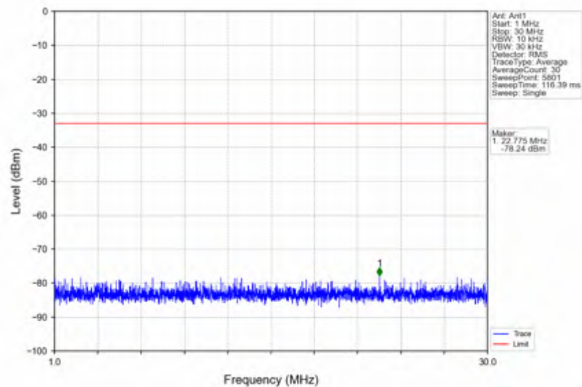
n41_30kHz_SISO_NTV_60MHz_CP-OFDM_QPSK_2526MHz_Outer_Full
