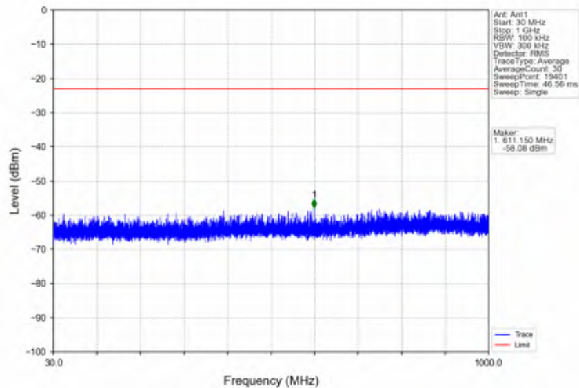
n41_30kHz_SISO_NTNV_50MHz_DFT-s-OFDM_QPSK_2521.02MHz_Edge_1RB_Left
