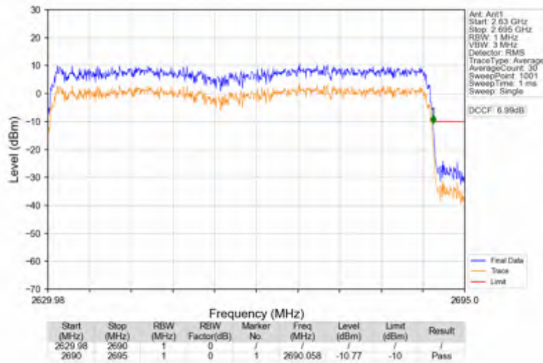
n41_30kHz_SISO_NTNV_60MHz_CP-OFDM QPSK_2659.98MHz_Outer_Full
