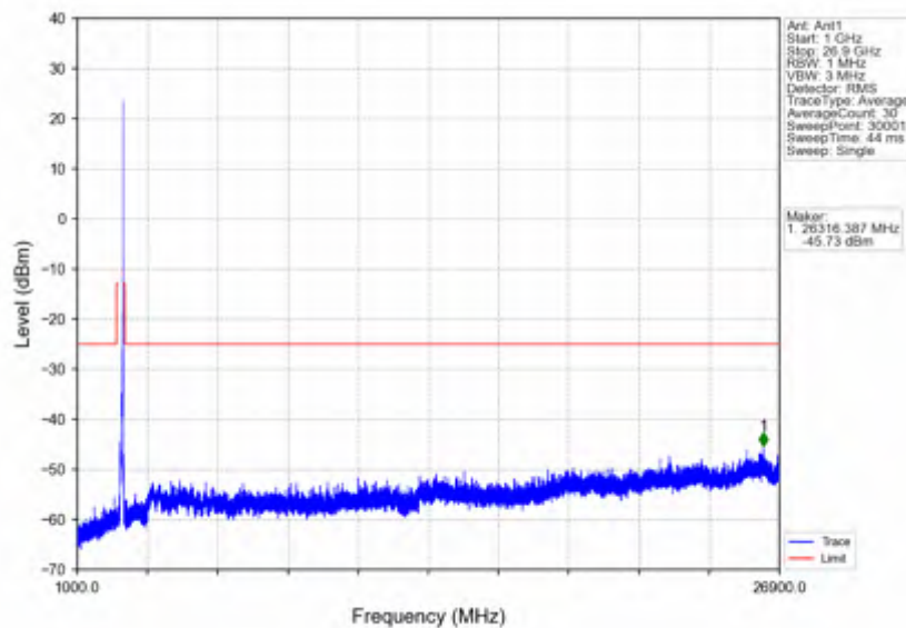
n41_30kHz_SISO_NTNV_60MHz_CP-OFDM QPSK_2659.98MHz_Outer_Full
