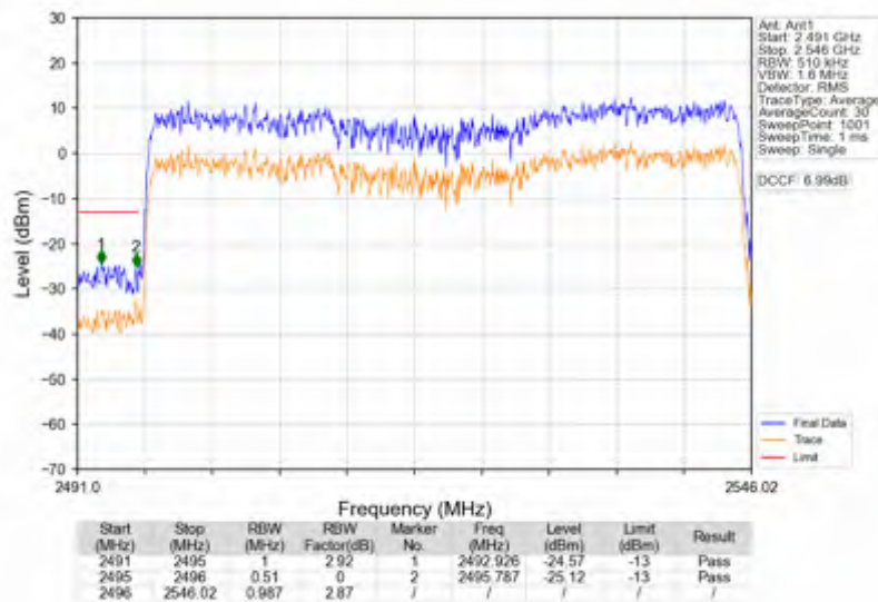
n41_30kHz_SISO_NTNV_50MHz_CP-OFDM QPSK_2521.02MHz_Outer_Full
