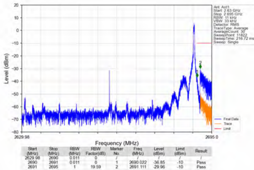
n41_30kHz_SISO_NTNV_60MHz_DFT-s-OFDM_QPSK_2659.98MHz_Edge_1RB_Right
