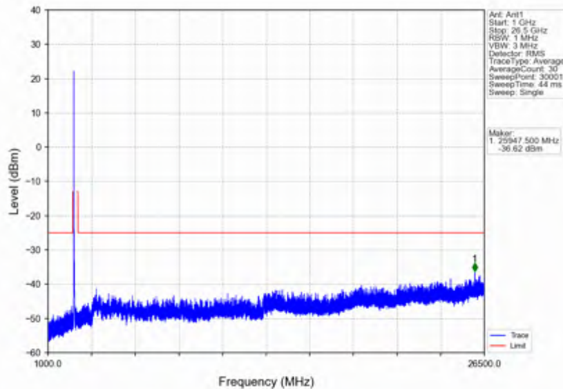
n41_30kHz_SISO_NTNV_50MHz_DFT-s-OFDM_QPSK_2521.02MHz_Edge_1RB_Left
