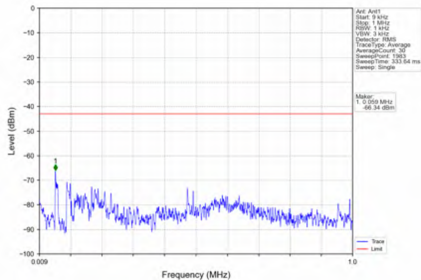
n41_30kHz_SISO_NTNV_80MHz_CP-OFDM QPSK_2649.99MHz_Outer_Full
