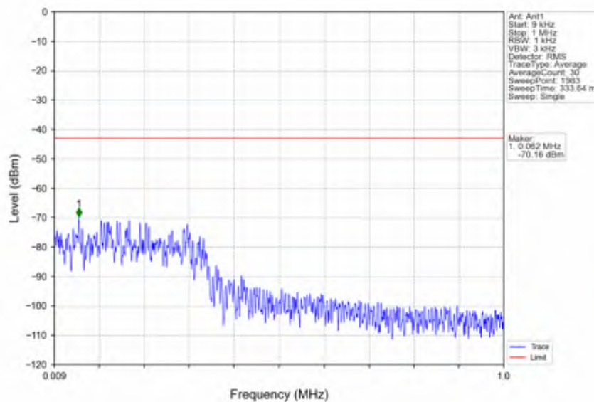
n41_30kHz_SISO_NTNV_80MHz_DFT-s-OFDM_QPSK_2592.99MHz_Edge_1RB_Left
