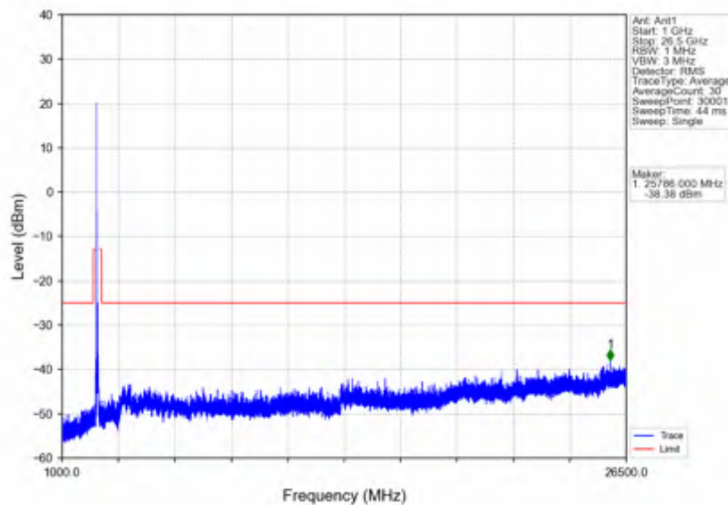
n41_30kHz_SISO_NTNV_90MHz_DFT-s-OFDM_QPSK_2644.98MHz_Edge_1RB_Right
