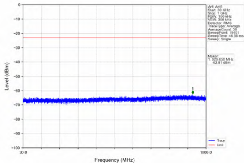
n41_30kHz_SISO_NTNV_90MHz_DFT-s-OFDM_PI/2_BPSK_2541MHz_Outer_Full
