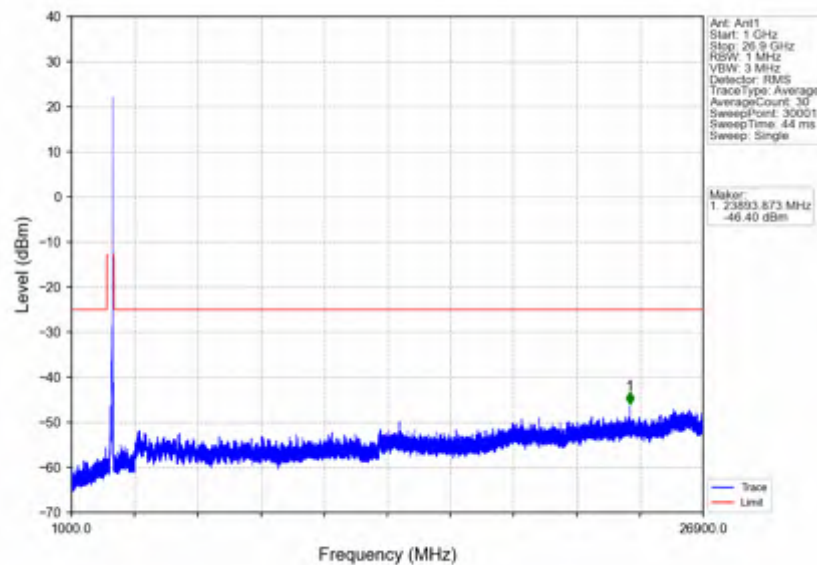
n41_30kHz_SISO_NTNV_50MHz_DFT-s-OFDM QPSK_2664.99MHz_Edge_1RB_Right
