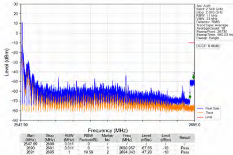
n41_30kHz_SISO_NTNV_90MHz_DFT-s-OFDM QPSK_2592.99MHz_Edge_1RB_Left
