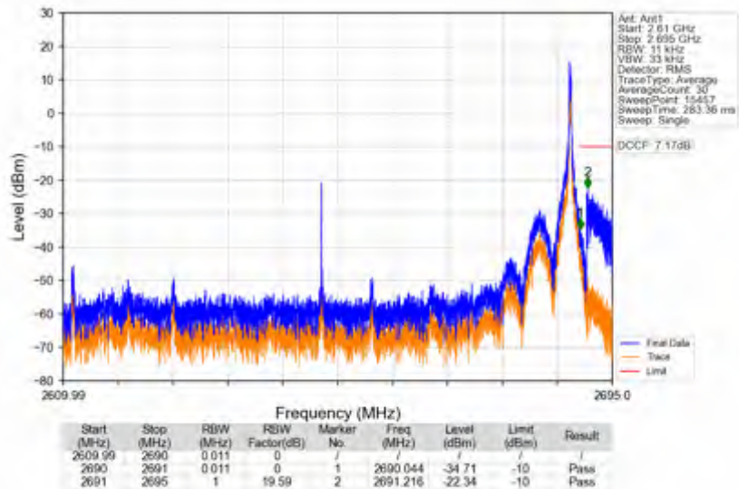
n41_30kHz_SISO_NTNV_80MHz_DFT-s-OFDM QPSK_2649.99MHz_Inner_1RB_Right
