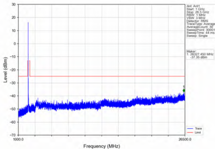
n41_30kHz_SISO_NTNV_60MHz_CP-OFDM QPSK_2526MHz_Outer_Full
