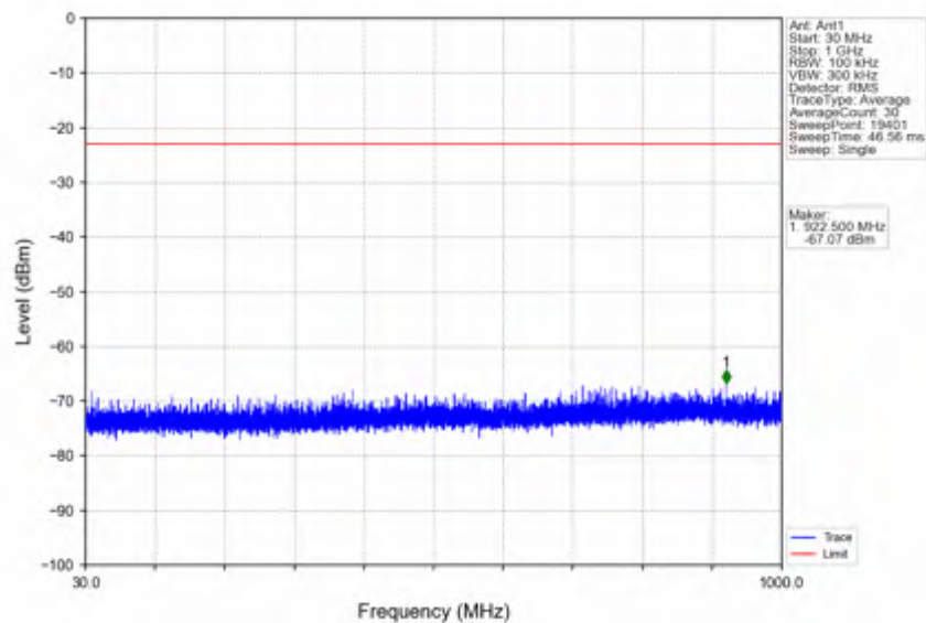
n41_30kHz_SISO_NTNV_50MHz_CP-OFDM QPSK_2664.99MHz_Inner_1RB_Right
