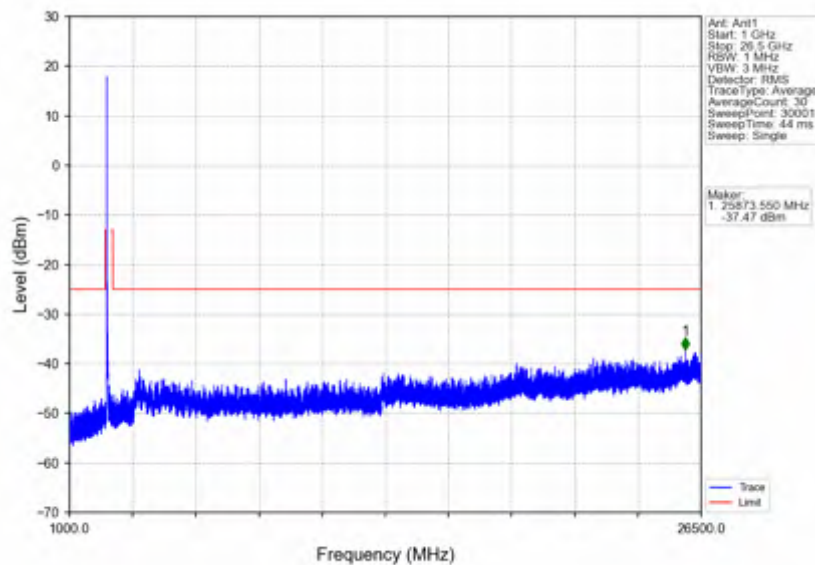
n41_30kHz_SISO_NTNV_50MHz_CP-OFDM QPSK_2521.02MHz_Outer_Full
