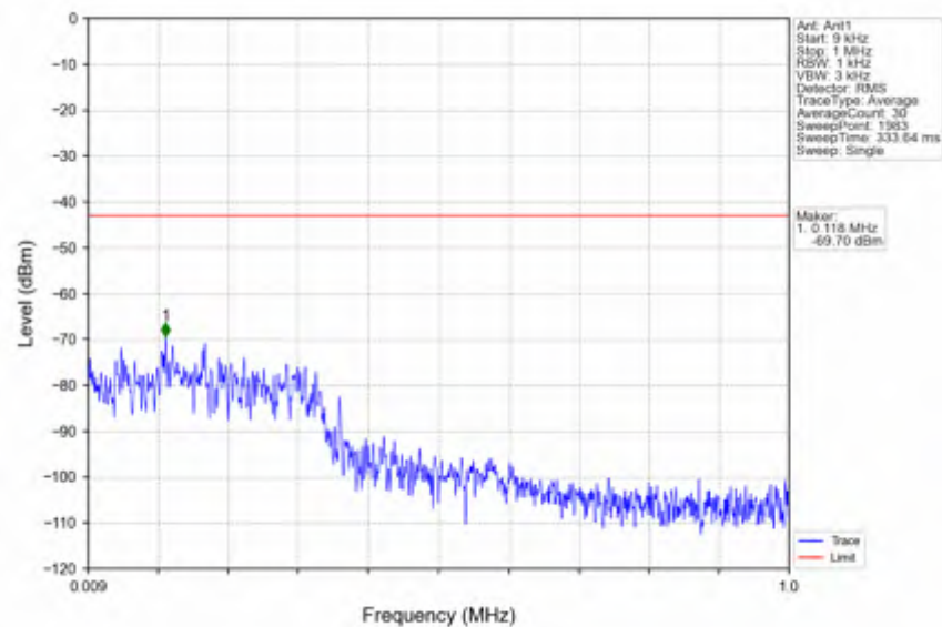
n41_30kHz_SISO_NTNV_60MHz_DFT-s-OFDM QPSK_2659.98MHz_Edge_1RB_Right
