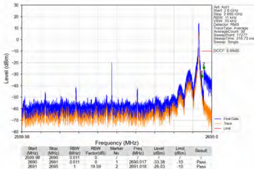
n41_30kHz_SISO_NTNV_90MHz_DFT-s-OFDM_QPSK_2644.98MHz_Inner_1RB_Right
