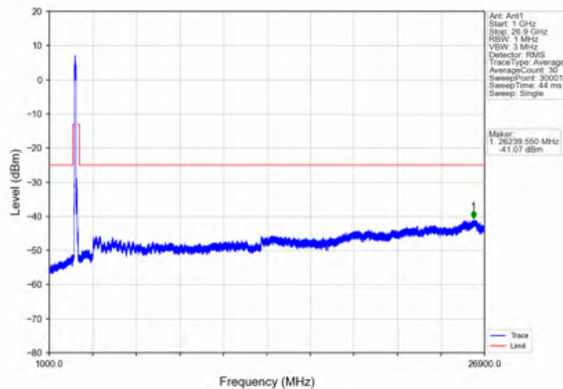
n41_30kHz_SISO_NTNV_90MHz_DFT-s-OFDM_PI/2_BPSK_2541MHz_Outer_Full
