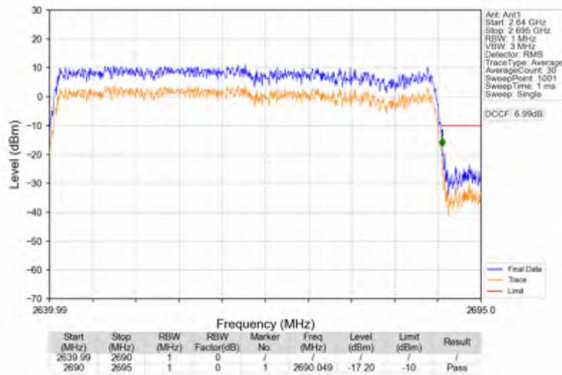
n41_30kHz_SISO_NTNV_50MHz_CP-OFDM QPSK_2664.99MHz_Outer_Full
