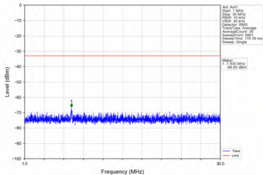
n41_30kHz_SISO_NTNV_50MHz_CP-OFDM QPSK_2592.99MHz_Edge_1RB_Left
