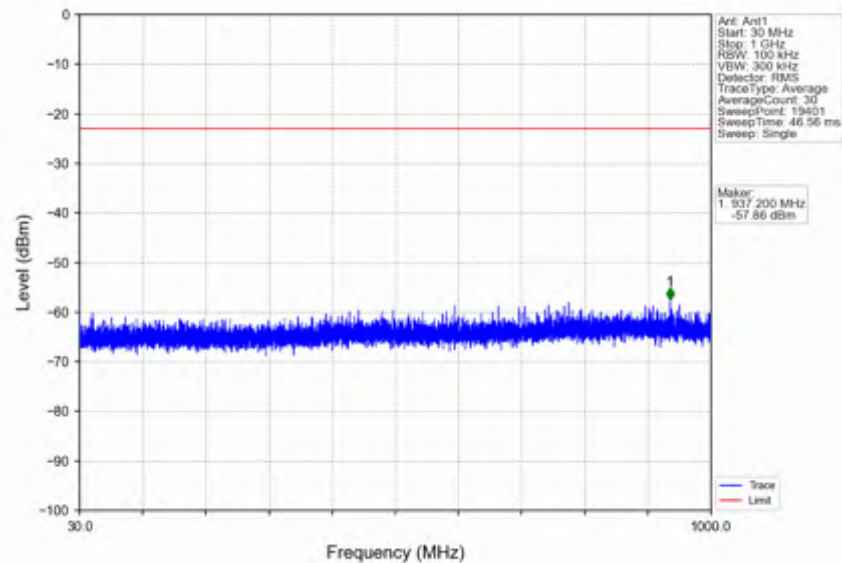
n41_30kHz_SISO_NTNV_80MHz_DFT-s-OFDM QPSK_2536.02MHz_Edge_1RB_Left
