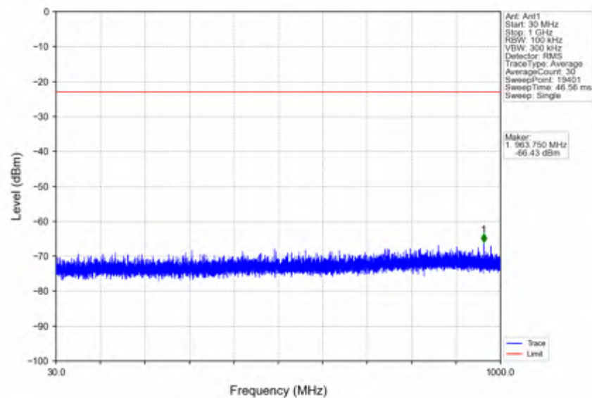
n41_30kHz_SISO_NTNV_50MHz_DFT-s-OFDM QPSK_2521.02MHz_Outer_Full
