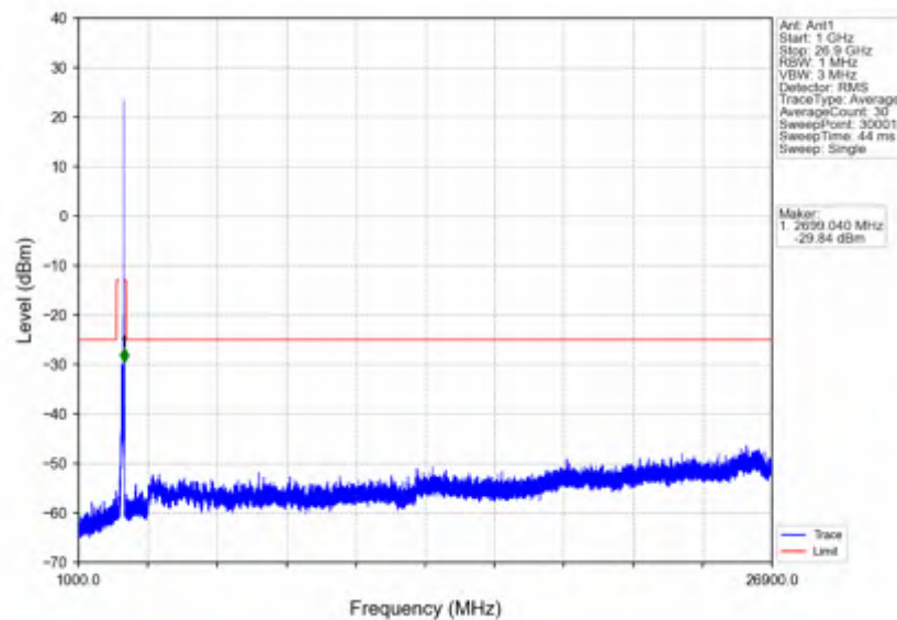
n41_30kHz_SISO_NTNV_80MHz_DFT-s-OFDM_QPSK_2649.99MHz_Inner_1RB_Right
