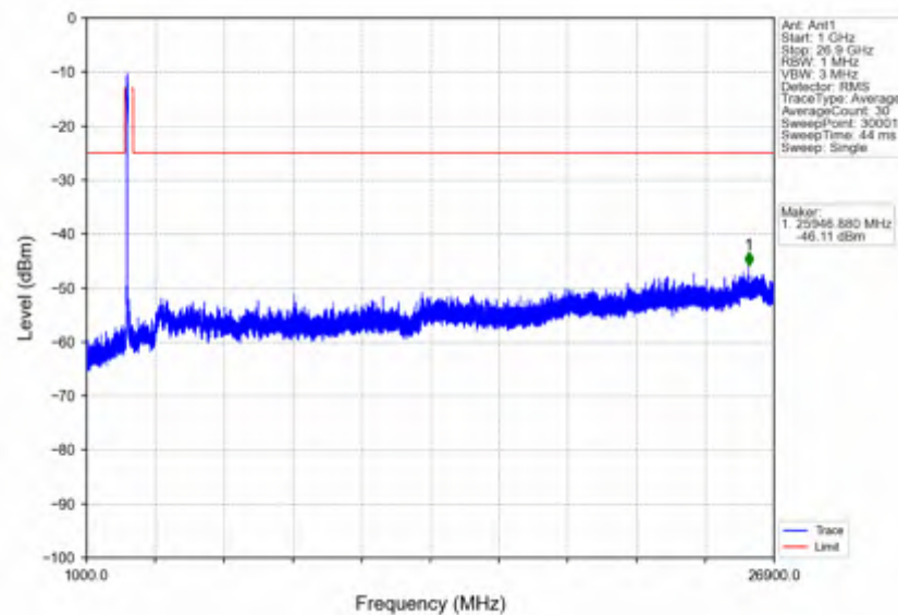
n41_30kHz_SISO_NTNV_60MHz_DFT-s-OFDM_PI/2_BPSK_2526MHz_Outer_Full
