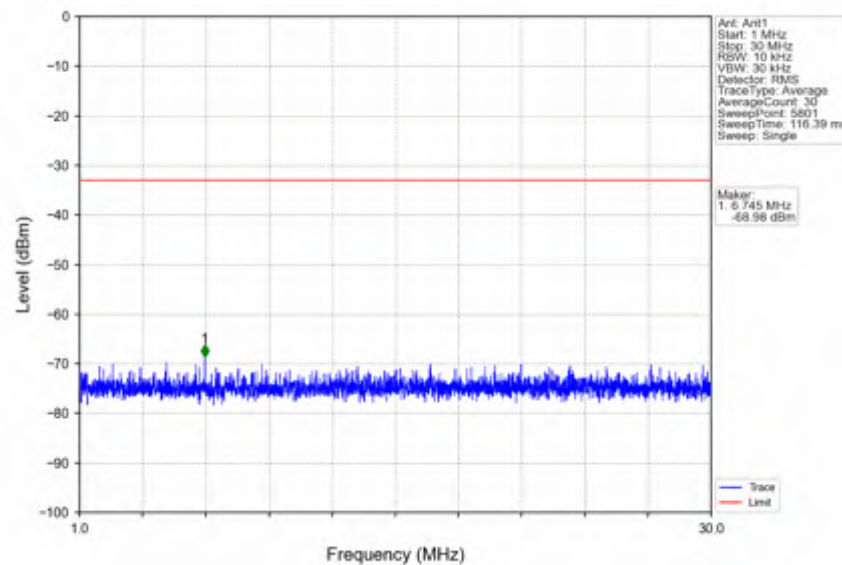
n41_30kHz_SISO_NTNV_90MHz_DFT-s-OFDM QPSK_2592.99MHz_Edge_1RB_Left
