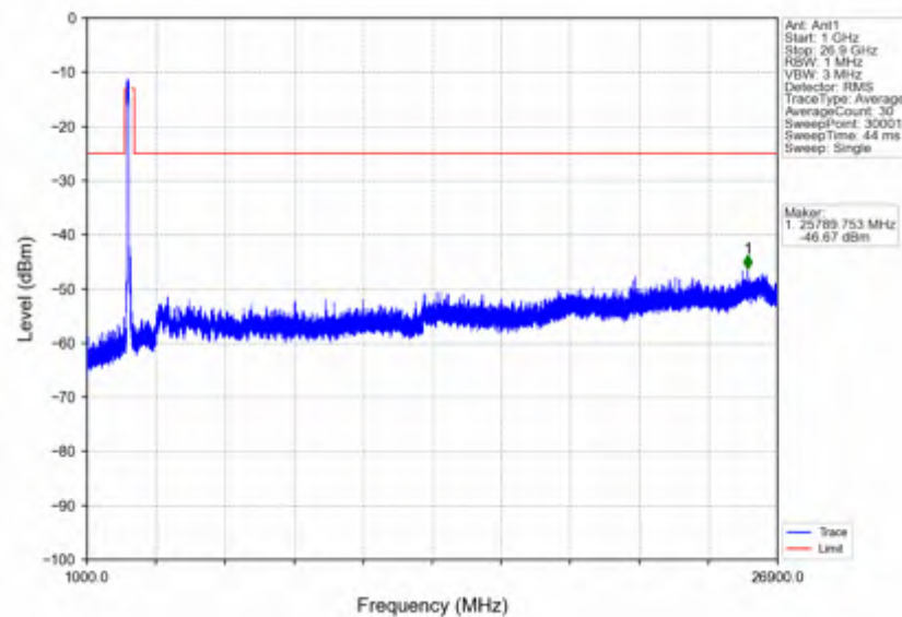
n41_30kHz_SISO_NTNV_80MHz_CP-OFDM QPSK_2536.02MHz_Outer_Full
