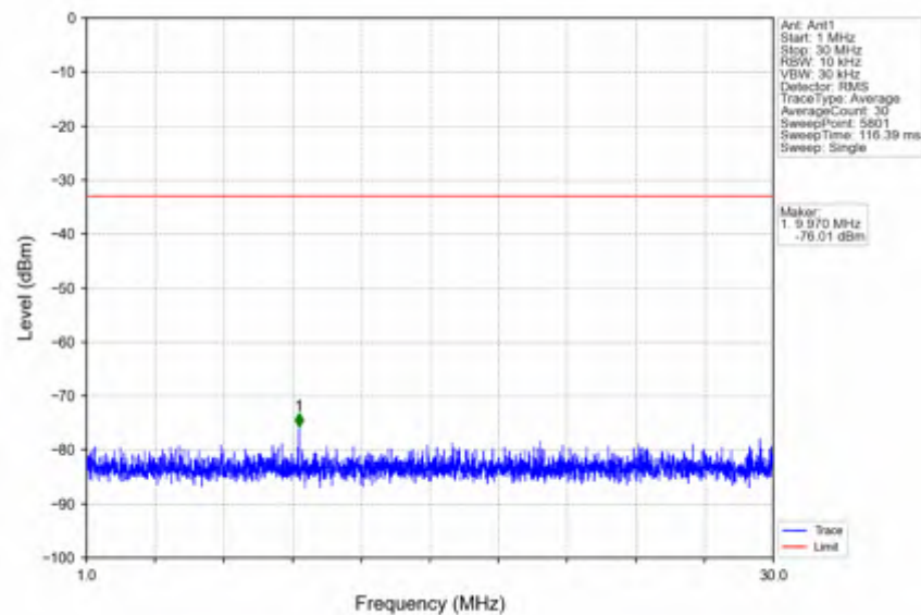
n41_30kHz_SISO_NTNV_80MHz_DFT-s-OFDM QPSK_2536.02MHz_Outer_Full
