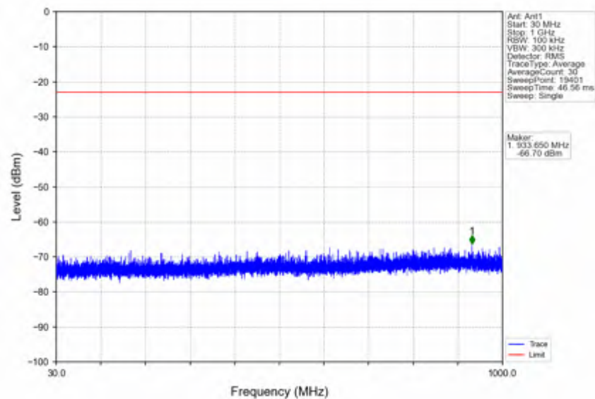
n41_30kHz_SISO_NTNV_60MHz_DFT-s-OFDM_PI/2_BPSK_2526MHz_Outer_Full
