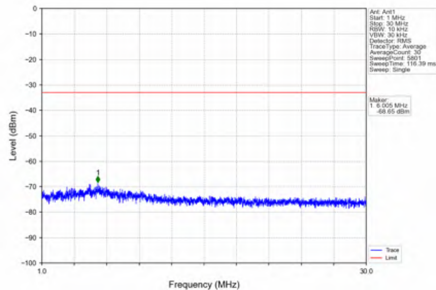
n41_30kHz_SISO_NTNV_90MHz_DFT-s-OFDM QPSK_2541MHz_Outer_Full
