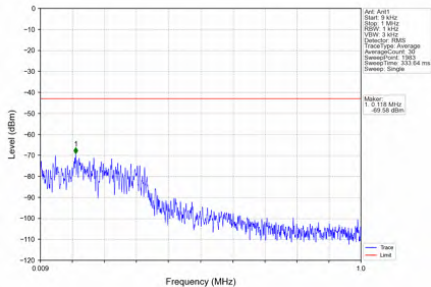
n41_30kHz_SISO_NTNV_50MHz_DFT-s-OFDM QPSK_2664.99MHz_Edge_1RB_Right
