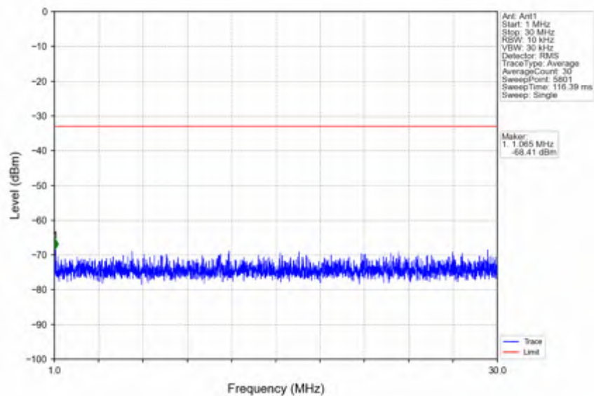
n41_30kHz_SISO_NTNV_50MHz_DFT-s-OFDM QPSK_2521.02MHz_Edge_1RB_Left
