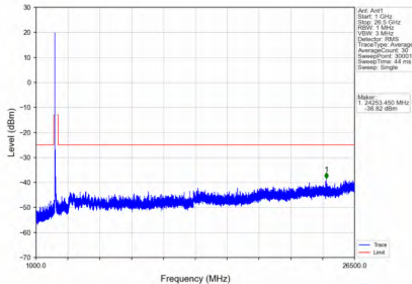
n41_30kHz_SISO_NTNV_80MHz_DFT-s-OFDM QPSK_2536.02MHz_Edge_1RB_Left
