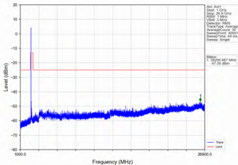
n41_30kHz_SISO_NTNV_80MHz_CP-OFDM QPSK_2592.99MHz_Edge_1RB_Left
