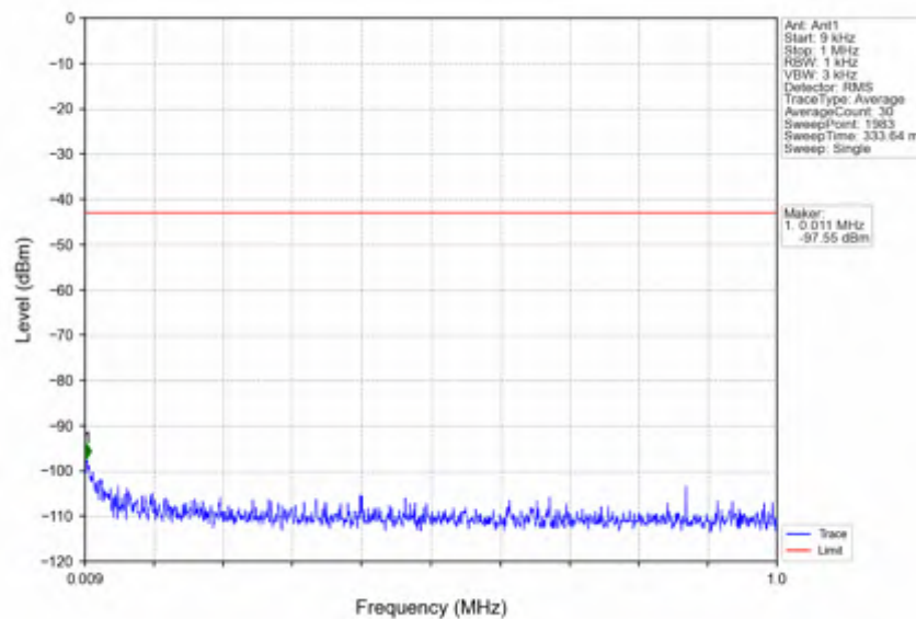
n41_30kHz_SISO_NTNV_50MHz_DFT-s-OFDM_QPSK_2664.99MHz_Outer_Full
