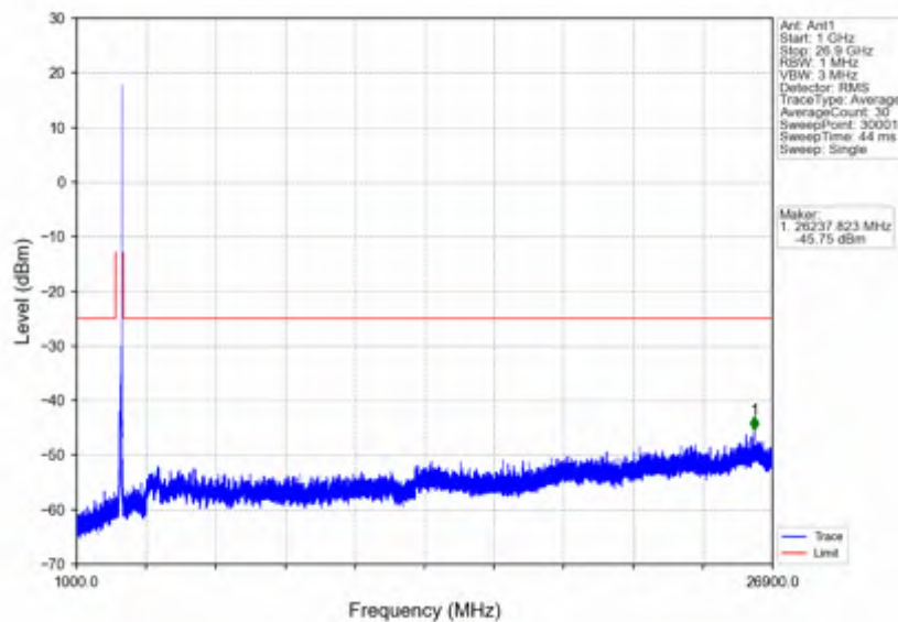
n41_30kHz_SISO_NTNV_50MHz_CP-OFDM QPSK_2664.99MHz_Outer_Full
