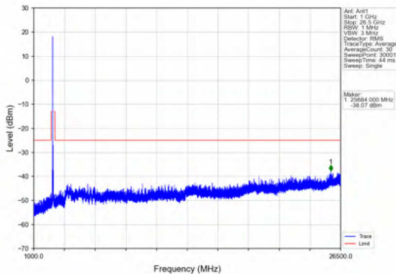
n41_30kHz_SISO_NTNV_60MHz_DFT-s-OFDM_QPSK_2659.98MHz_Edge_1RB_Right
