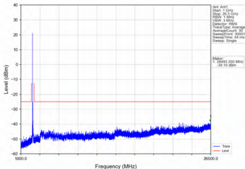
n41_30kHz_SISO_NTNV_80MHz_DFT-s-OFDM QPSK_2649.99MHz_Edge_1RB_Right
