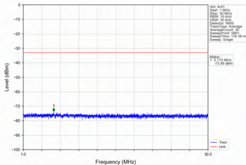
n41_30kHz_SISO_NTNV_60MHz_DFT-s-OFDM QPSK_2659.98MHz_Outer_Full
