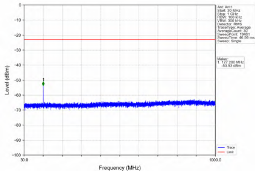
n41_30kHz_SISO_NTNV_80MHz_DFT-s-OFDM_QPSK_2649.99MHz_Inner_1RB_Right
