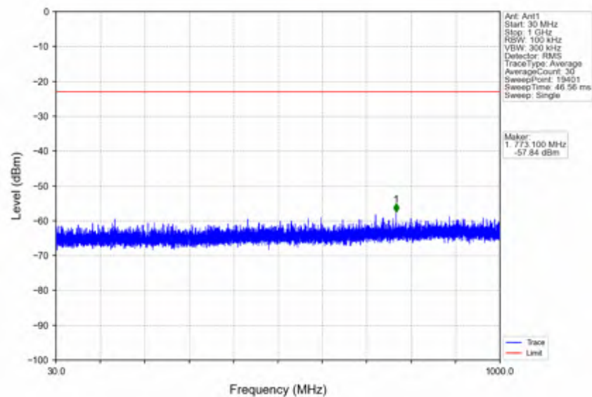
n41_30kHz_SISO_NTNV_80MHz_DFT-s-OFDM QPSK_2649.99MHz_Edge_1RB_Right
