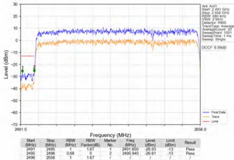
n41_30kHz_SISO_NTNV_60MHz_CP-OFDM QPSK_2526MHz_Outer_Full
