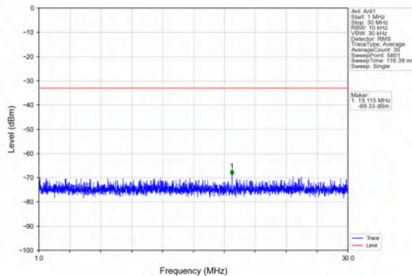
n41_30kHz_SISO_NTNV_60MHz_CP-OFDM QPSK_2659.98MHz_Edge_1RB_Right
