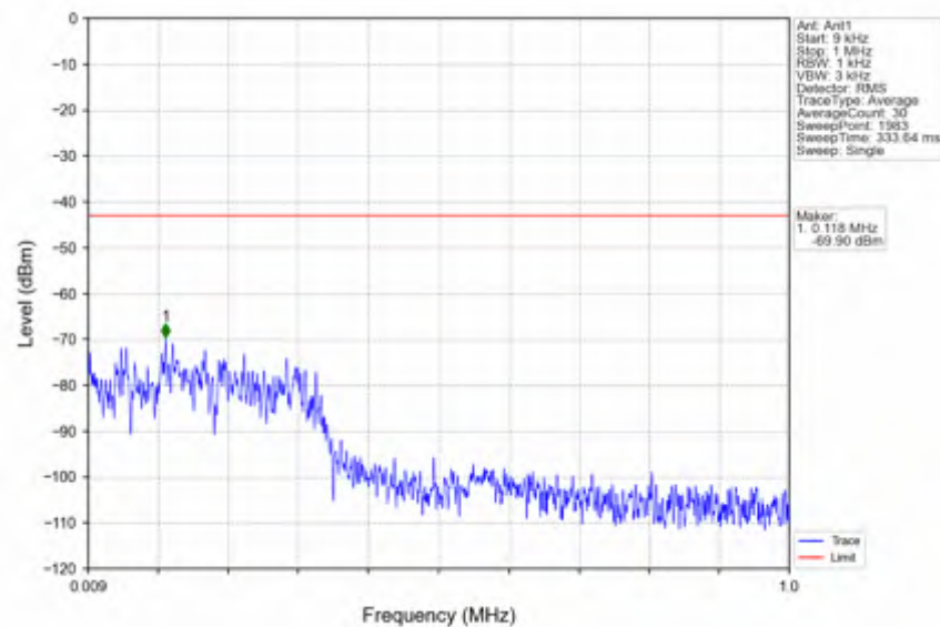
n41_30kHz_SISO_NTNV_80MHz_DFT-s-OFDM QPSK_2536.02MHz_Edge_1RB_Left
