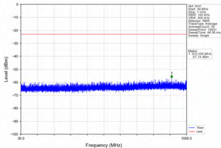
n41_30kHz_SISO_NTNV_50MHz_DFT-s-OFDM QPSK_2664.99MHz_Edge_1RB_Right
