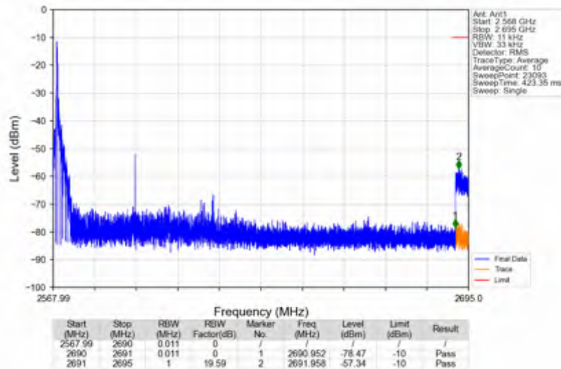
n41_30kHz_SISO_NTNV_50MHz_CP-OFDM QPSK_2592.99MHz_Edge_1RB_Left
