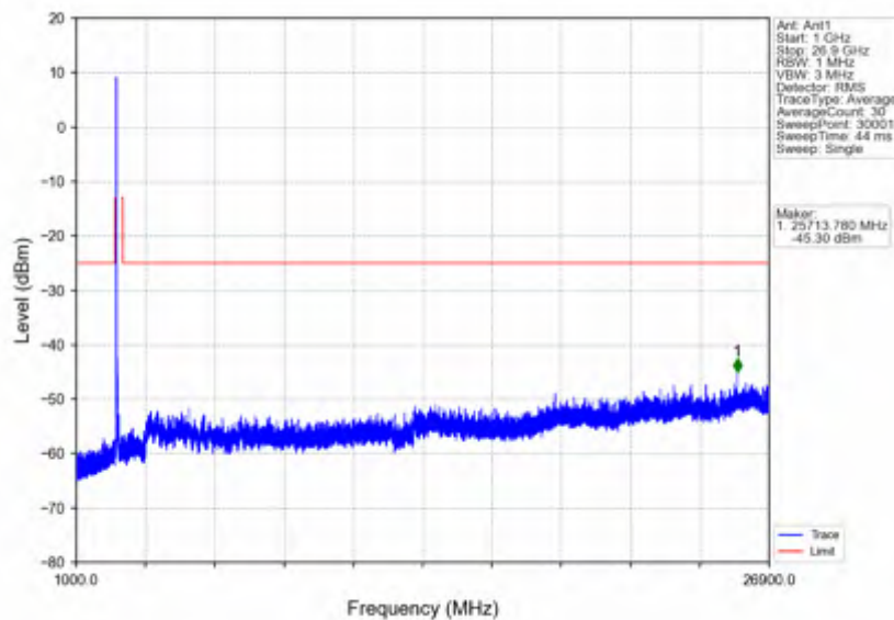
n41_30kHz_SISO_NTNV_50MHz_CP-OFDM QPSK_2592.99MHz_Edge_1RB_Left
