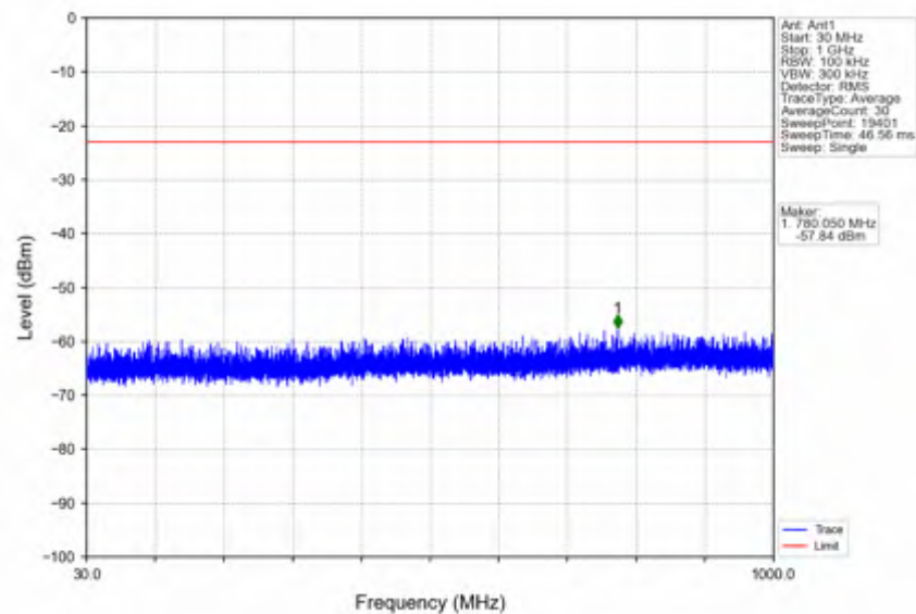
n41_30kHz_SISO_NTNV_50MHz_CP-OFDM_QPSK_2592.99MHz_Edge_1RB_Left
