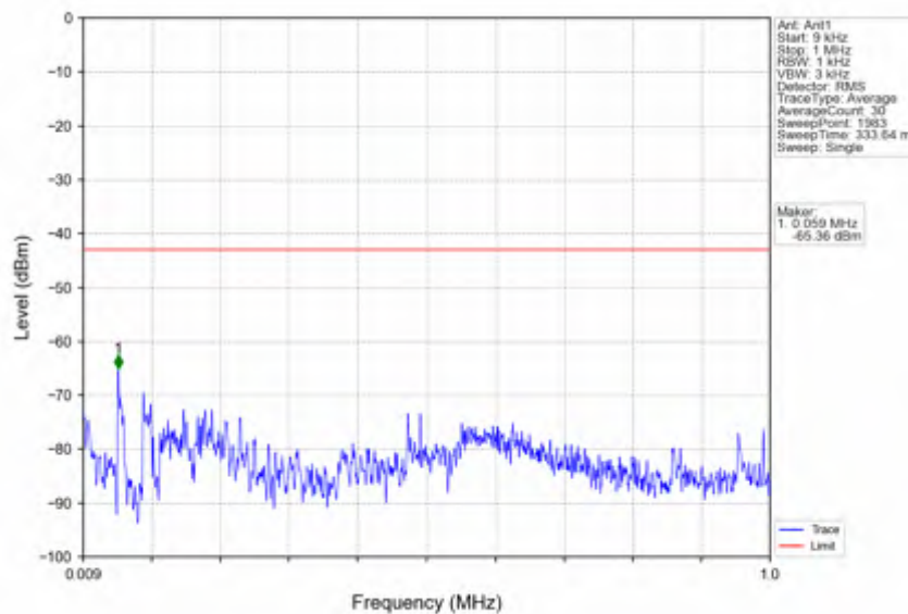
n41_30kHz_SISO_NTNV_80MHz_DFT-s-OFDM_QPSK_2649.99MHz_Outer_Full
