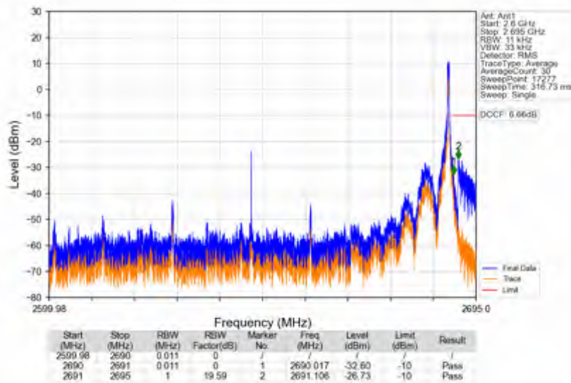
n41_30kHz_SISO_NTNV_90MHz_DFT-s-OFDM_QPSK_2644.98MHz_Edge_1RB_Right
