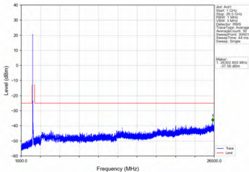
n41_30kHz_SISO_NTNV_80MHz_CP-OFDM_QPSK_2536.02MHz_Outer_Full
