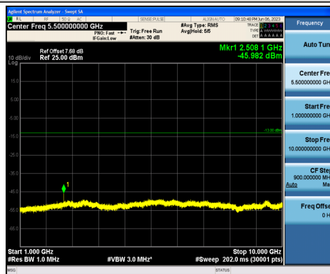
Band5-1.4MHz-QPSK-20525-1-0-Low-1000-10000--45.98-PASS
