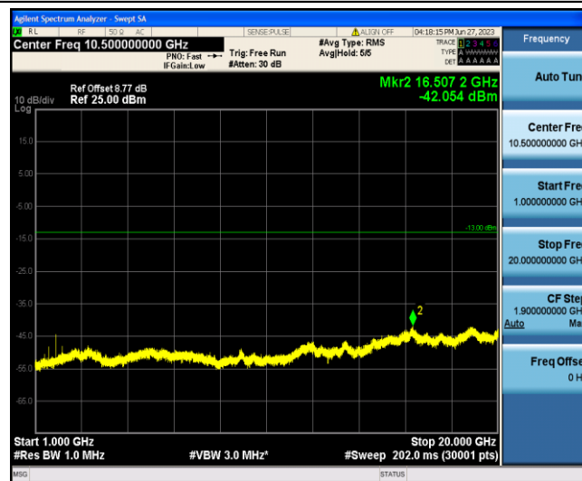
Band4-10MHz-QPSK-20000-1-0-Low-1000-20000--42.05-PASS
