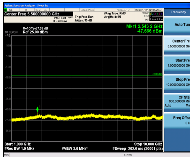
Band5-1.4MHz-16QAM-20643-1-0-Low-1000-10000--47.67-PASS
