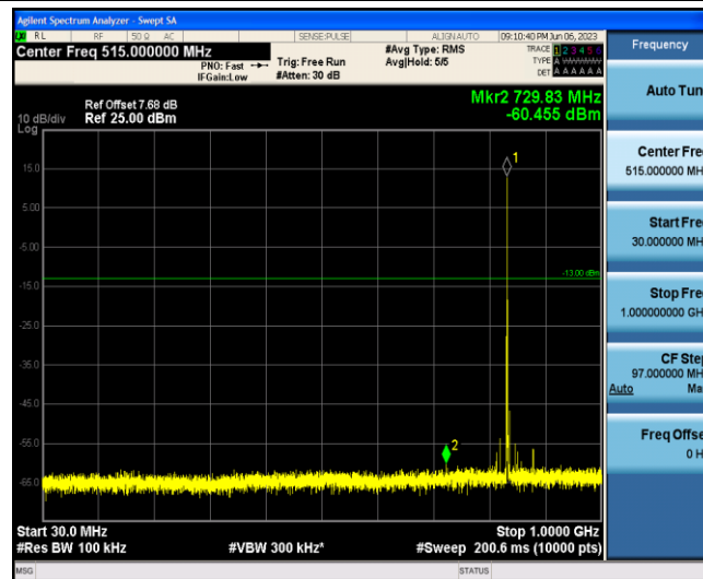
Band5-1.4MHz-QPSK-20525-1-0-Low-30-1000--60.46-PASS
