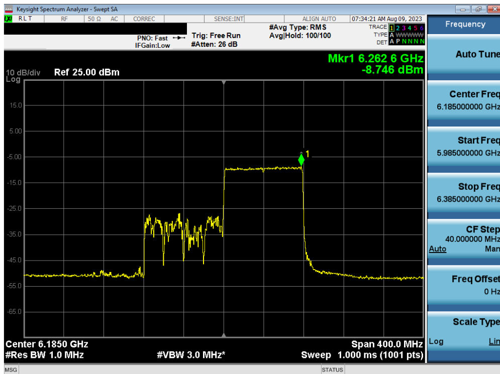
Plot 7-116. Power Spectral Density Plot MIMO ANT2 (160MHz BW 802.11ax (996 Tone) (UNII Band 5) – Ch. 47)
