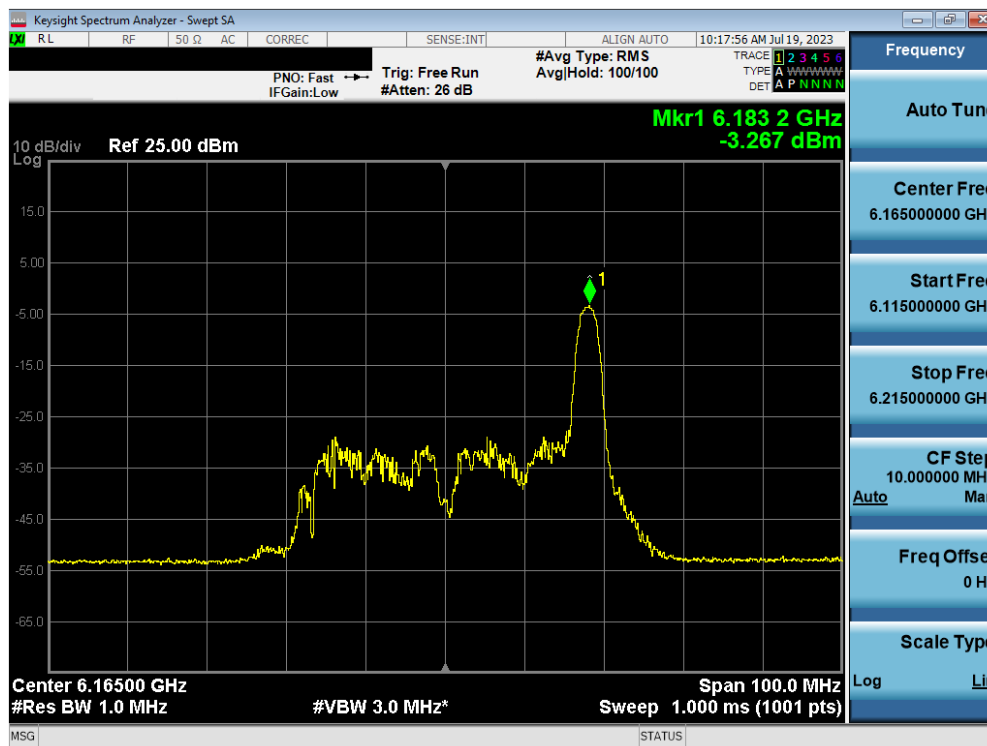
Plot 7-66. Power Spectral Density Plot MIMO ANT1 (40MHz BW 802.11ax (26 Tones) (UNII Band 5) – Ch. 43)
