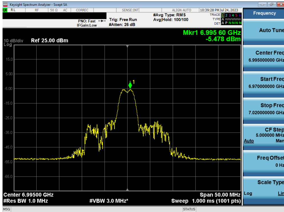
Plot 7-77. Power Spectral Density Plot MIMO ANT1 (20MHz BW 802.11ax (26 Tones) (UNII Band 8) – Ch. 209)
