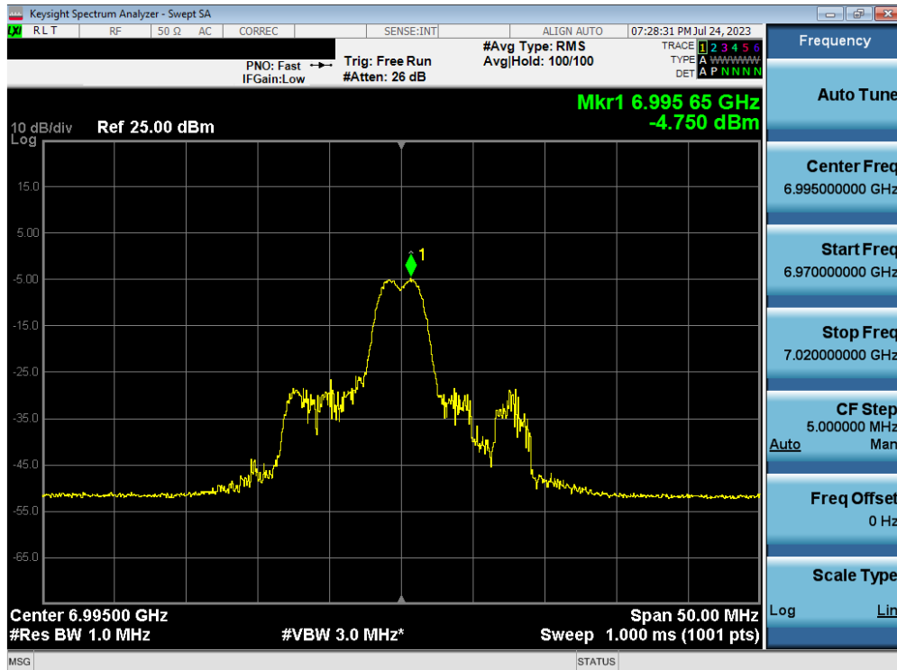
Plot 7-109. Power Spectral Density Plot MIMO ANT2 (20MHz BW 802.11ax (26 Tones) (UNII Band 8) – Ch. 209)
