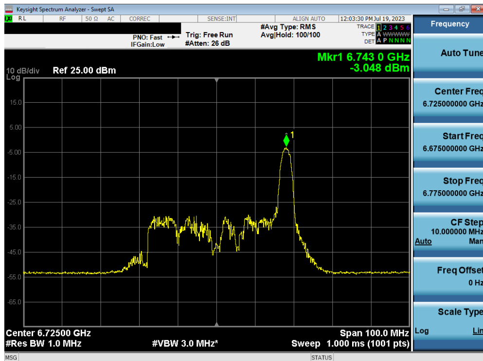
Plot 7-74. Power Spectral Density Plot MIMO ANT1 (40MHz BW 802.11ax (26 Tones) (UNII Band 7) – Ch. 155)
