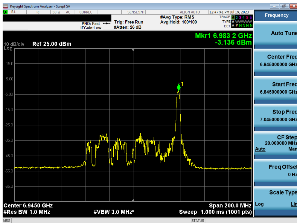
Plot 7-79. Power Spectral Density Plot MIMO ANT1 (80MHz BW 802.11ax (26 Tones) (UNII Band 8) – Ch. 199)
