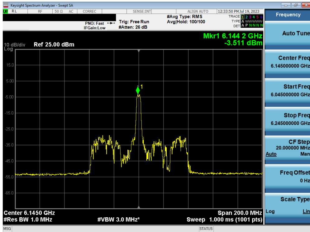
Plot 7-67. Power Spectral Density Plot MIMO ANT1 (80MHz BW 802.11ax (26 Tones) (UNII Band 5) – Ch. 39)
