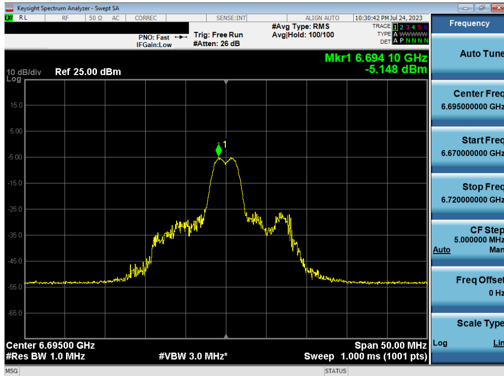
Plot 7-73. Power Spectral Density Plot MIMO ANT1 (20MHz BW 802.11ax (26 Tones) (UNII Band 7) – Ch. 149)
