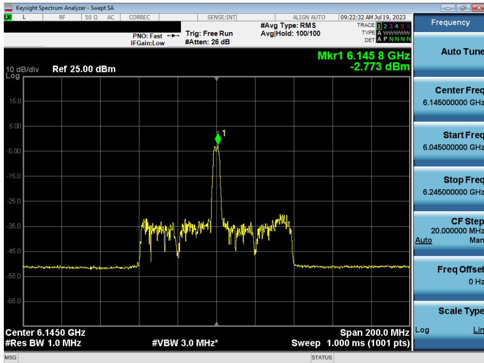
Plot 7-99. Power Spectral Density Plot MIMO ANT2 (80MHz BW 802.11ax (26 Tones) (UNII Band 5) – Ch. 39)
