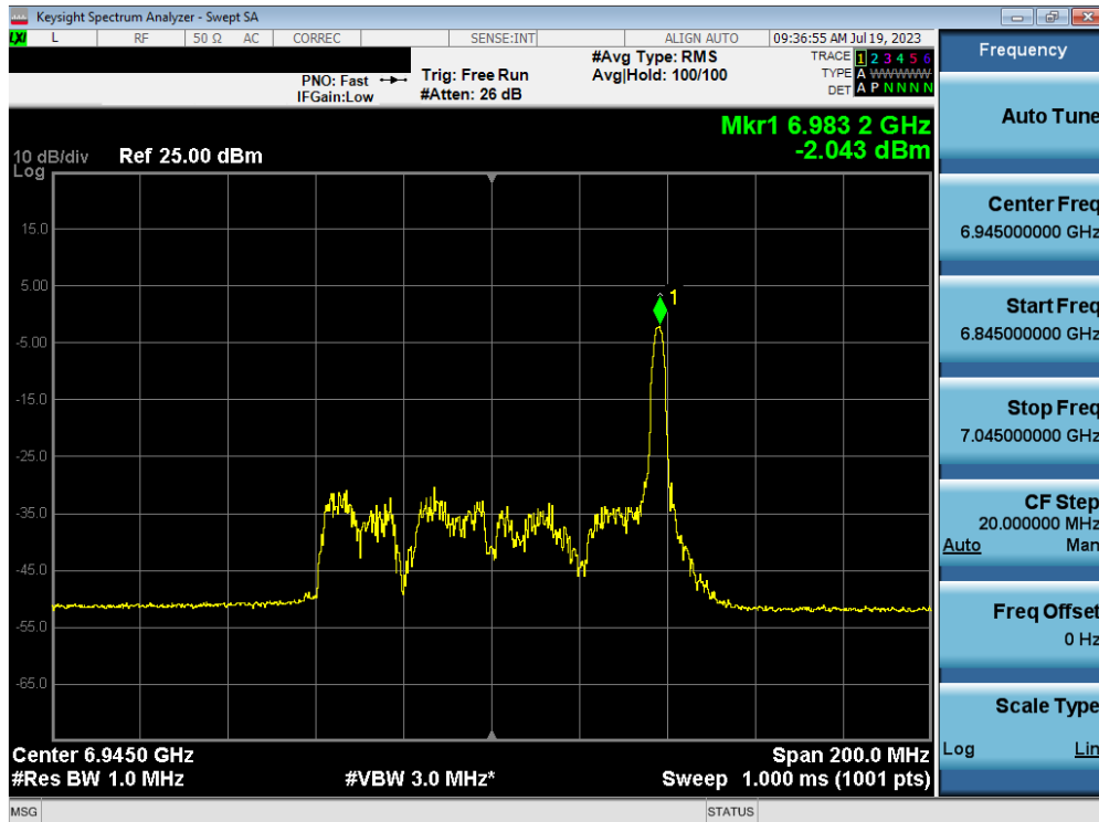
Plot 7-111. Power Spectral Density Plot MIMO ANT2 (80MHz BW 802.11ax (26 Tones) (UNII Band 8) – Ch. 199)
