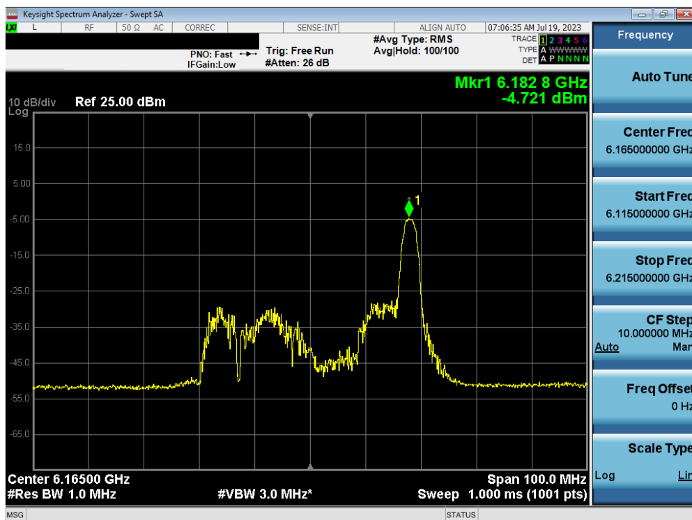
Plot 7-98. Power Spectral Density Plot MIMO ANT2 (40MHz BW 802.11ax (26 Tones) (UNII Band 5) – Ch. 43)
