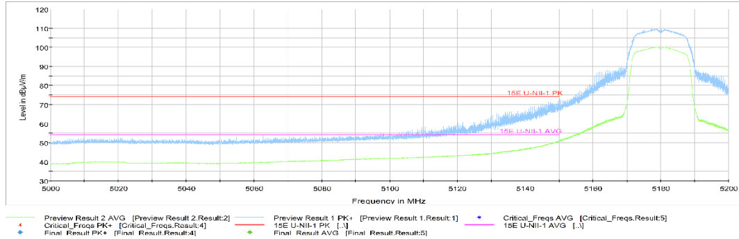
Fig.34 Band Edges (802.11a Ch36, 5180MHz)
