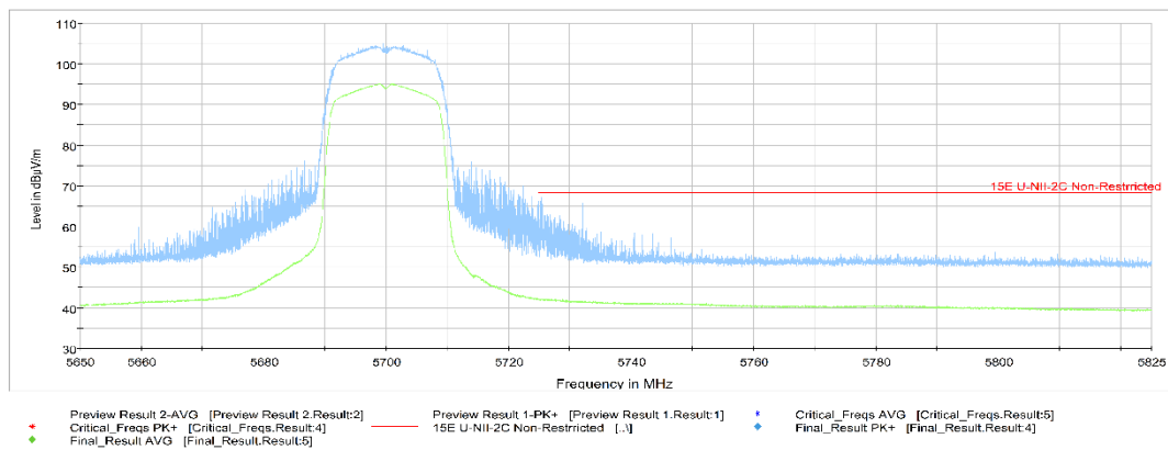
Fig.41 Band Edges (802.11n-HT20 Ch140, 5700MHz)
