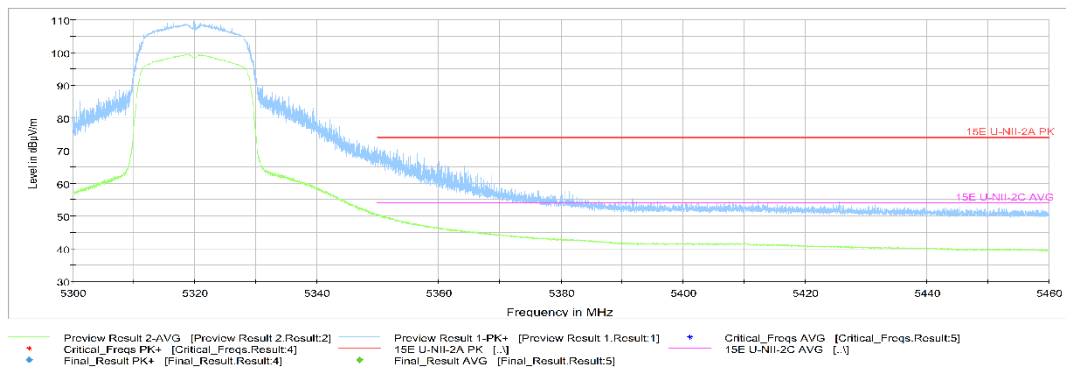
Fig.39 Band Edges (802.11n-HT20 Ch64, 5320MHz)
