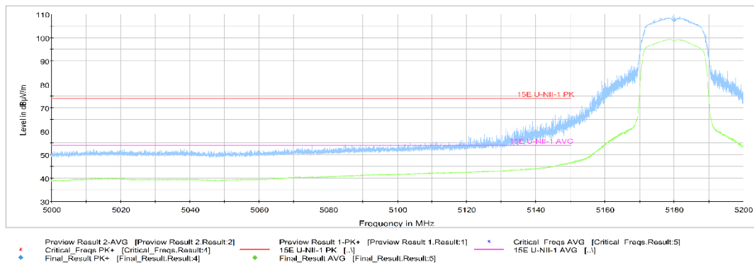
Fig.46 Band Edges (802.11ac-HT20 Ch36, 5180MHz)
