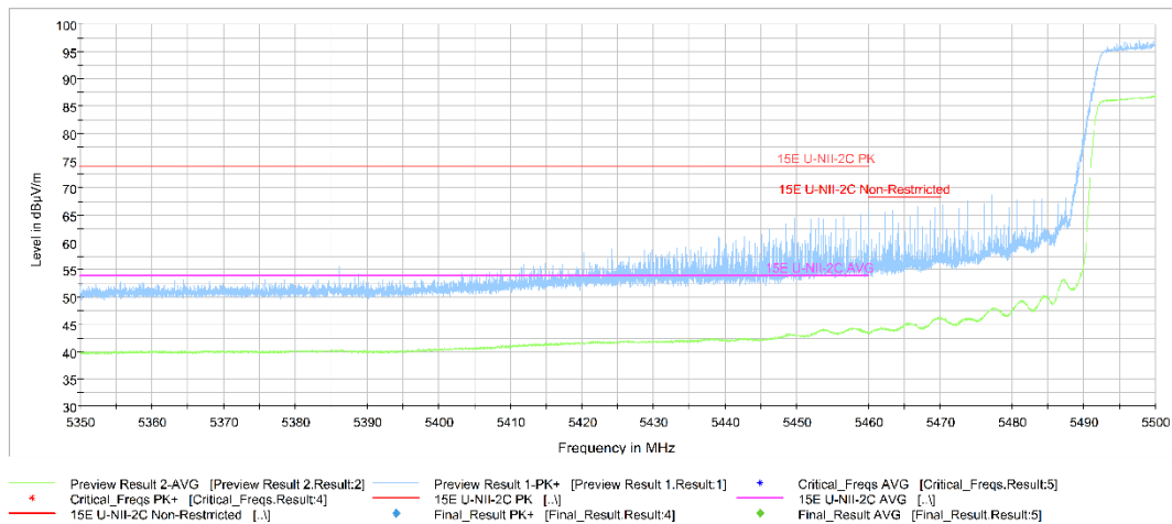
Fig.56 Band Edges (802.11ac-HT80 Ch106, 5530MHz)
