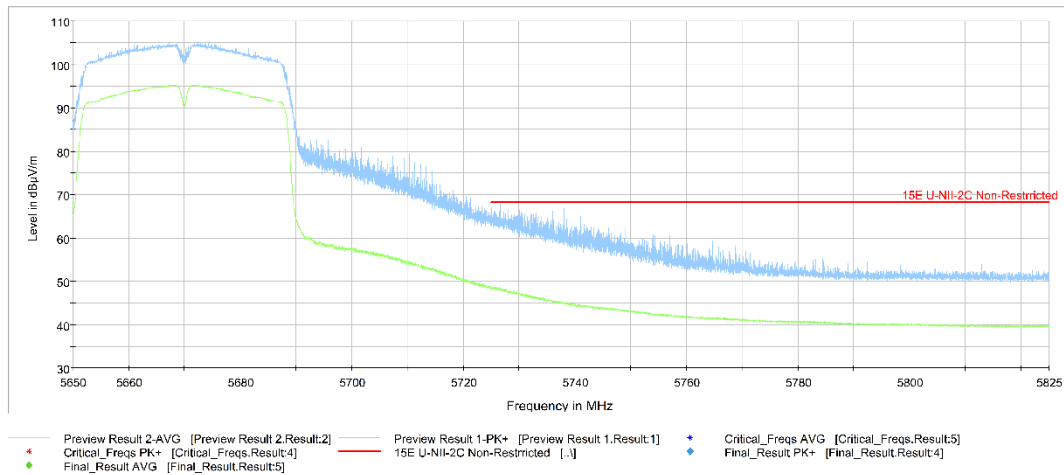
Fig.53 Band Edges (802.11ac-HT40 Ch134, 5670MHz)
