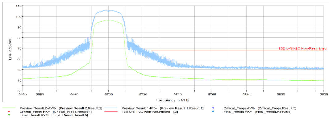
Fig.37 Band Edges (802.11a Ch140, 5700MHz)
