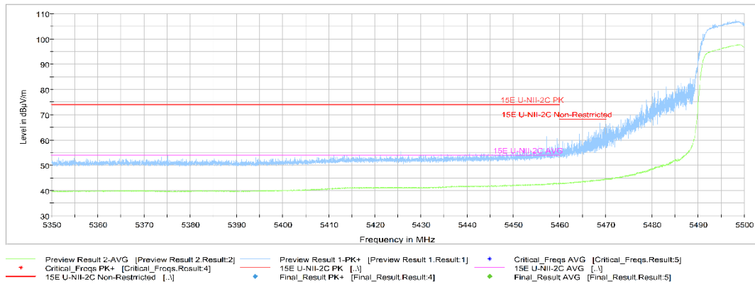
Fig.40 Band Edges (802.11n-HT20 Ch100, 5500MHz)
