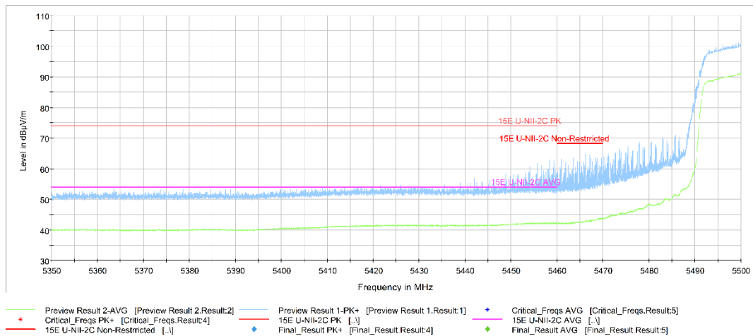
Fig.44 Band Edges (802.11n-HT40 Ch102, 5510MHz)
