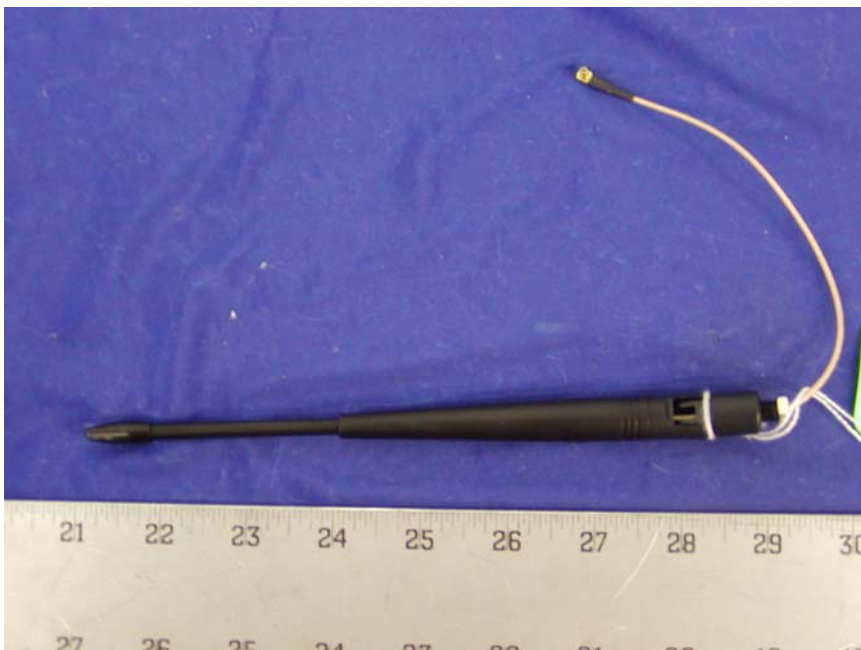
S467FL-L-RMM-915S Antenna – Top View
