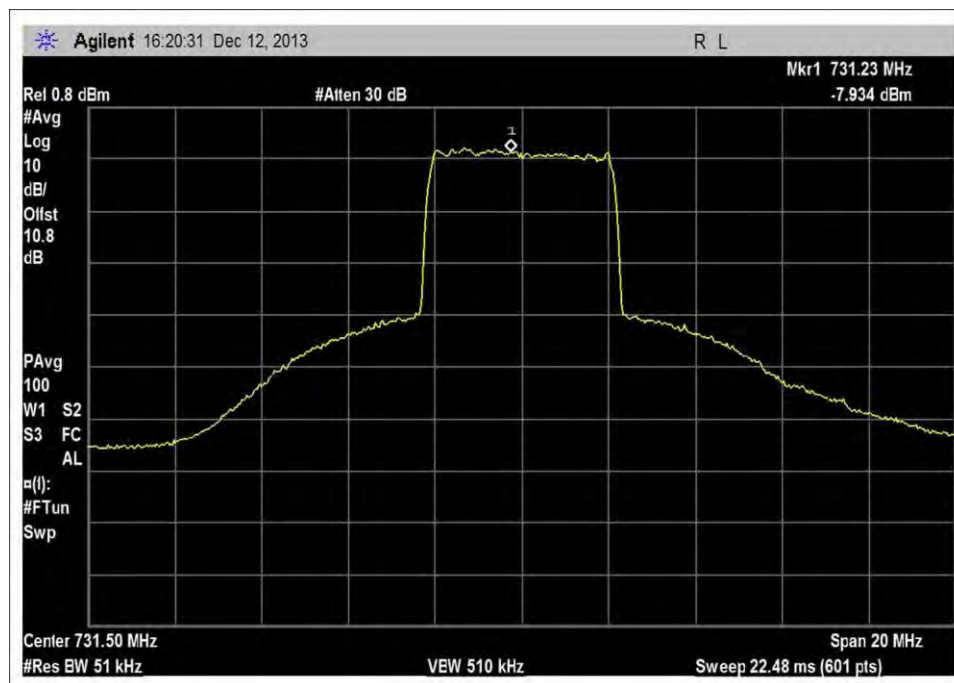
DL_716-746MHz_Output
