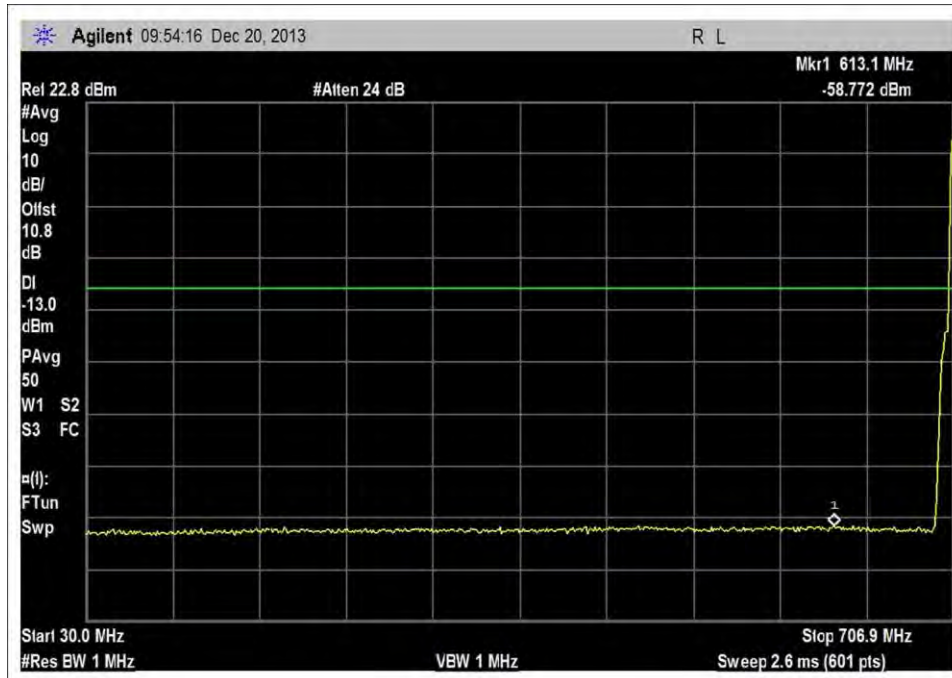
UL_698-716MHz_M_5WCDMATM1_2
