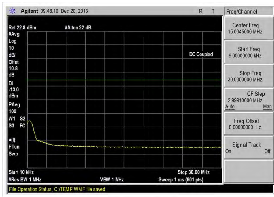
UL_698-716MHz_M_5WCDMATM1_1
