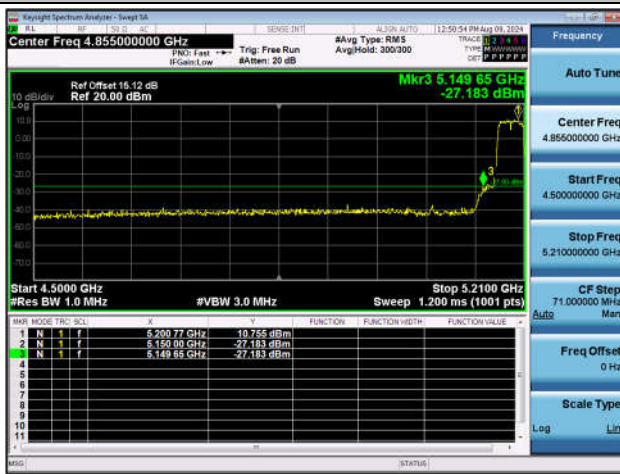
11AC40SISO-Ant1-5190-PASS
