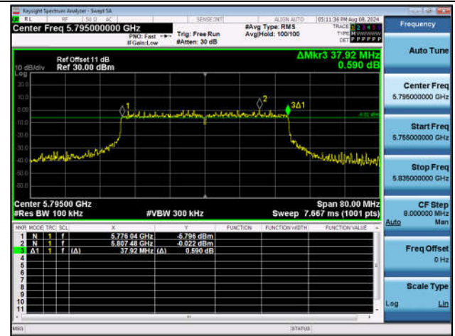
11AX40SISO-Ant1-5795-PASS
