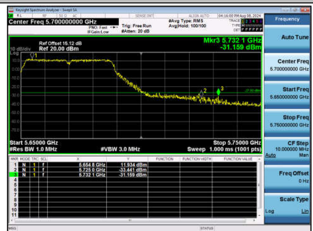
11N40SISO-Ant1-5670-PASS
