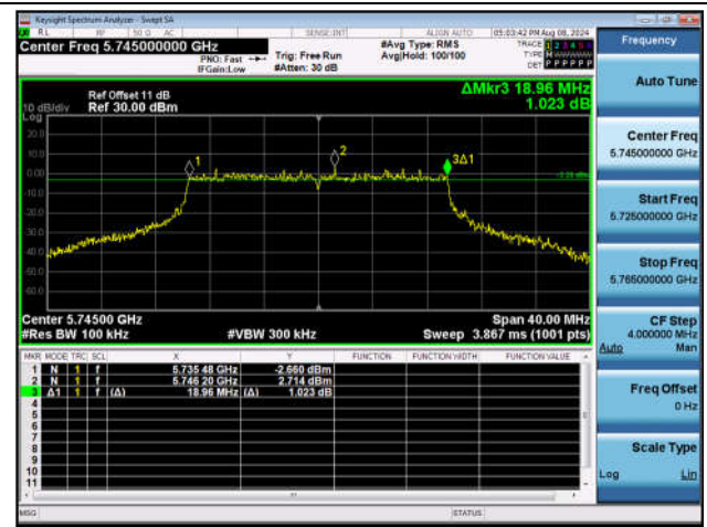
11AX20SISO-Ant1-5745-PASS
