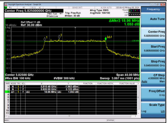
11AX20SISO-Ant1-5825-PASS
