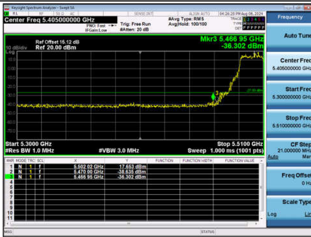
11AX20SISO-Ant1-5500-PASS
