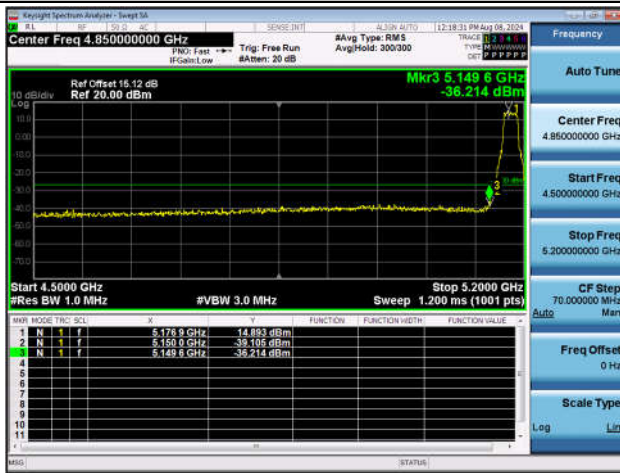
11AX20SISO-Ant1-5180-PASS
