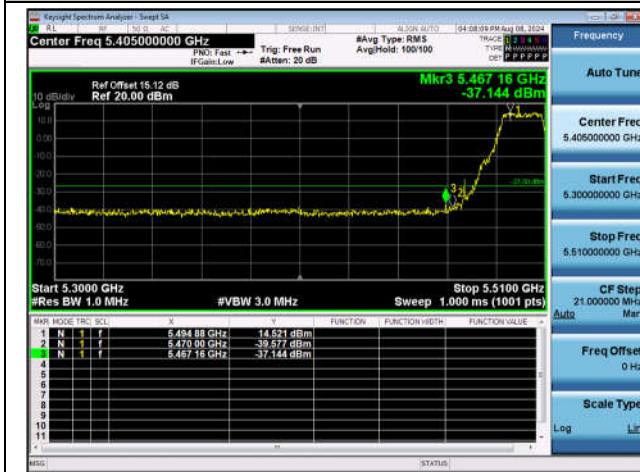
11N20SISO-Ant1-5500-PASS
