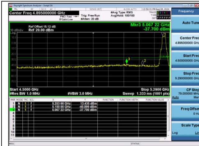
11A-Ant1-5260-PASS
