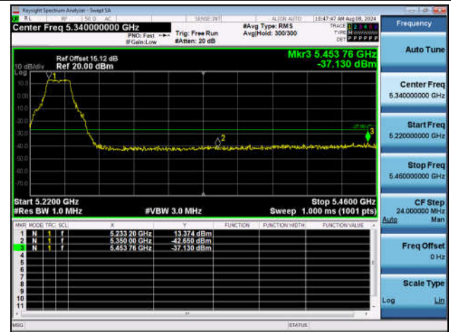
11A-Ant1-5240-PASS
