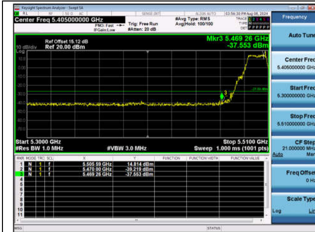
11A-Ant1-5500-PASS
