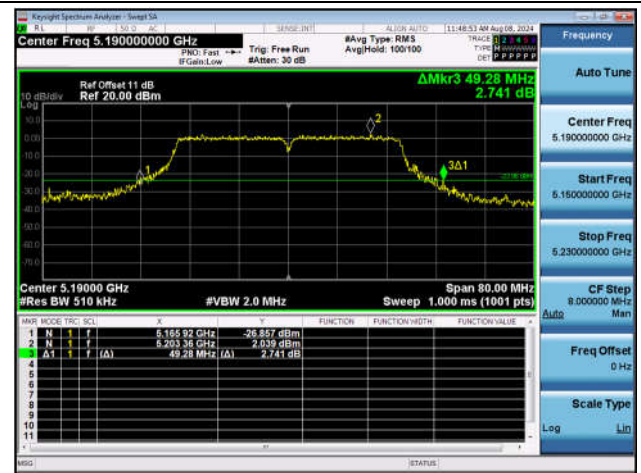
11N40SISO-Ant1-5190-26dB EBW
