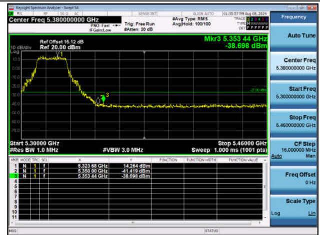
11AX20SISO-Ant1-5320-PASS
