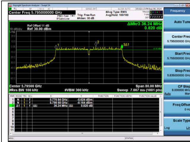
11AC40SISO-Ant1-5795-PASS
