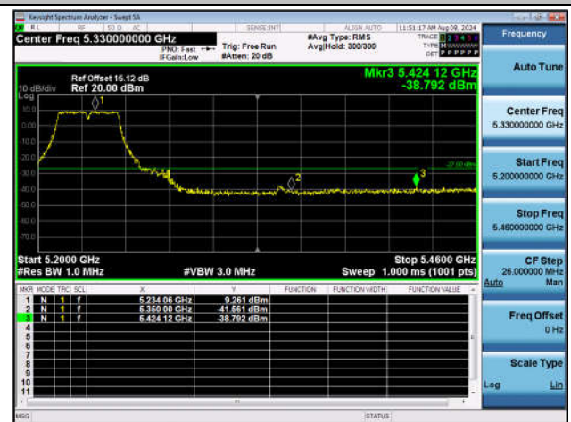
11N40SISO-Ant1-5230-PASS
