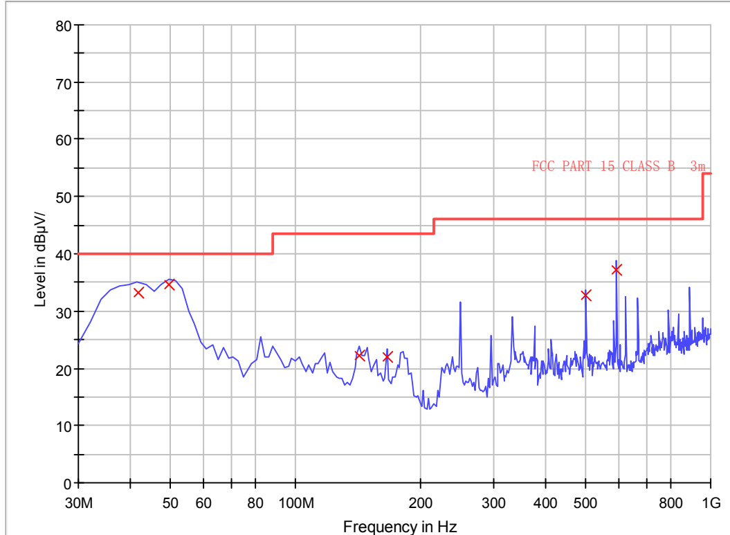
EMI Sweep-3M(30-1G)
