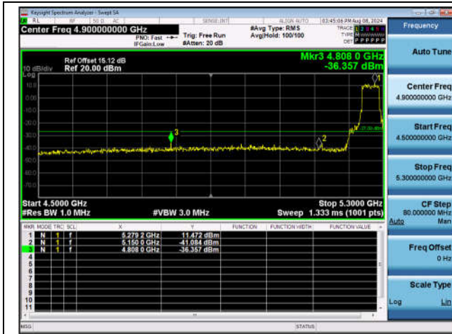
11AX40SISO-Ant1-5270-PASS
