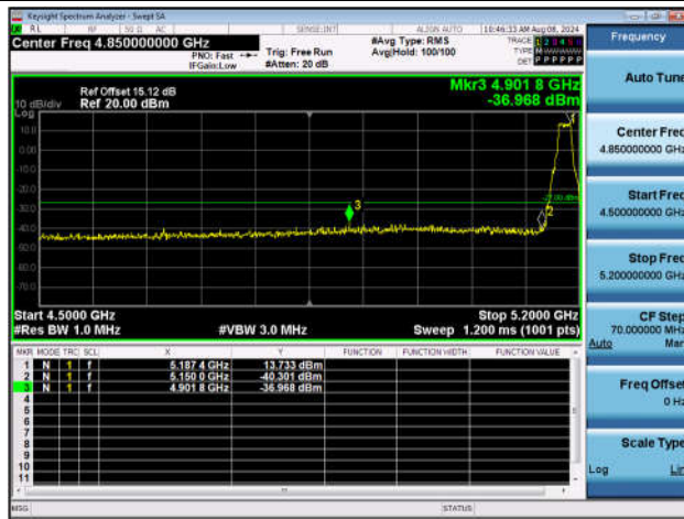
11A-Ant1-5180-PASS
