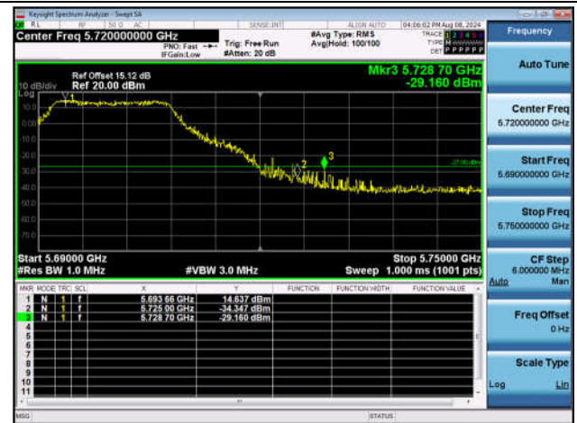
11A-Ant1-5700-PASS
