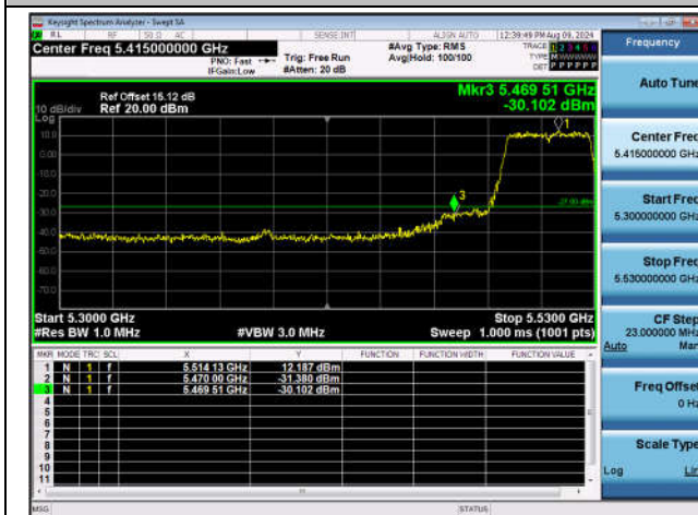
11N40SISO-Ant1-5510-PASS
