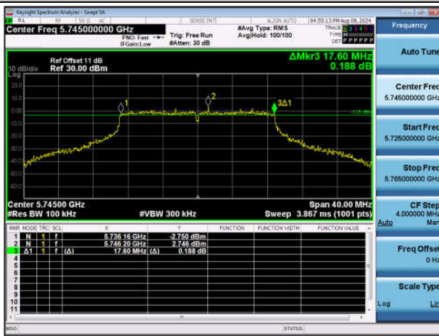
11AC20SISO-Ant1-5745-PASS
