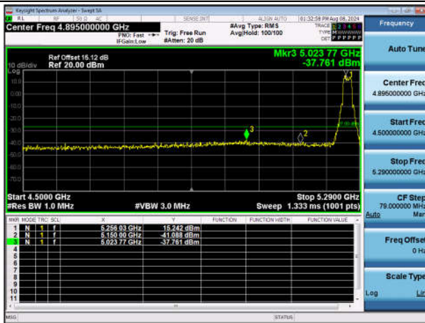
11AX20SISO-Ant1-5260-PASS
