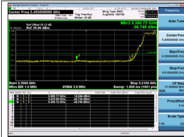
11AC20SISO-Ant1-5500-PASS
