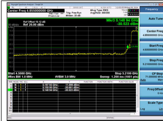
11AX40SISO-Ant1-5190-PASS
