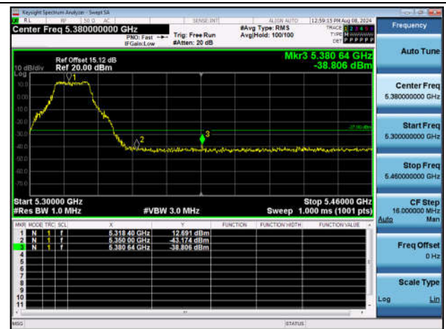
11A-Ant1-5320-PASS
