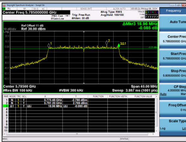
11AX20SISO-Ant1-5785-PASS
