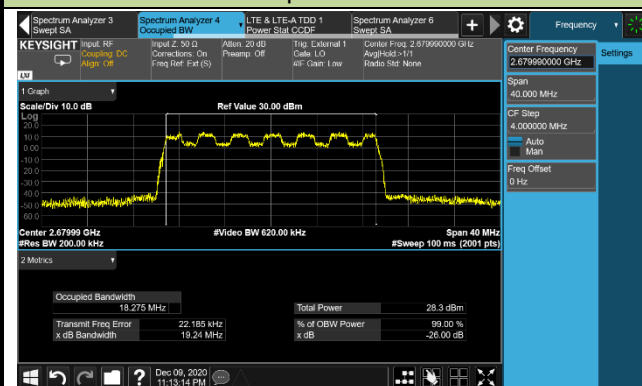
Emission Bandwidth - 16QAM
