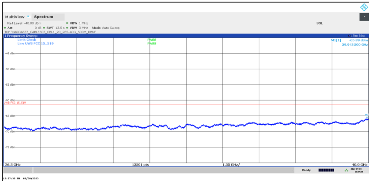
Plot 36: 26.5 GHz to 40.0 GHz, UWB test mode
