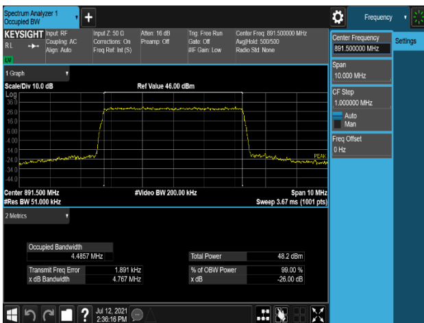
Plot 7-11. Occupied Bandwidth Plot (LTE_B5_5M_1C_64QAM - High Channel, Port 0)
