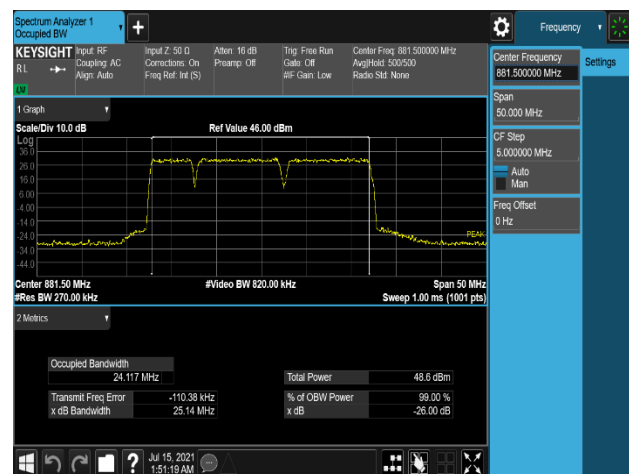
Plot 7-52. Occupied Bandwidth Plot (LTE_B5_5M+10M+10M_3C_256QAM - Low Channel, Port 2)
