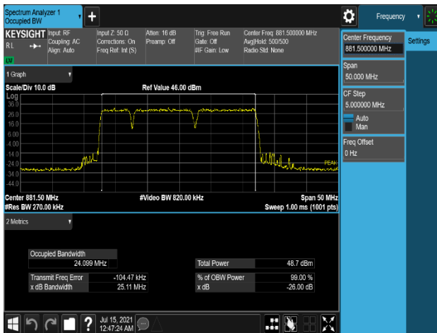
Plot 7-49. Occupied Bandwidth Plot (LTE_B5_5M+10M+10M_3C_QPSK - Low Channel, Port 1)
