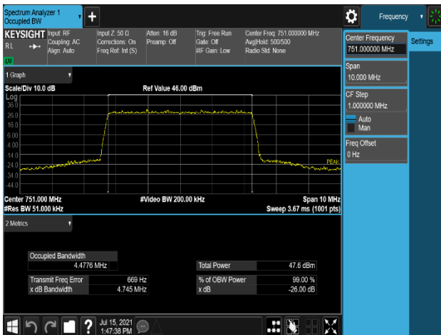
Plot 7-57. Occupied Bandwidth Plot (LTE_B13_5M_1C_QPSK - Mid Channel, Port 0)
