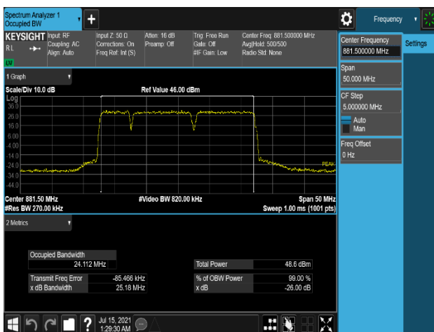
Plot 7-51. Occupied Bandwidth Plot (LTE_B5_5M+10M+10M_3C_64QAM - Low Channel, Port 0)
