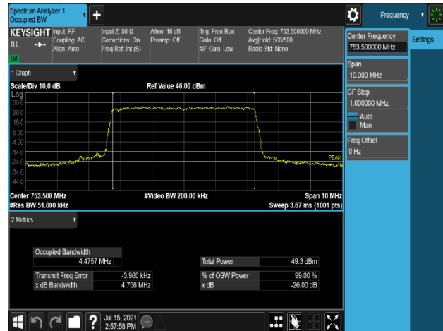
Plot 7-62. Occupied Bandwidth Plot (LTE_B13_5M_1C_16QAM - High Channel, Port 1)
