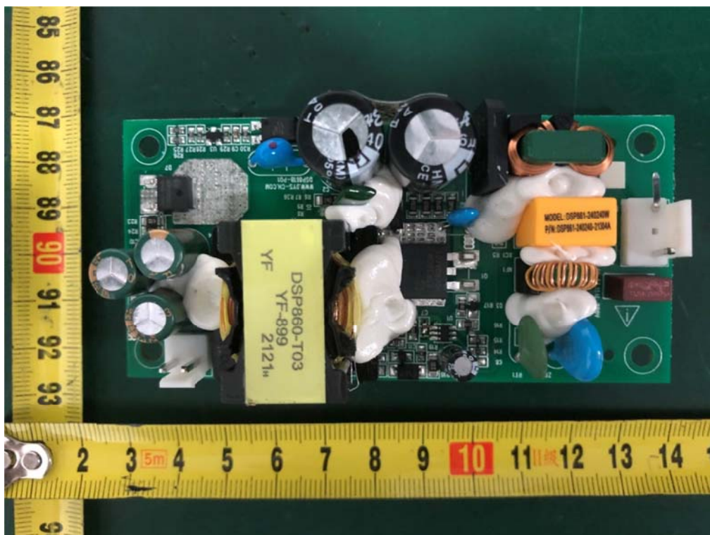
Internal Photos M/N: M215a-J6 Subwoofer
