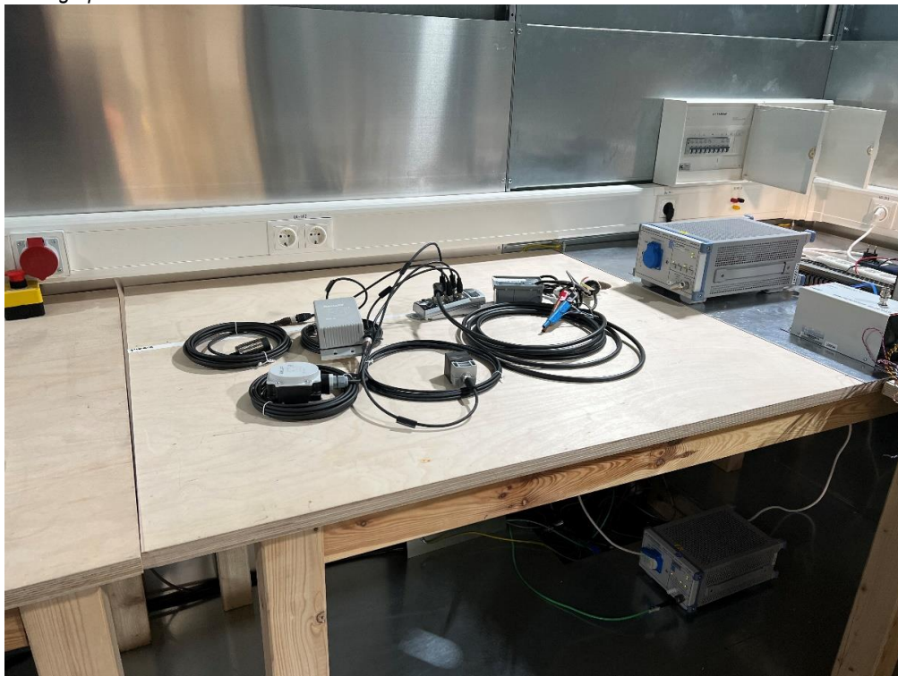
Photograph 8: EUT A + AE 4 + AE 5 + AE 7 + AE 8. Close view.
