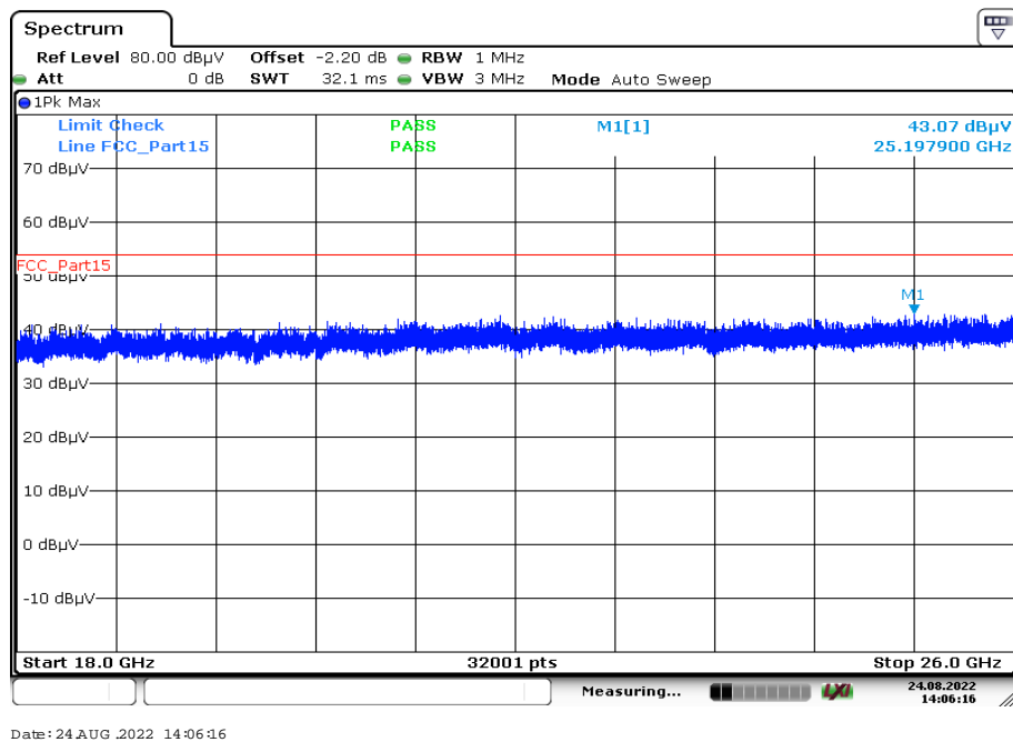
Plot 4: 18 GHz to 26 GHz, TX mode, vertical & horizontal polarization, valid for all channels and all antennas
