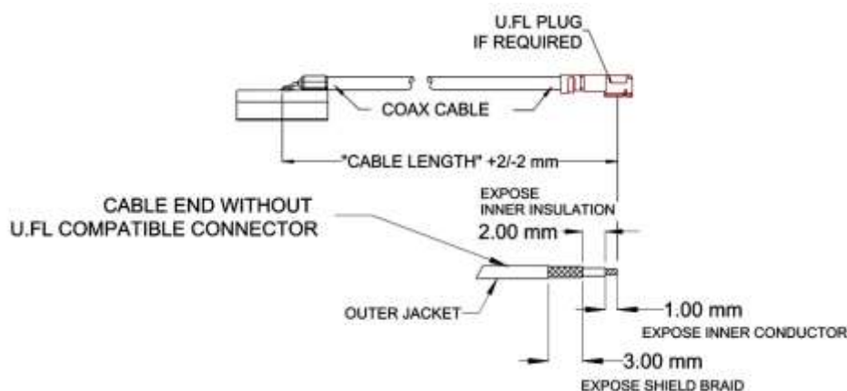
Figure 10: N2420DG3 with connector or stripped
