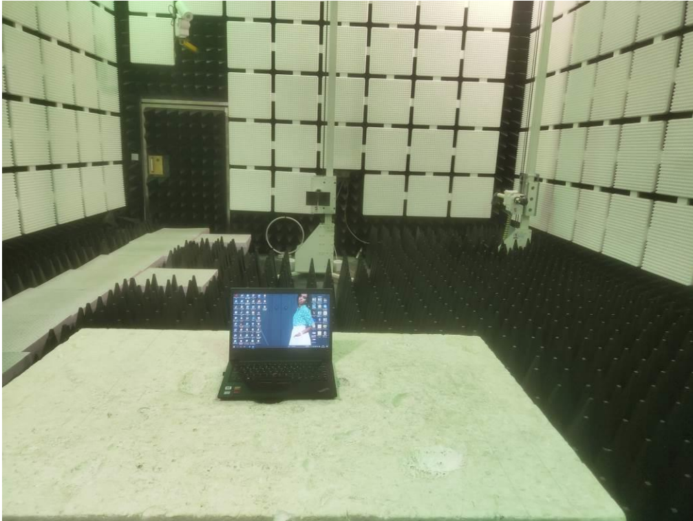
Photo of Radiated emission Measurement (1000-6000MHz)
