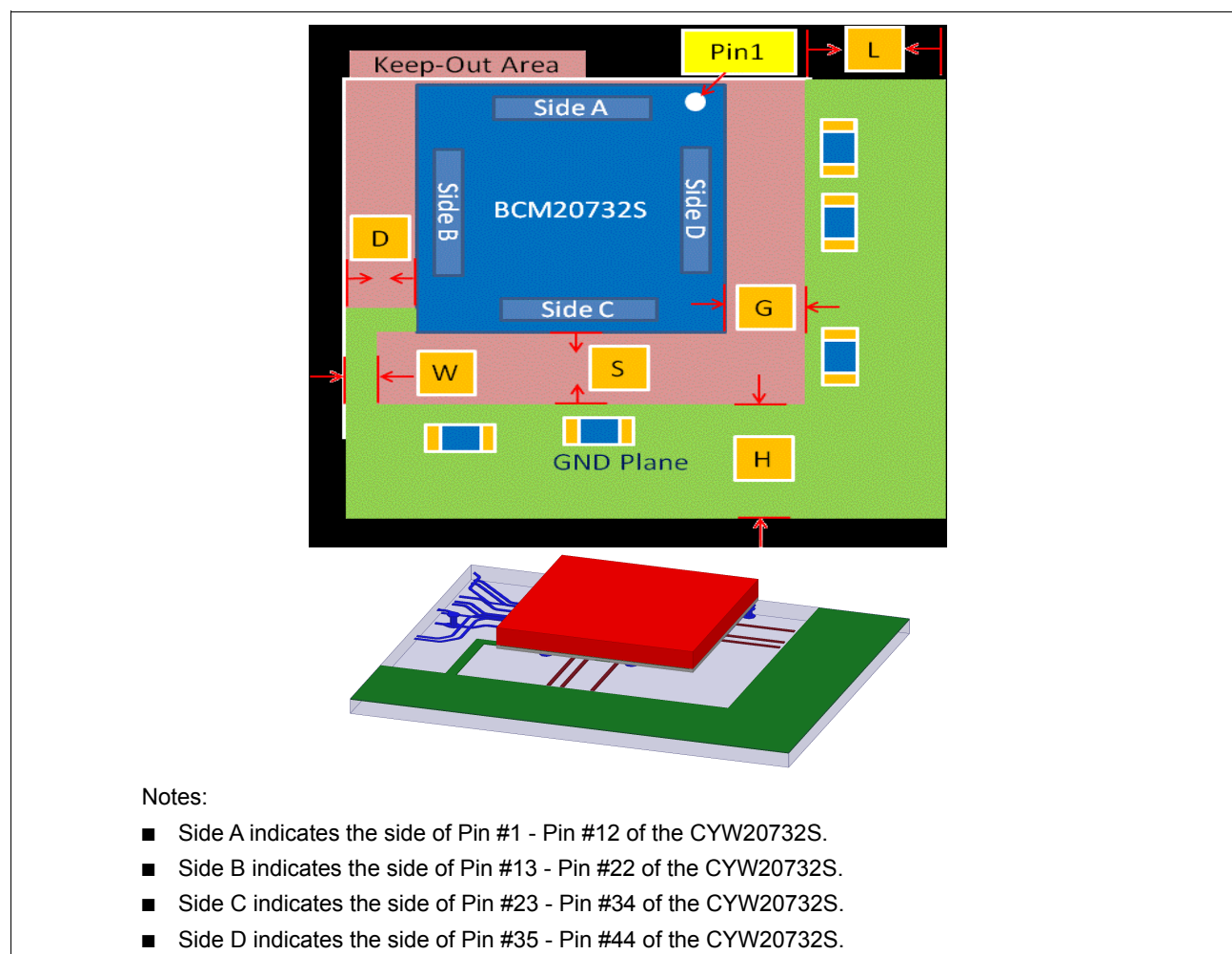
Figure 1-11. PCB Layout Example, Configuration B
