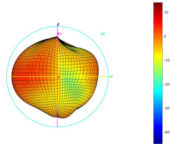
Total_3D_E2_5.15GHz
