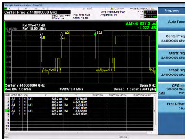
GFSK(BLE 1Mbps)
