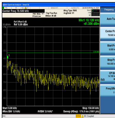
Band5_5MHz_16QAM_20625_1RB#0_0.009~0.15_0.009~0.15
