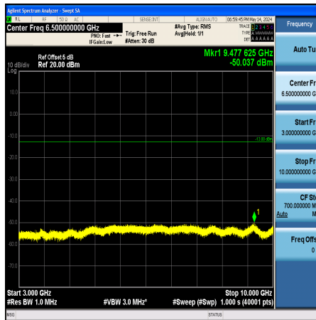
Band5_5MHz_QPSK_20625_1RB#0_3000~10000_3000~10000
