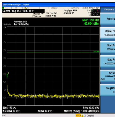
Band5_5MHz_16QAM_20625_1RB#0_0.15~30_0.15~30
