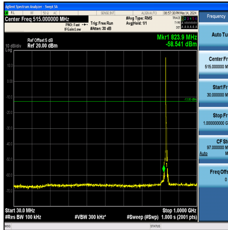
Band5_5MHz_QPSK_20525_1RB#0_30~1000_30~1000
