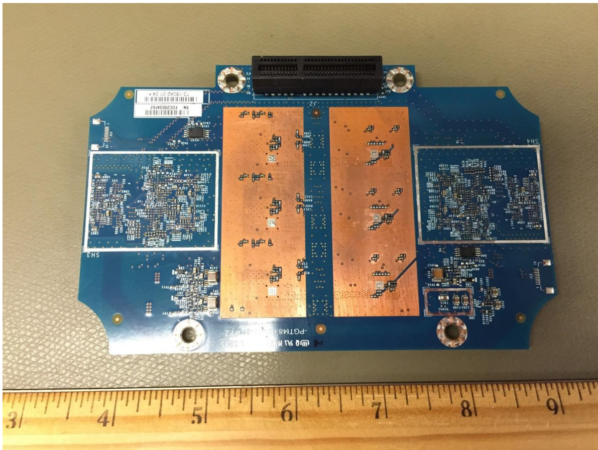
Bottom Side RF Board without Shields
