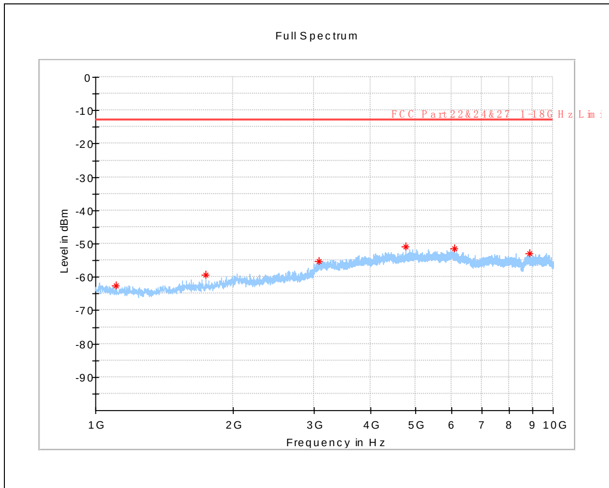
(1XEVD0 Rev A BC 0 _ CH 1013 _ 1GHz to 10GHz _ Horizontal)
