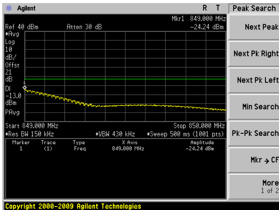
Figure Channel 26965 (841.50MHz) 1RB74
