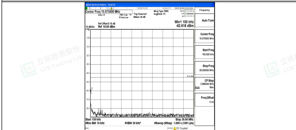
Band38_5MHz_16QAM_38225_1RB#0_0.15~30_0.15~30
