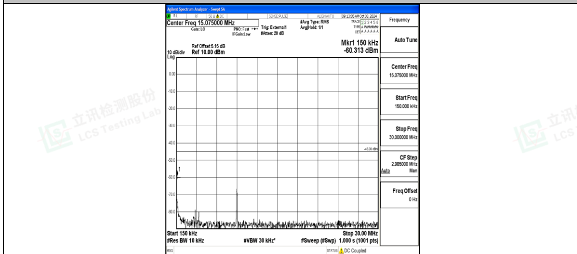
Band38_5MHz_16QAM_37775_1RB#0_0.15~30_0.15~30
