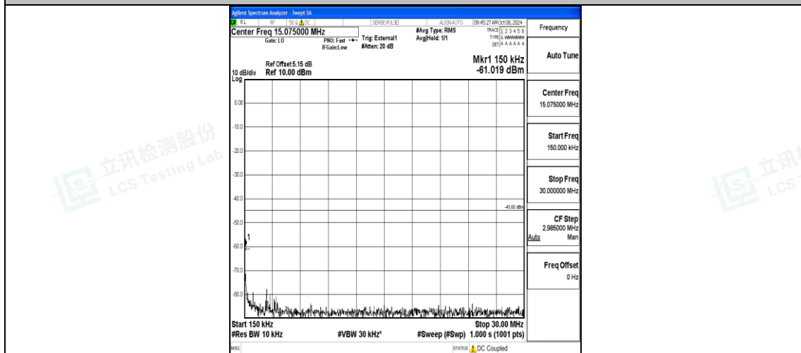
Band38_10MHz_16QAM_38200_1RB#0_0.15~30_0.15~30
