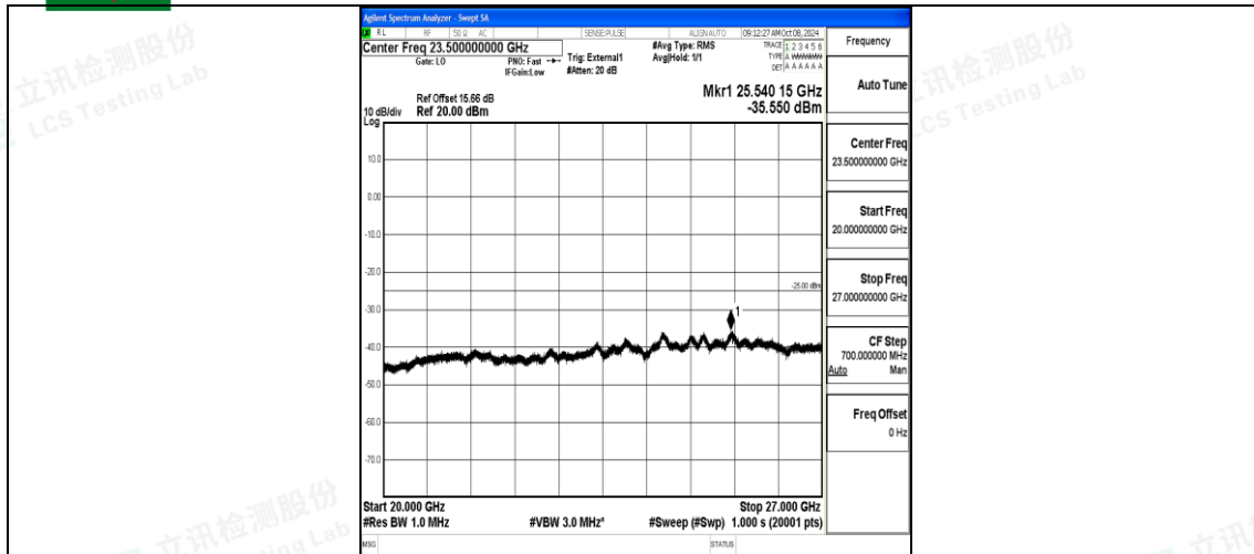
Band38_5MHz_QPSK_37775_1RB#0_20000~27000_20000~27000
