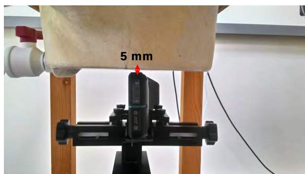
Fig.5 EUT right side to flat phantom
