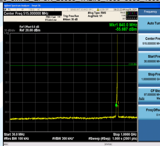
Band5_3MHz_QPSK_20635_1RB#14_30~1000_30~1000
