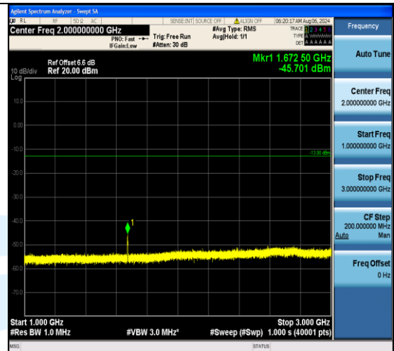
Band5_3MHz_16QAM_20525_15RB#0_1000~3000_1000~3000
