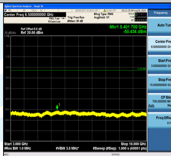
Band5_3MHz_QPSK_20635_1RB#14_3000~10000_3000~10000
