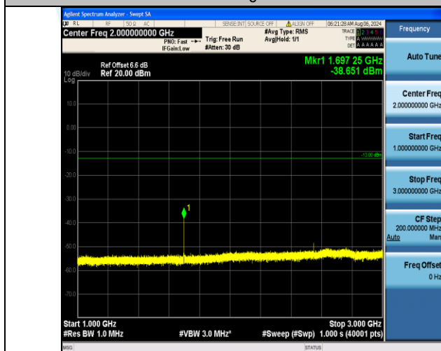
Band5_3MHz_QPSK_20635_1RB#14_1000~3000_1000~3000
