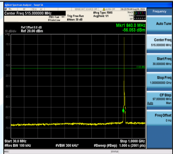
Band5_3MHz_16QAM_20635_1RB#0_30~1000_30~1000
