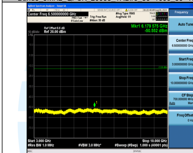
Band5_3MHz_QPSK_20635_1RB#0_3000~10000_3000~10000
