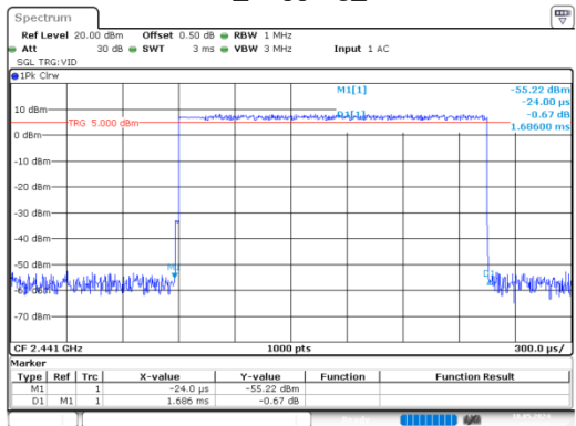
8DPSK_Hopping_3DH3
