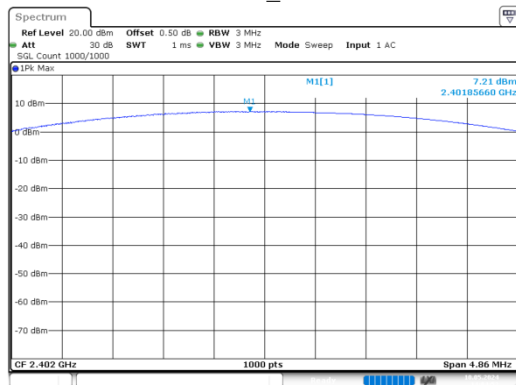
GFSK_Low
