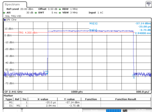
8DPSK_Hopping_3DH5
