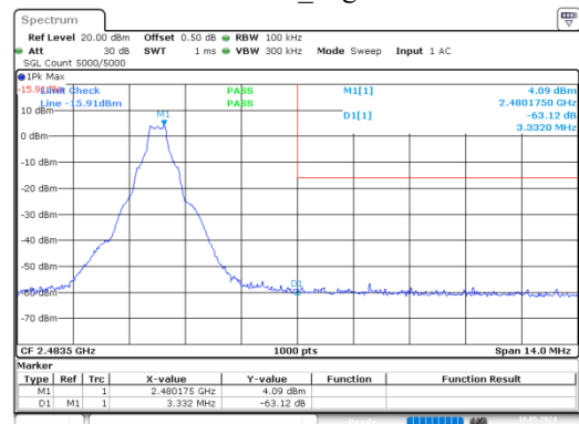
GFSK_High
