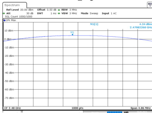
GFSK_High
