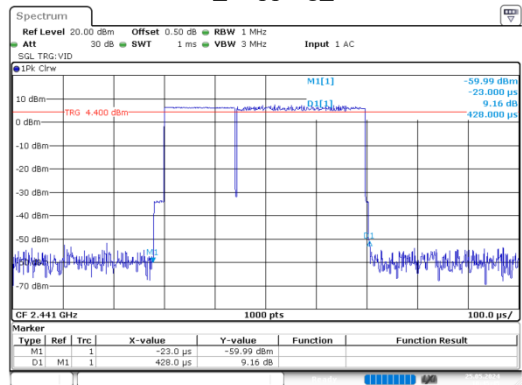
8DPSK_Hopping_3DH1
