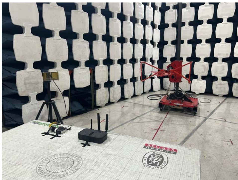
30MHz-1GHz Rear
