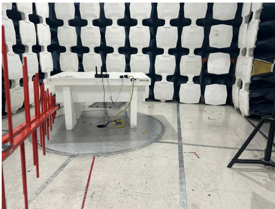
30MHz-1GHz Front
