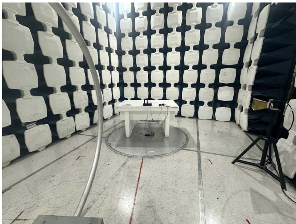
9k-30MHz Front
