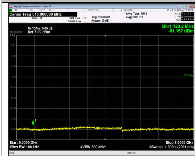
41-41-5MHz-20MHz-QPSK-QPSK-39683-39800-1RB#24-0RB#0-30~1000MHz-PASS
