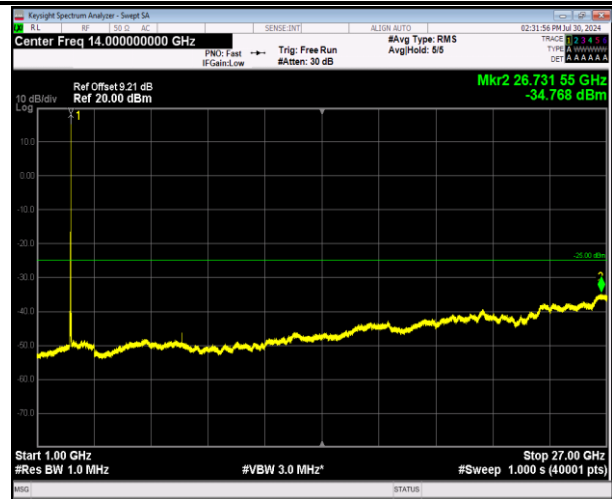
7-7-20MHz-20MHz-64QAM-64QAM-21001-21199-1RB#99- 0RB#0-1000~27000MHz-PASS
