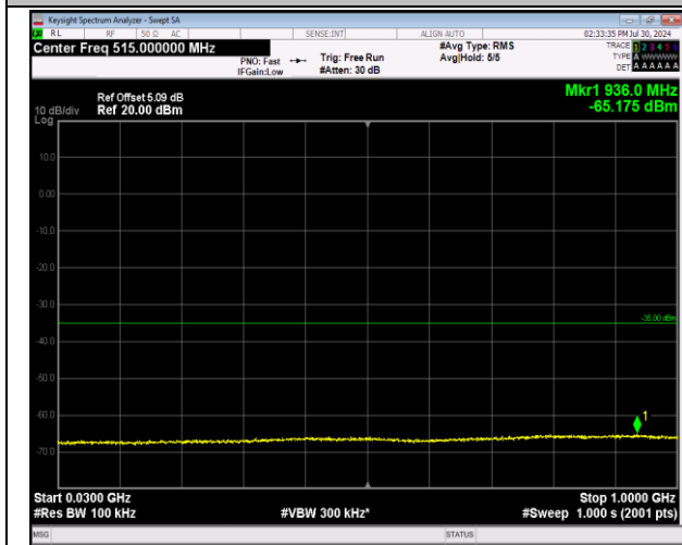
7-7-20MHz-20MHz-64QAM-64QAM-21152-21350-1RB#0 -0RB#0-30~1000MHz-PASS
