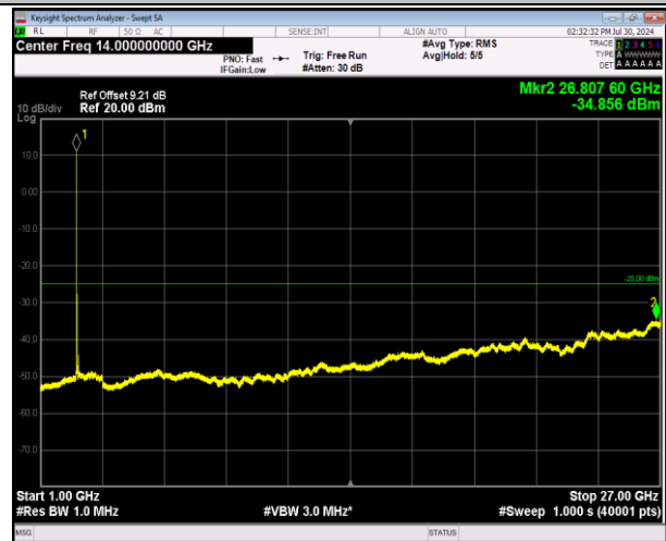
7-7-20MHz-20MHz-64QAM-64QAM-21001-21199-1RB#0-1 RB#99-1000~27000MHz-PASS
