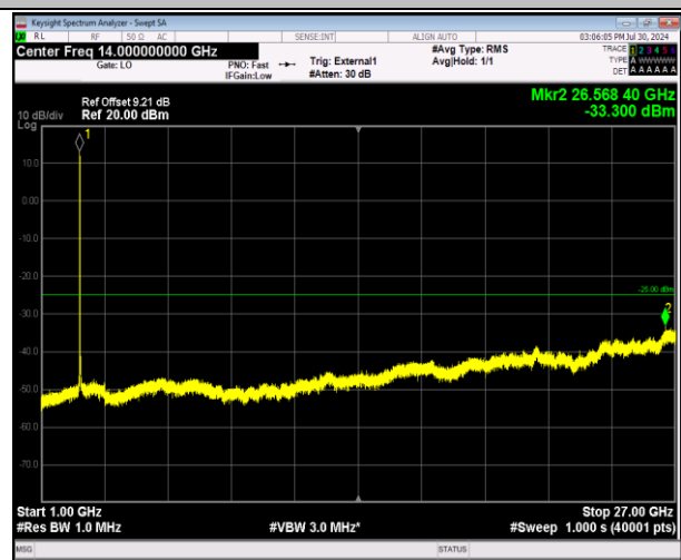
41-41-5MHz-20MHz-64QAM-64QAM-40528-40645-25RB#0 -100RB#0-1000~27000MHz-PASS
