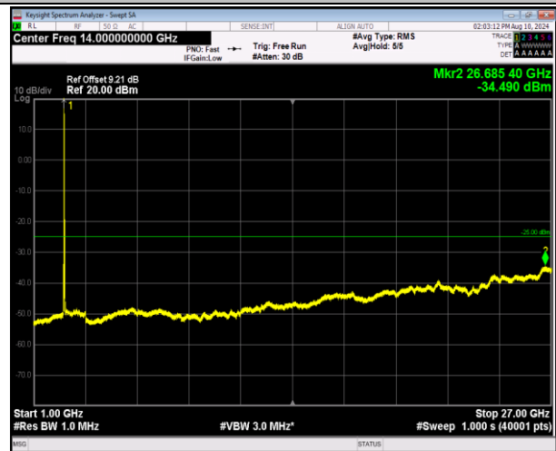
7-7-20MHz-20MHz-QPSK-QPSK-21152-21350-1RB#0-0RB #0-1000~27000MHz-PASS
