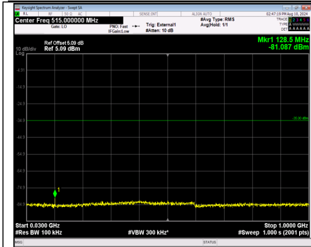
41-41-5MHz-20MHz-16QAM-16QAM-39683-39800-1RB# 0-ORB#0-30~1000MHz-PASS
