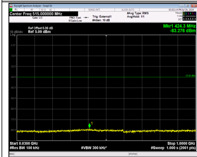
41-41-5MHz-20MHz-64QAM-64QAM-39683-39800-25RB #0-100RB#0-30~1000MHz-PASS
