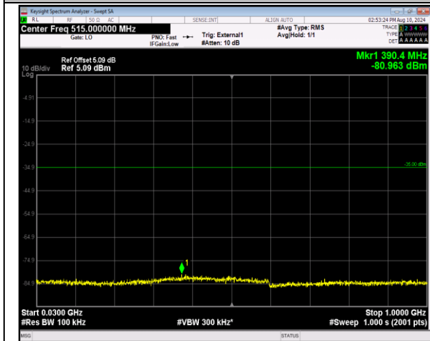
41-41-5MHz-20MHz-QPSK-QPSK-40528-40645-1RB#0-ORB#0-30~1000MHz-PASS
