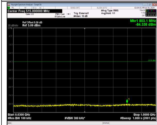
41-41-5MHz-20MHz-64QAM-64QAM-40528-40645-1RB# 0-1RB#99-30~1000MHz-PASS
