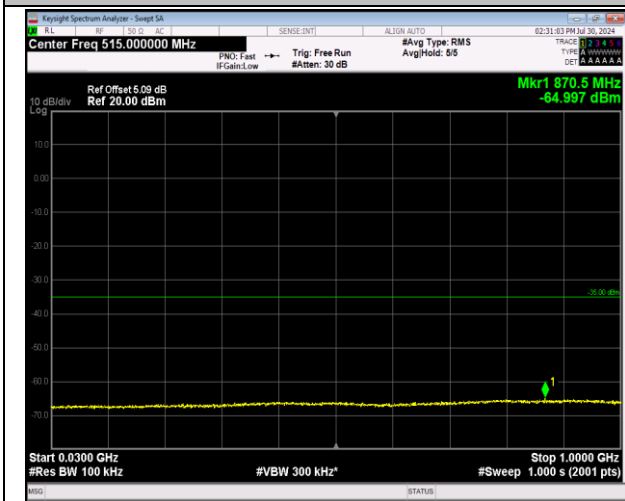
7-7-20MHz-20MHz-64QAM-64QAM-21001-21199-1RB#0 -0RB#0-30~1000MHz-PASS
