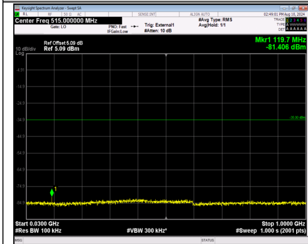
41-41-5MHz-20MHz-16QAM-16QAM-39683-39800-1RB# 24-ORB#0-30~1000MHz-PASS
