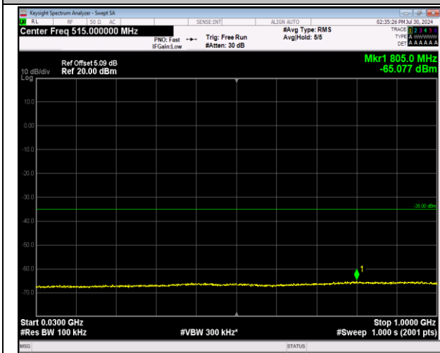
7-7-20MHz-20MHz-64QAM-64QAM-21152-21350-100RB #0-100RB#0-30~1000MHz-PASS
