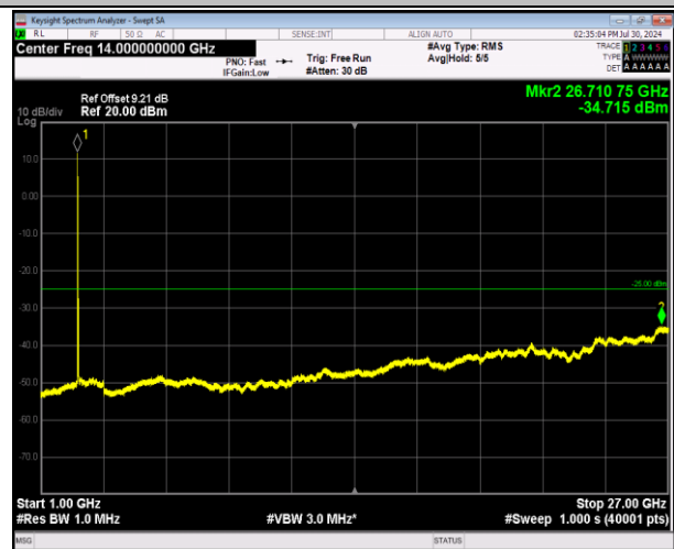
7-7-20MHz-20MHz-64QAM-64QAM-21152-21350-1RB#0-1 RB#99-1000~27000MHz-PASS
