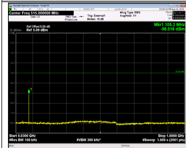
41-41-5MHz-20MHz-QPSK-QPSK-41373-41490-1RB#0-0 ORB#0-30~1000MHz-PASS
