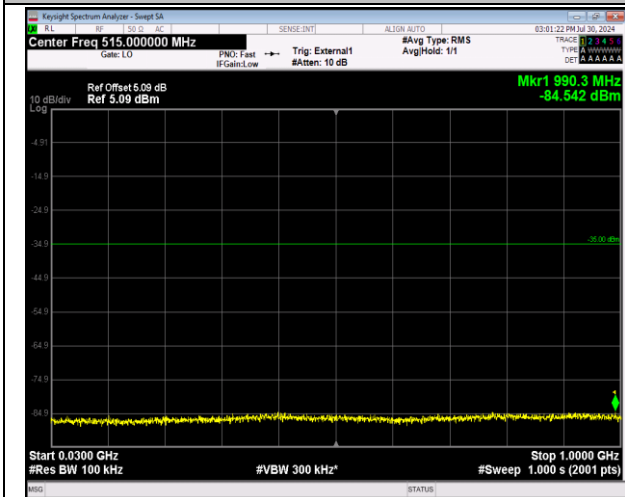
41-41-5MHz-20MHz-64QAM-64QAM-39683-39800-1RB# 0-1RB#99-30~1000MHz-PASS
