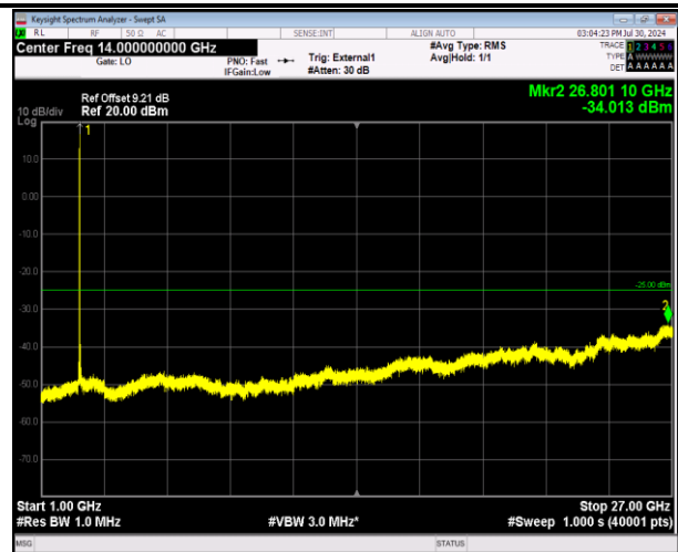
41-41-5MHz-20MHz-64QAM-64QAM-40528-40645-1RB#24 -ORB#0-1000~27000MHz-PASS
