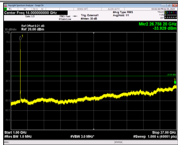
41-41-5MHz-20MHz-64QAM-64QAM-39683-39800-25RB#0 -100RB#0-1000~27000MHz-PASS
