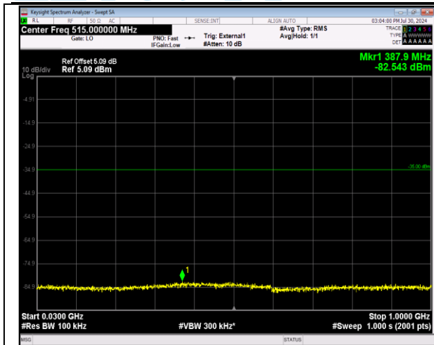
41-41-5MHz-20MHz-64QAM-64QAM-40528-40645-1RB# 24-ORB#0-30~1000MHz-PASS
