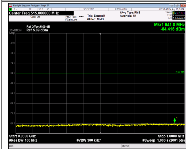
41-41-5MHz-20MHz-16QAM-16QAM-39683-39800-1RB# 0-1RB#99-30~1000MHz-PASS
