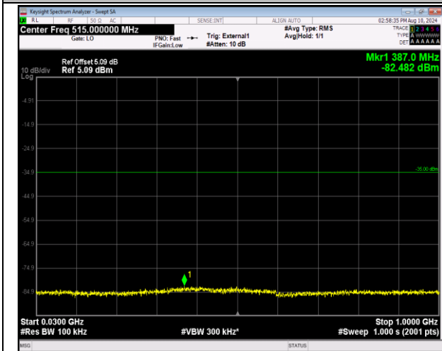
41-41-5MHz-20MHz-QPSK-QPSK-40528-40645-25RB#0-100RB#0-30~1000MHz-PASS
