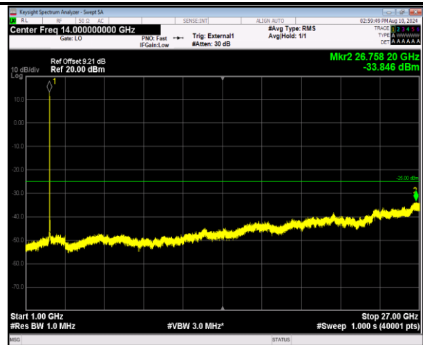
41-41-5MHz-20MHz-16QAM-16QAM-40528-40645-25RB#0 -100RB#0-1000~27000MHz-PASS
