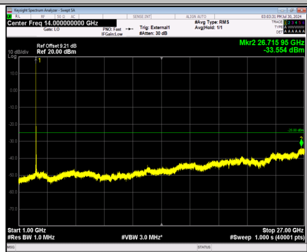
41-41-5MHz-20MHz-64QAM-64QAM-40528-40645-1RB#0- 0RB#0-1000~27000MHz-PASS
