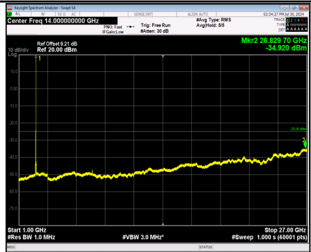
7-7-20MHz-20MHz-64QAM-64QAM-21152-21350-1RB#99- ORB#0-1000~27000MHz-PASS
