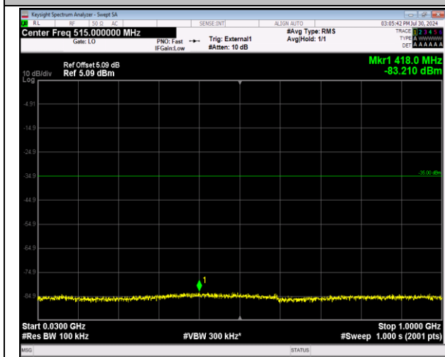
41-41-5MHz-20MHz-64QAM-64QAM-40528-40645-25RB #0-100RB#0-30~1000MHz-PASS
