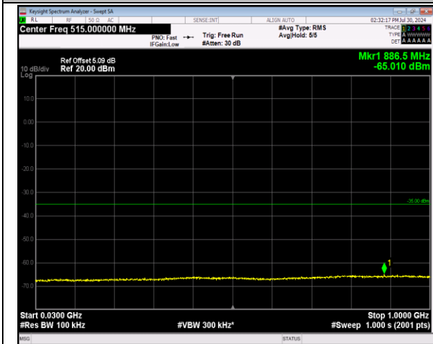
7-7-20MHz-20MHz-64QAM-64QAM-21001-21199-1RB#0 -1RB#99-30~1000MHz-PASS
