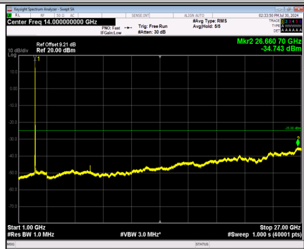
7-7-20MHz-20MHz-64QAM-64QAM-21152-21350-1RB#0-0 RB#0-1000~27000MHz-PASS
