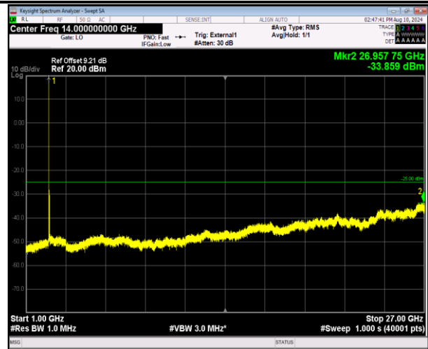
41-41-5MHz-20MHz-16QAM-16QAM-39683-39800-1RB#0- ORB#0-1000~27000MHz-PASS
