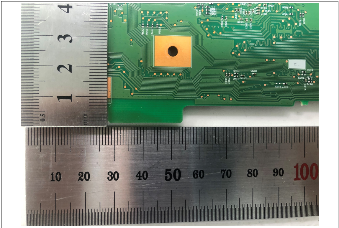
<Wifi Antenna>
