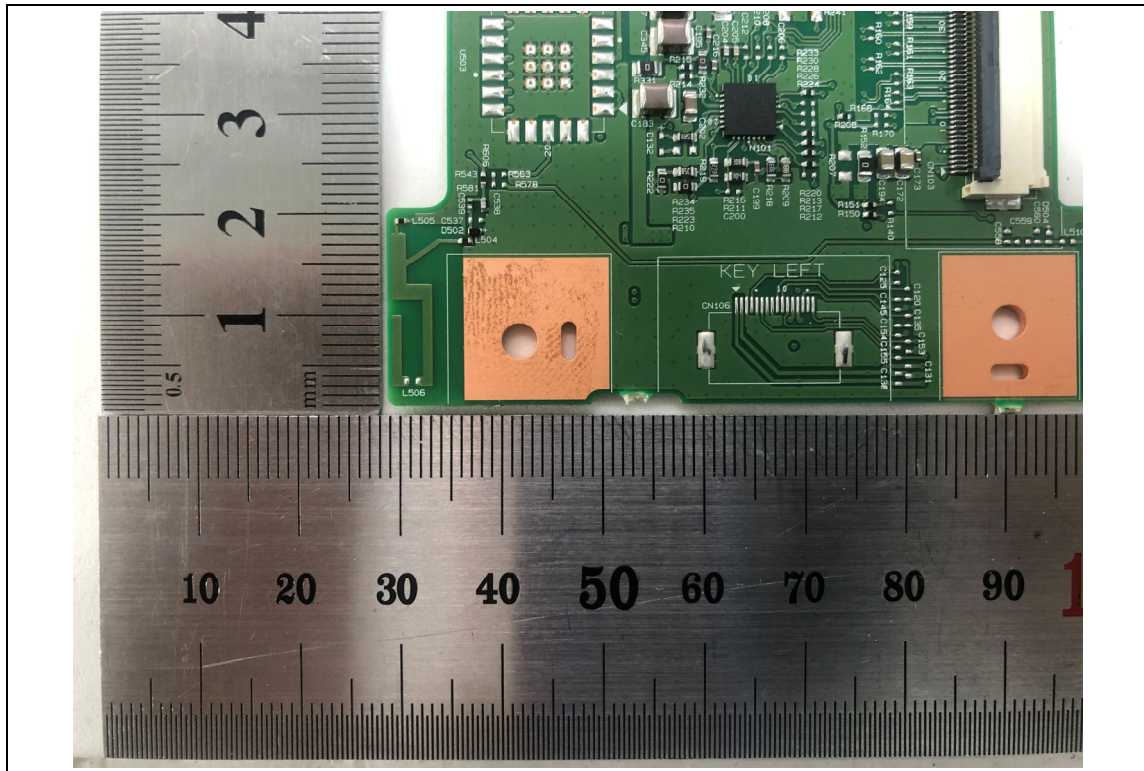
<BT Antenna>
