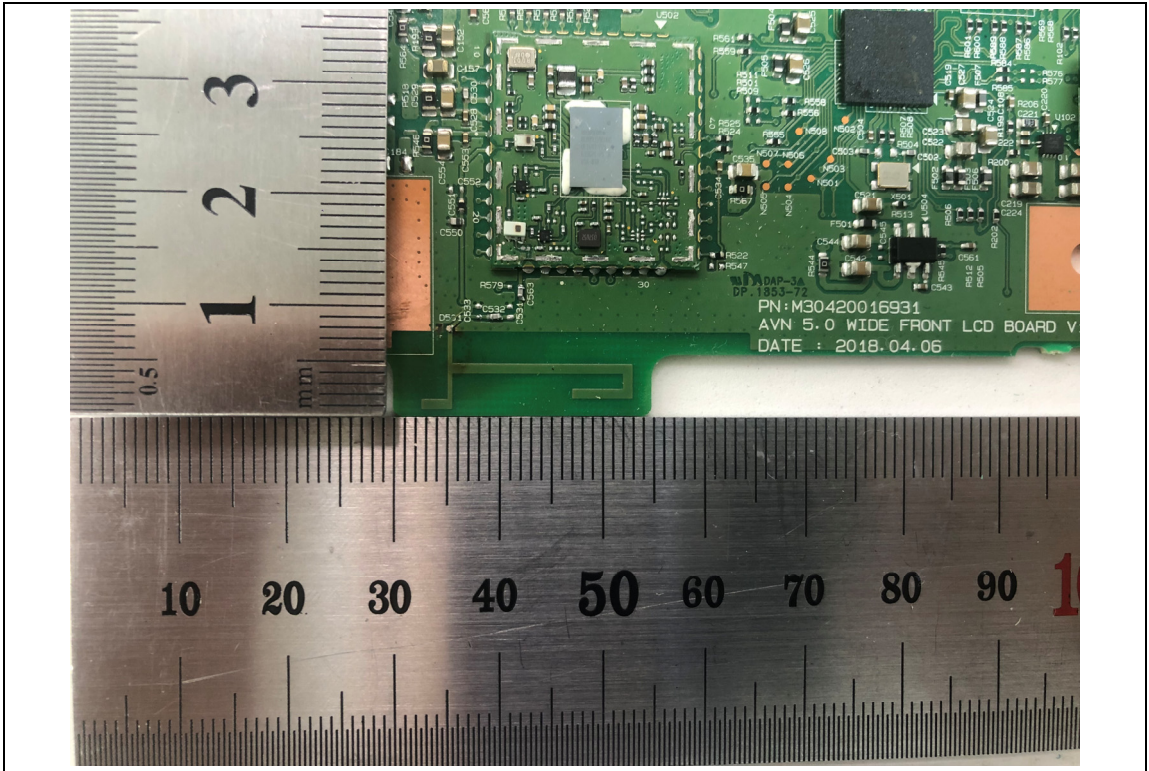
<Wifi Antenna>
