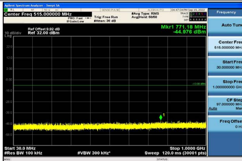
Band2-10MHz-16QAM-18900-1RB#0-30~1000MHz
