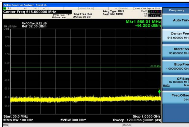
Band4-5MHz-QPSK-19975-1RB#0-30~1000MHz
