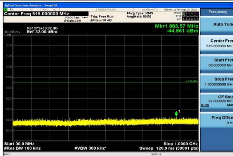
Band4-1.4MHz-16QAM-20175-1RB#0-30~1000MHz
