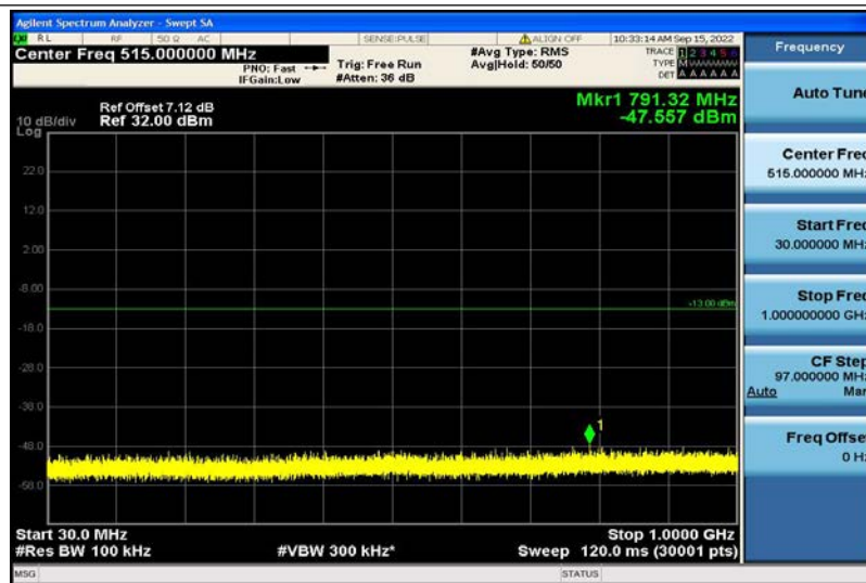
Band2-5MHz-16QAM-18625-1RB#0-30~1000MHz
