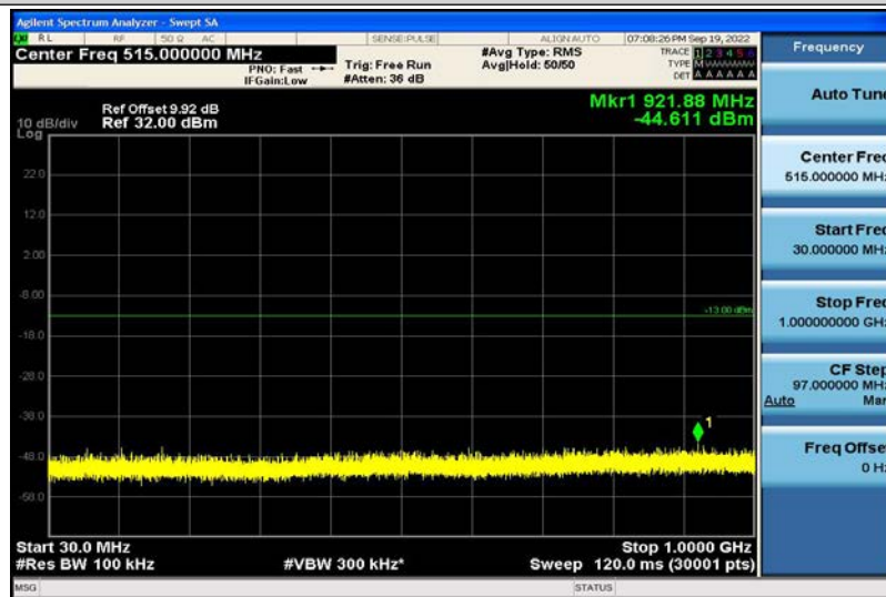
Band4-10MHz-16QAM-20350-1RB#0-30~1000MHz
