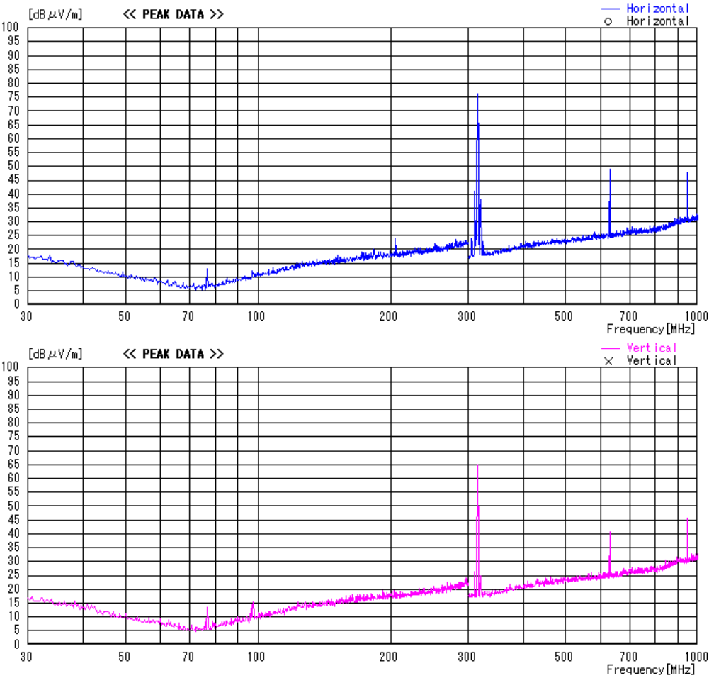
Figure 5. 30-1000MHz spectrum chart
