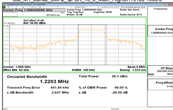
Cat_M1_Band2_3MHz_QPSK_15_0_Main_HighCH19185-1908.5
