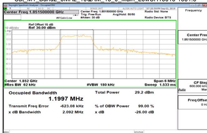
Cat_M1_Band2_3MHz_16QAM_15_0_Main_LowCH18615-1851.5
