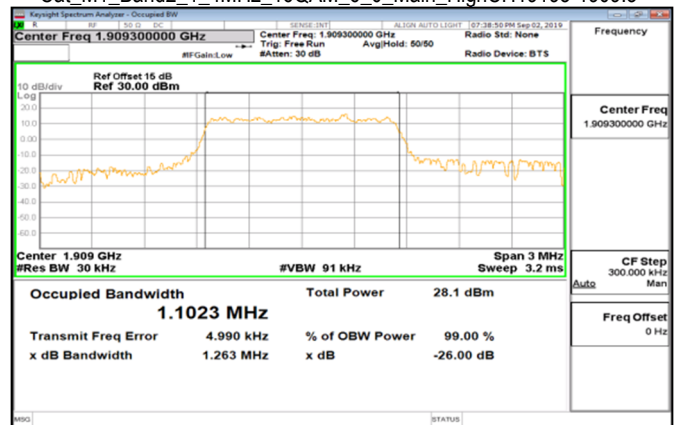
Cat M1_Band2_1_4MHz_16QAM_6_0_Main_HighCH19193-1909.3
