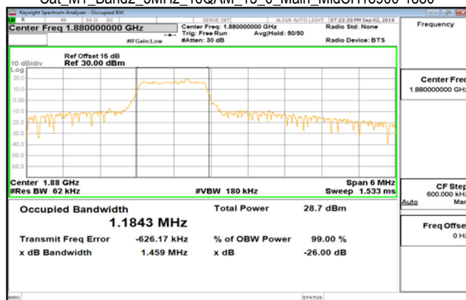
Cat_M1_Band2_3MHz_16QAM_15_0_Main_MidCH18900-1880
