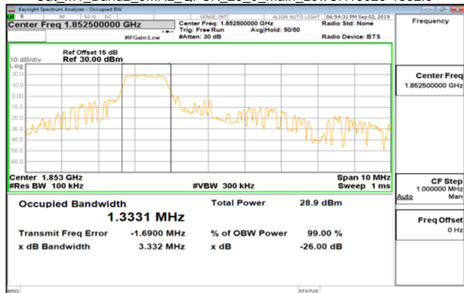
Cat_M1_Band2_5MHz_QPSK_25_0_Main_LowCH18625-1852.5
