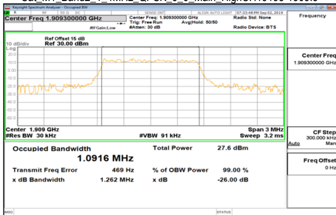
Cat M1_Band2_1_4MHz_QPSK_6_0_Main_HighCH19193-1909.3
