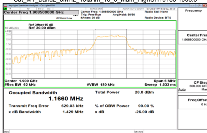
Cat_M1_Band2_3MHz_16QAM_15_0_Main_HighCH19185-1908.5
