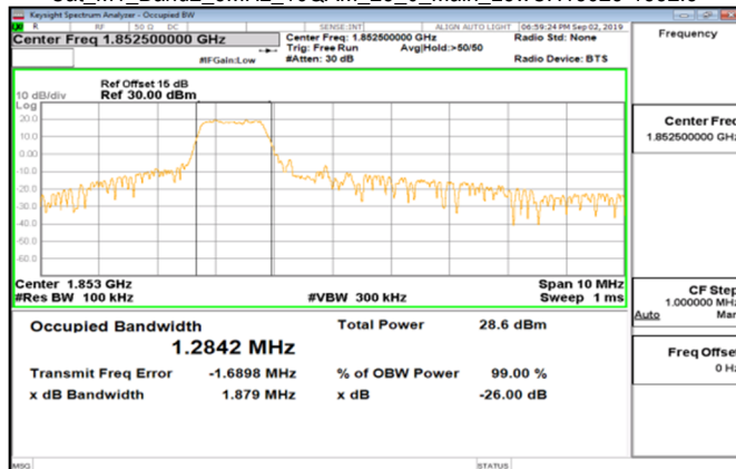
Cat_M1_Band2_5MHz_16QAM_25_0_Main_LowCH18625-1852.5
