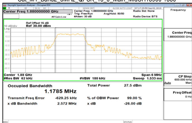
Cat_M1_Band2_3MHz_QPSK_15_0_Main_MidCH18900-1880
