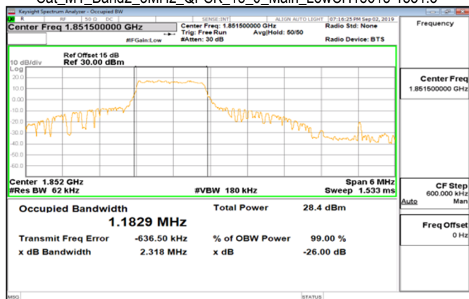
Cat_M1_Band2_3MHz_QPSK_15_0_Main_LowCH18615-1851.5
