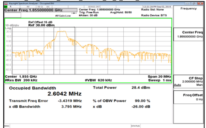
Cat_M1_Band2_10MHz_16QAM_50_0_Main_LowCH18650-1855
