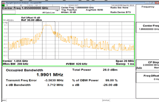
Cat_M1_Band2_10MHz_QPSK_50_0_Main_LowCH18650-1855
