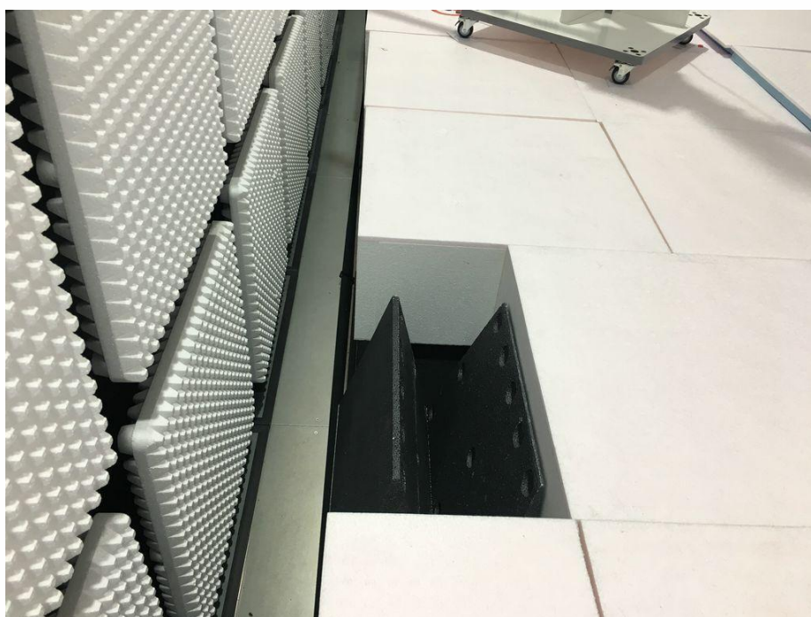
Radiated spurious emission Test Setup-4(Above 1GHz) There is absorber on the ground floor
