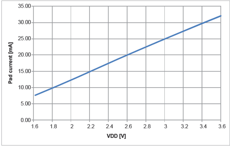
Max sink current vs Voltage, high drive
