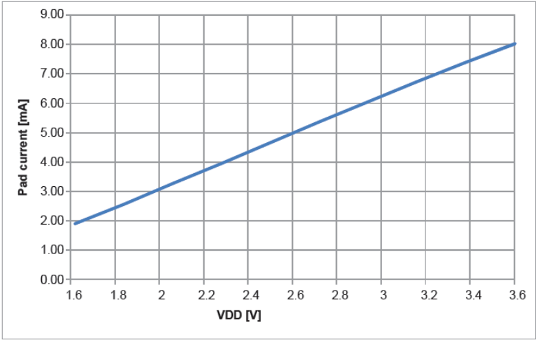
Max sink current vs Voltage, standard drive
