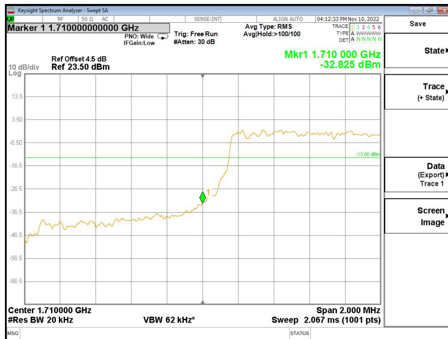
Band4-Low Channel-1.4MHz Bandwidth-6RB-QPSK
