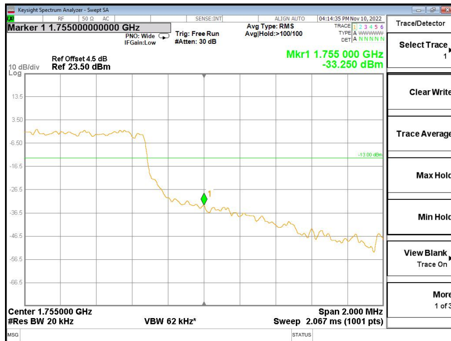
Band4-High Channel-3MHz Bandwidth-5RB-16QAM
