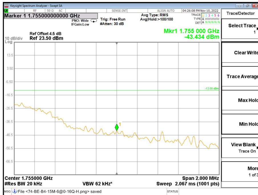
Band4-High Channel-20MHz Bandwidth-5RB-16QAM
