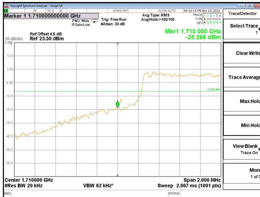
Band4-Low Channel-5MHz Bandwidth-5RB-16QAM
