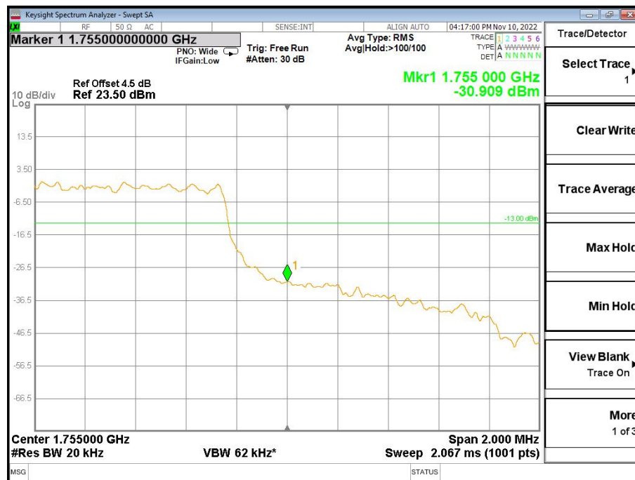
Band4-High Channel-5MHz Bandwidth-6RB-QPSK
