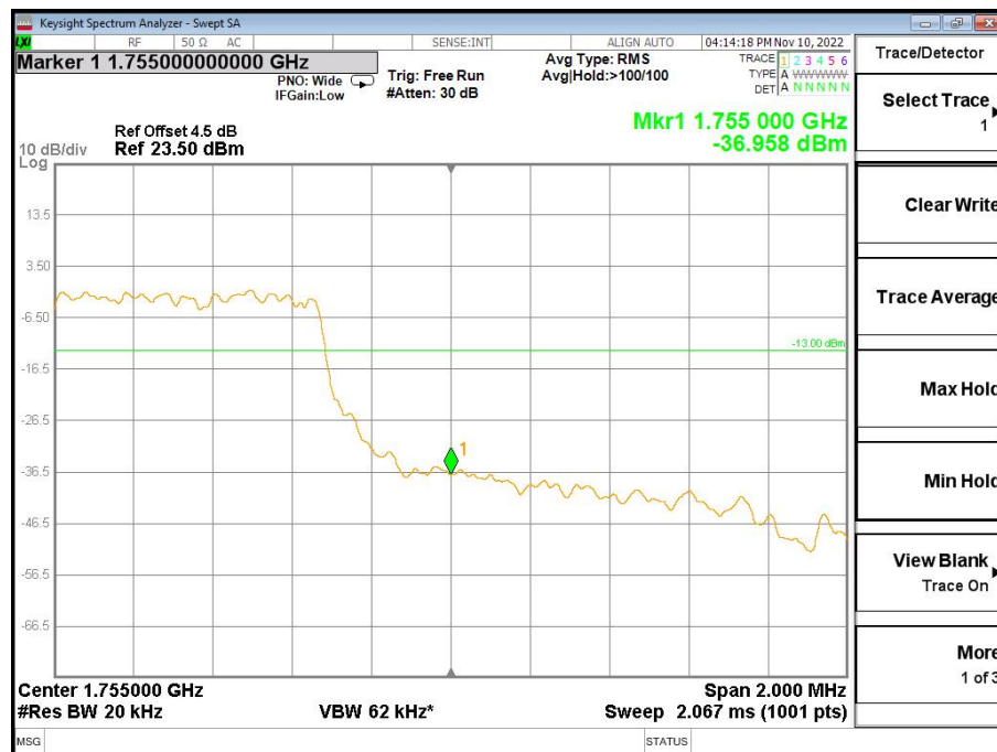
Band4-High Channel-3MHz Bandwidth-6RB-QPSK
