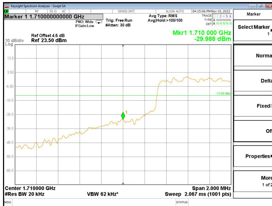
Band4-Low Channel-3MHz Bandwidth-5RB-16QAM
