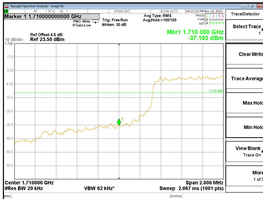
Band4-Low Channel-3MHz Bandwidth-6RB-QPSK
