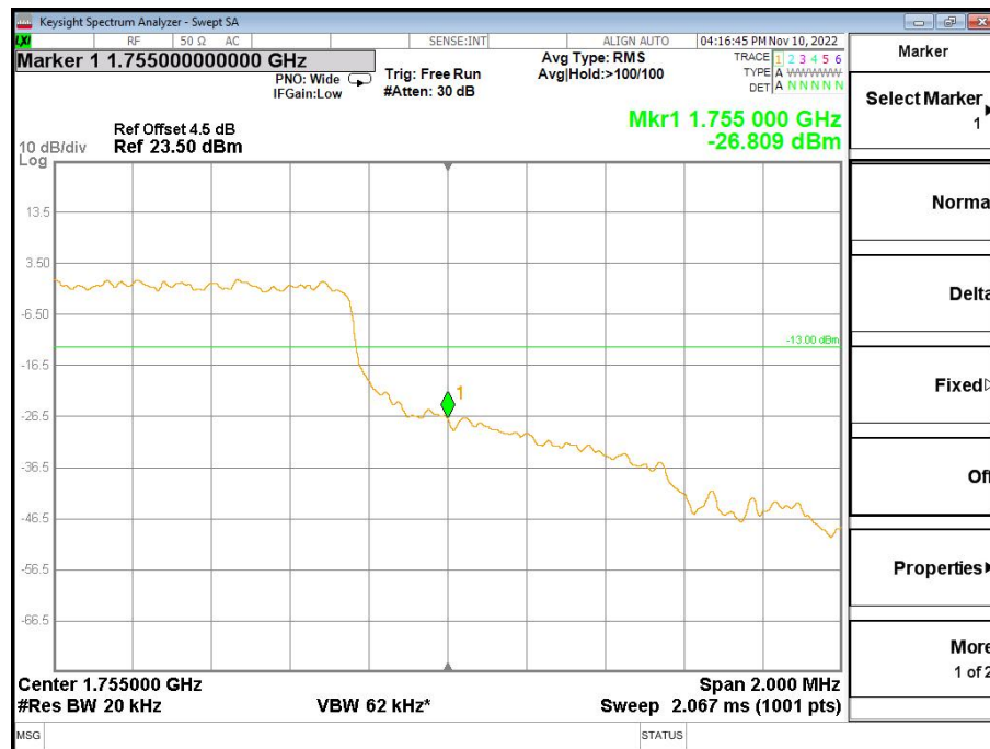
Band4-High Channel-5MHz Bandwidth-5RB-16QAM
