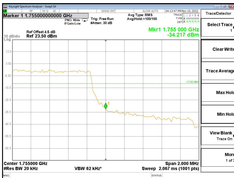
Band4-High Channel-1.4MHz Bandwidth-6RB-QPSK
