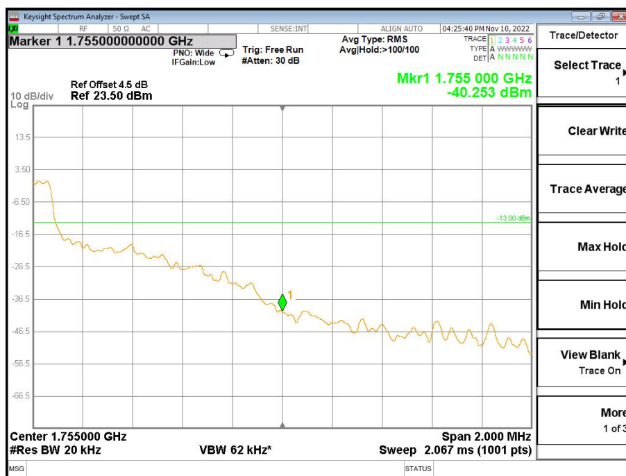
Band4-High Channel-15MHz Bandwidth-5RB-16QAM
