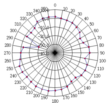
Vertical at 2480MHz
