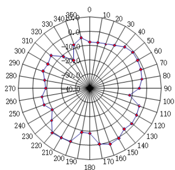
Horizontal at 2480MHz
