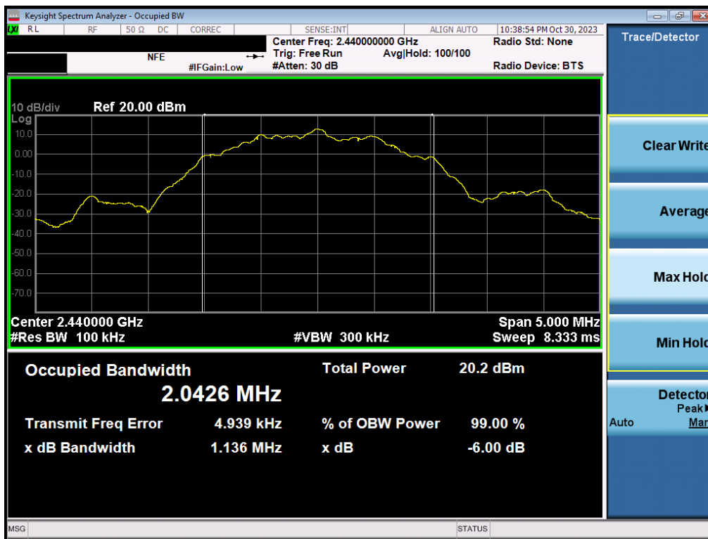
Plot 7-35. 6dB Bandwidth Plot (Bluetooth (LE), 2Mbps – Ch. 19) – MIMO ANT2
