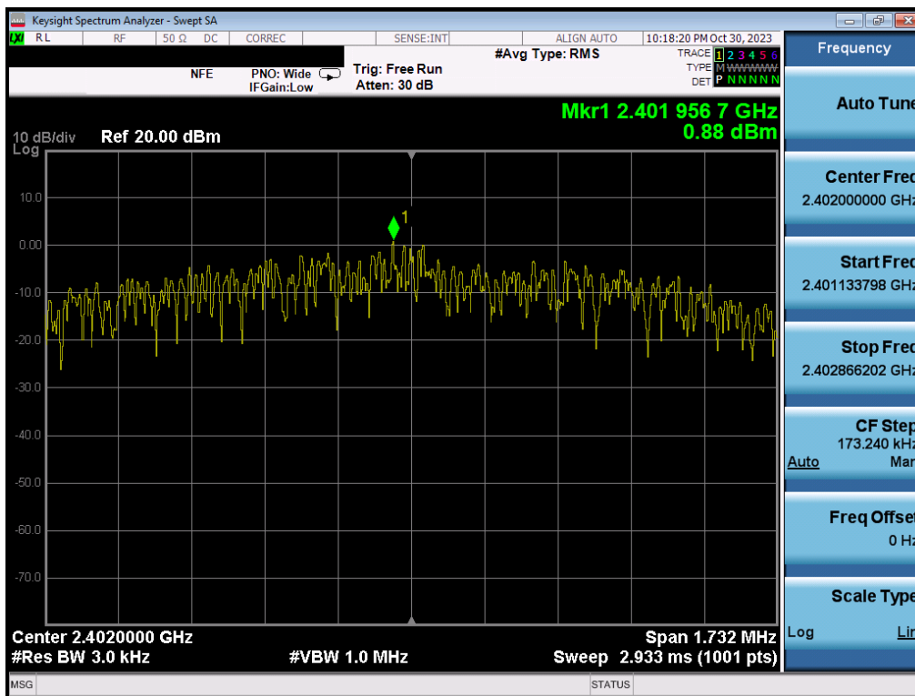
Plot 7-94. Power Spectral Density Plot (Bluetooth (LE), 2Mbps – Ch. 0) – SISO ANT2
