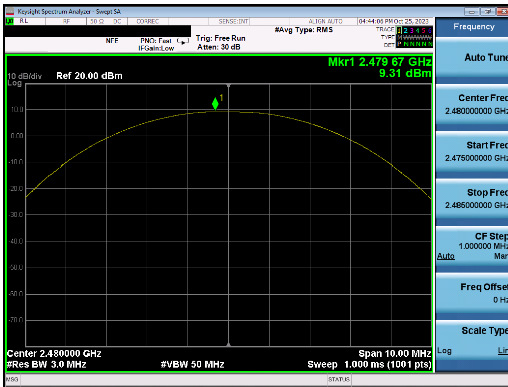
Plot 7-42. Peak Power Plot (Bluetooth (LE), 500kbps – Ch. 39) – SISO ANT1
