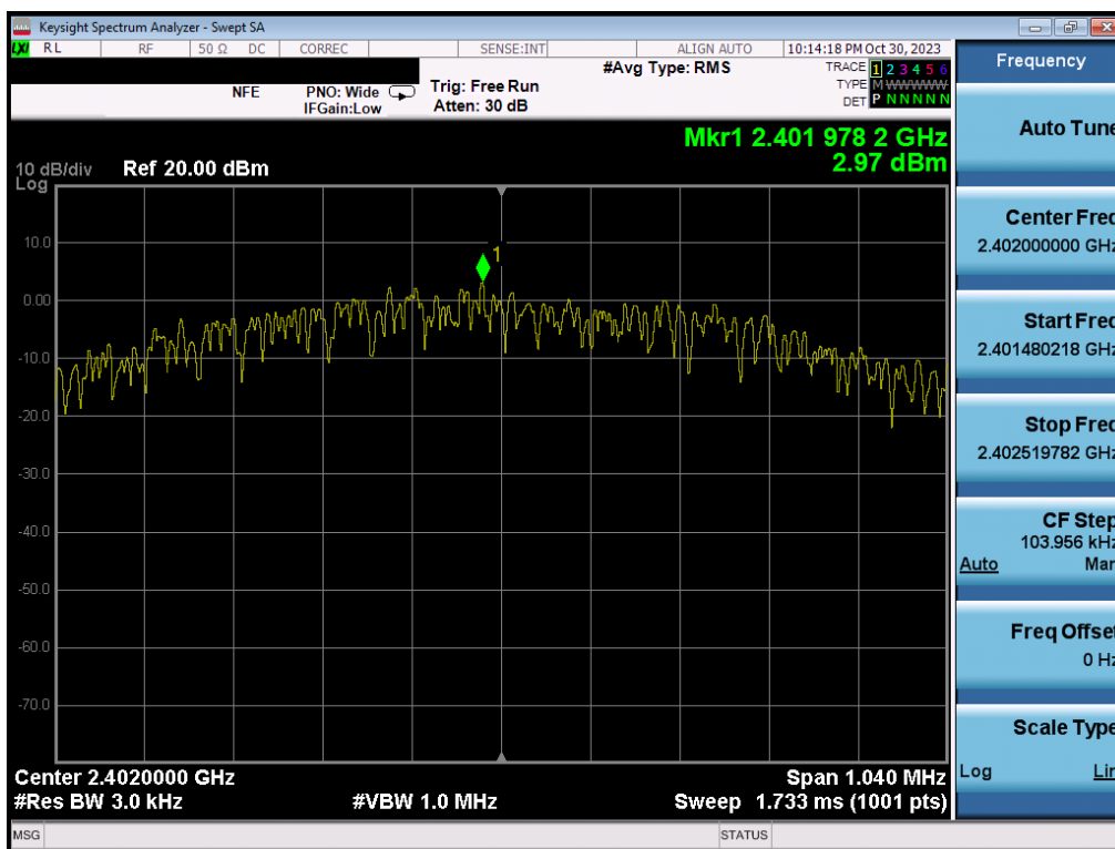
Plot 7-91. Power Spectral Density Plot (Bluetooth (LE), 1Mbps – Ch. 0) – SISO ANT2
