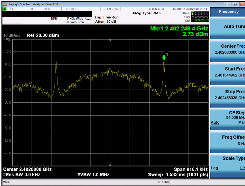
Plot 7-73. Power Spectral Density Plot (Bluetooth (LE), 125kbps – Ch. 0) – SISO ANT1
