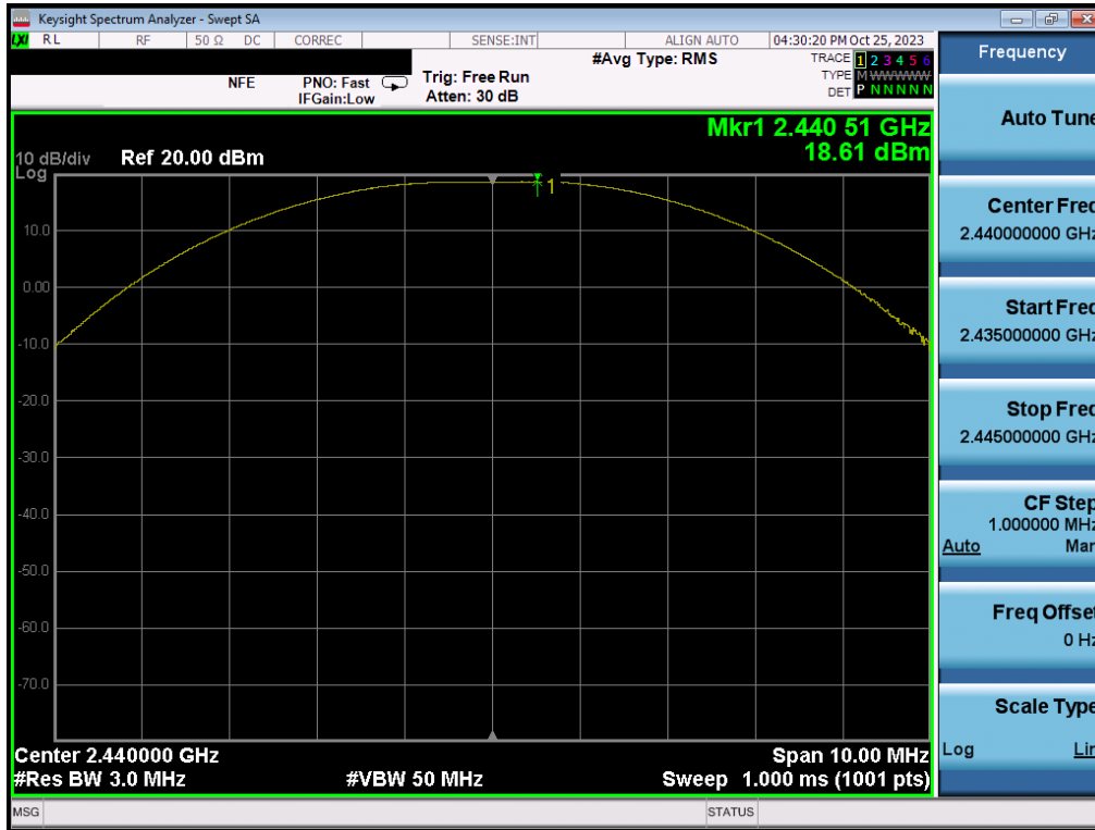
Plot 7-59. Peak Power Plot (Bluetooth (LE), 2Mbps – Ch. 19) – SISO ANT2
