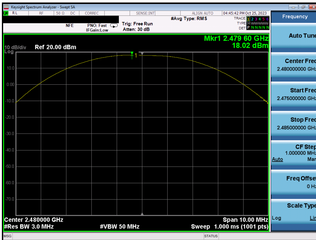
Plot 7-48. Peak Power Plot (Bluetooth (LE), 2Mbps – Ch. 39) – SISO ANT1
