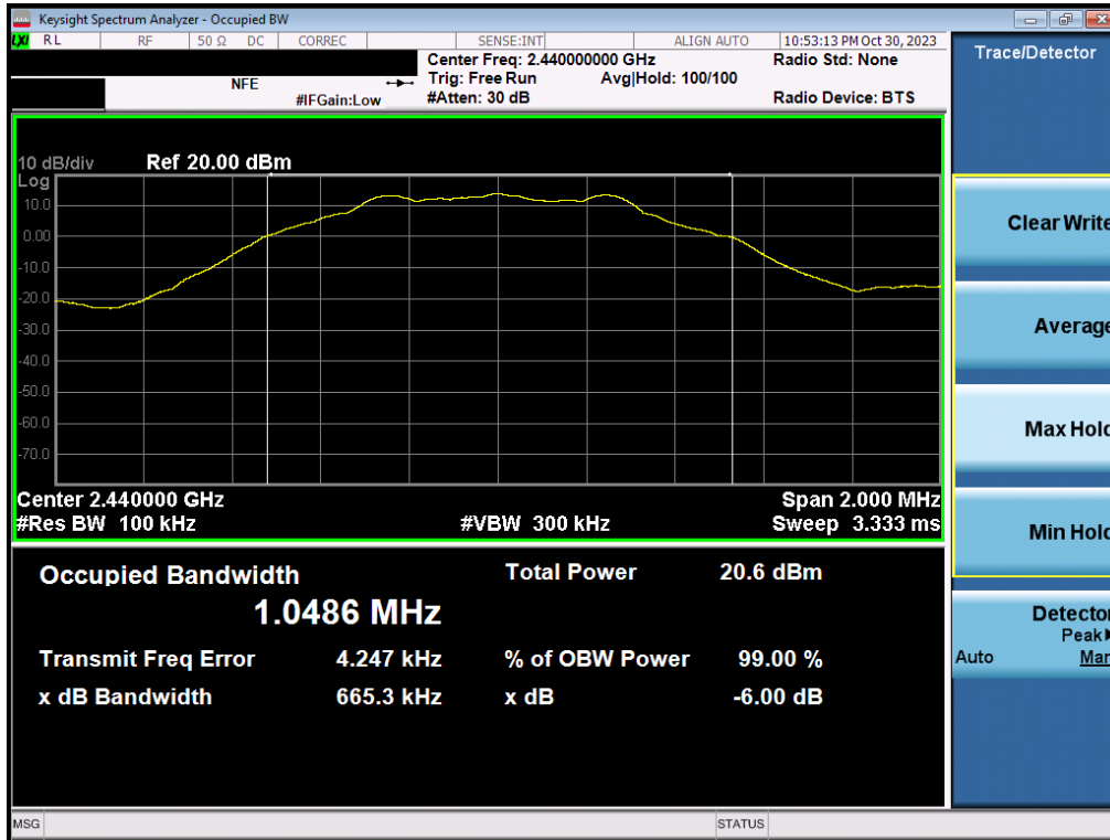
Plot 7-26. 6dB Bandwidth Plot (Bluetooth (LE), 1Mbps – Ch. 19) – MIMO ANT1
