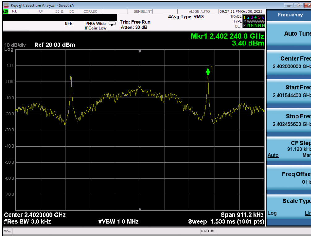
Plot 7-85. Power Spectral Density Plot (Bluetooth (LE), 125kbps – Ch. 0) – SISO ANT2
