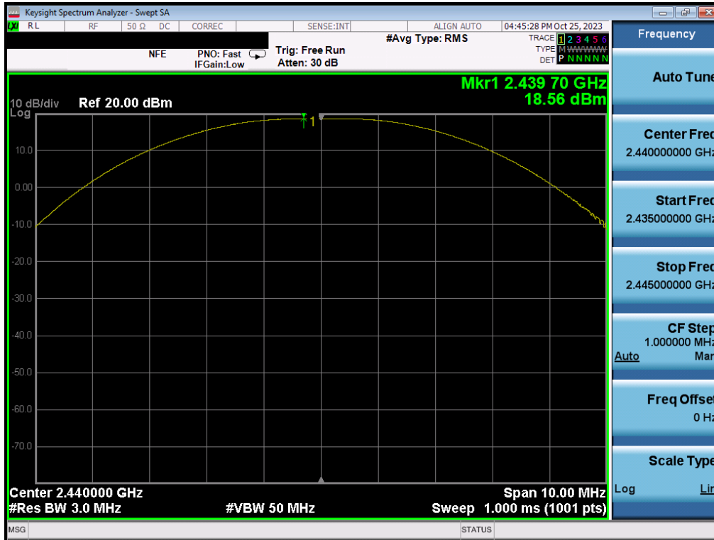
Plot 7-47. Peak Power Plot (Bluetooth (LE), 2Mbps – Ch. 19) – SISO ANT1
