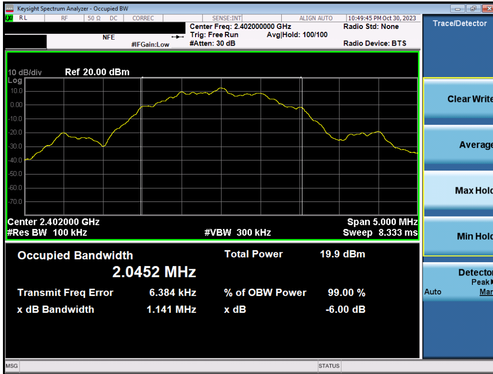
Plot 7-28. 6dB Bandwidth Plot (Bluetooth (LE), 2Mbps – Ch. 0) – MIMO ANT1
