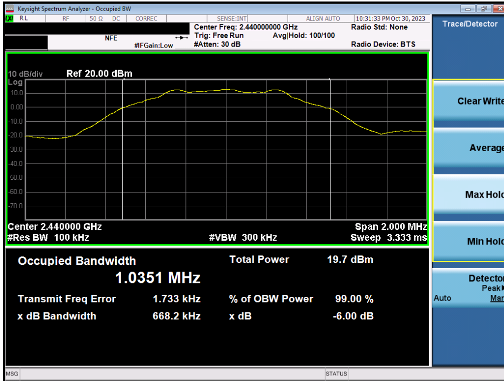
Plot 7-32. 6dB Bandwidth Plot (Bluetooth (LE), 1Mbps – Ch. 19) – MIMO ANT2
