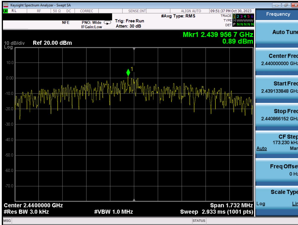
Plot 7-83. Power Spectral Density Plot (Bluetooth (LE), 2Mbps – Ch. 19) – SISO ANT1
