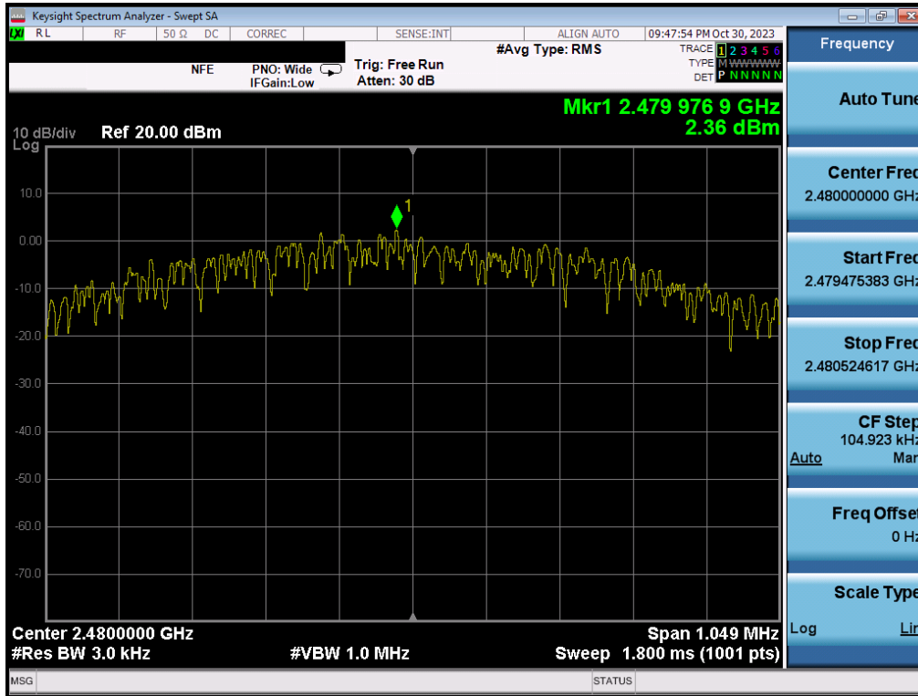
Plot 7-81. Power Spectral Density Plot (Bluetooth (LE), 1Mbps – Ch. 39) – SISO ANT1
