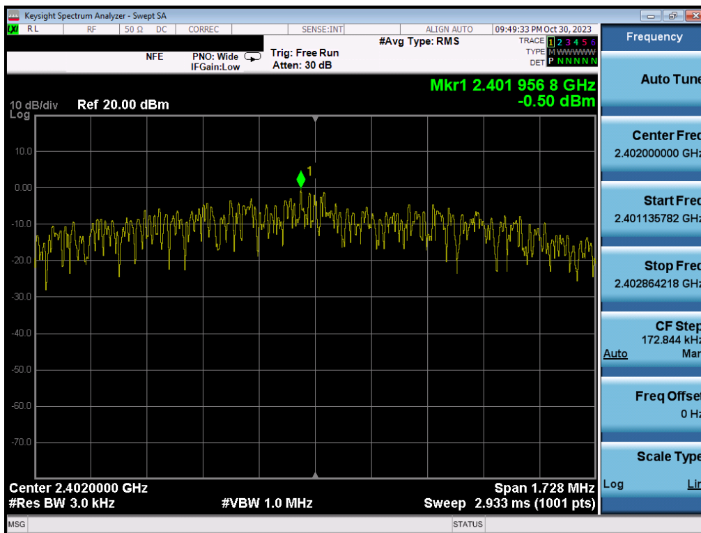
Plot 7-82. Power Spectral Density Plot (Bluetooth (LE), 2Mbps – Ch. 0) – SISO ANT1
