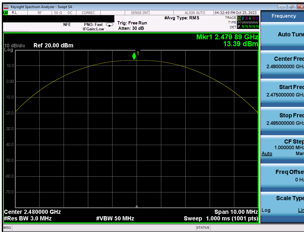
Plot 7-69. Peak Power Plot (Bluetooth (LE), 1Mbps – Ch. 39) – MIMO ANT2
