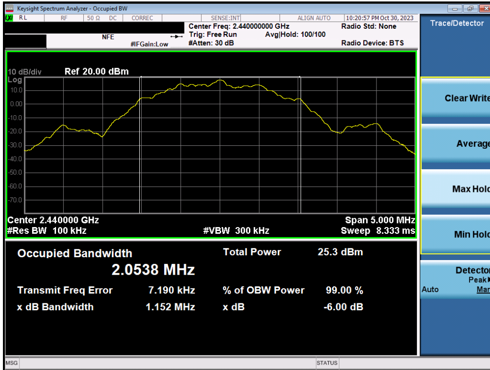
Plot 7-23. 6dB Bandwidth Plot (Bluetooth (LE), 2Mbps – Ch. 19) – SISO ANT2
