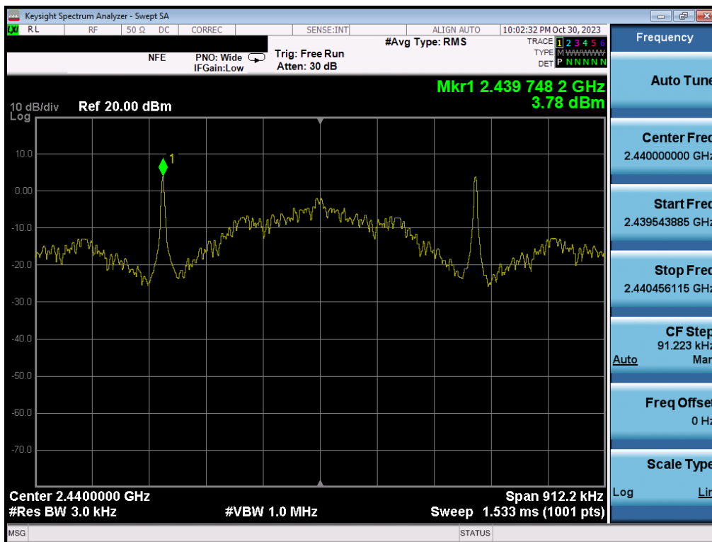
Plot 7-86. Power Spectral Density Plot (Bluetooth (LE), 125kbps – Ch. 19) – SISO ANT2
