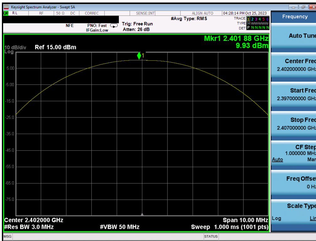
Plot 7-52. Peak Power Plot (Bluetooth (LE), 500kbps – Ch. 0) – SISO ANT2
