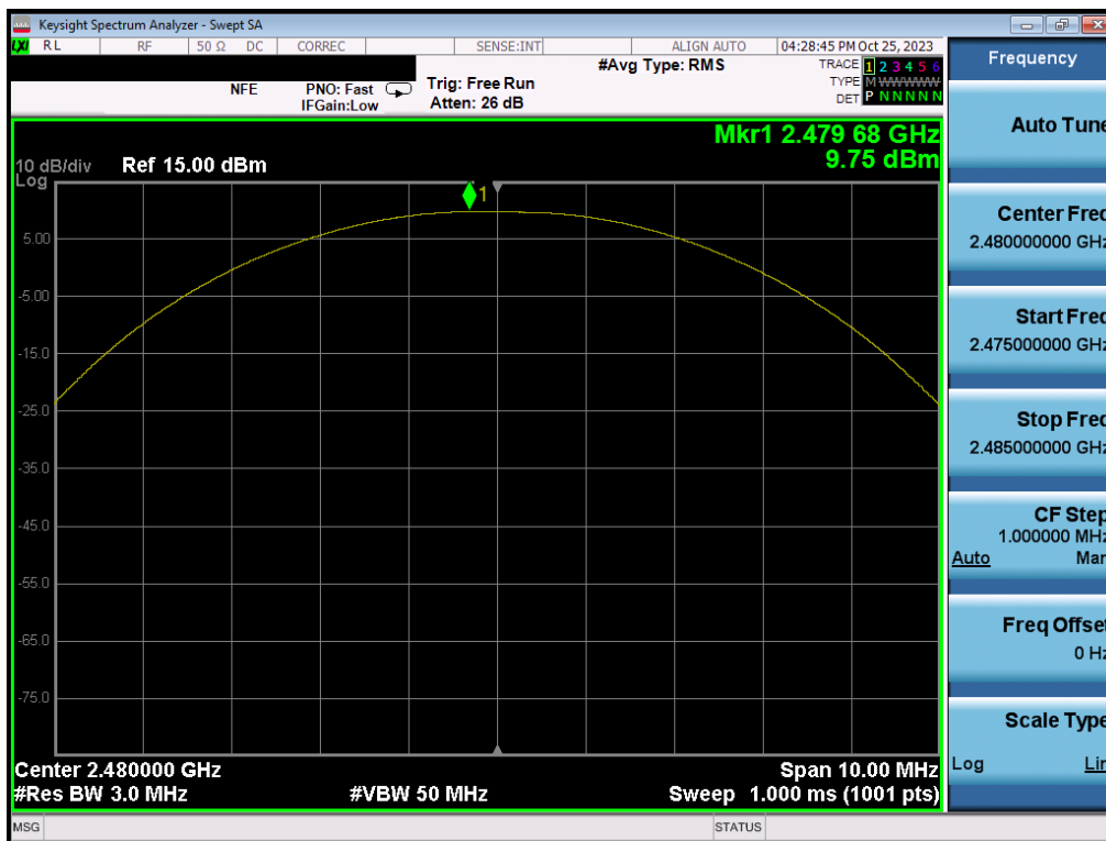
Plot 7-54. Peak Power Plot (Bluetooth (LE), 500kbps – Ch. 39) – SISO ANT
