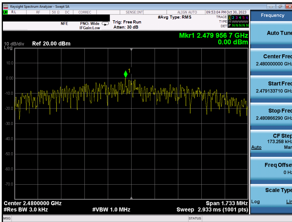
Plot 7-84. Power Spectral Density Plot (Bluetooth (LE), 2Mbps – Ch. 39) – SISO ANT1
