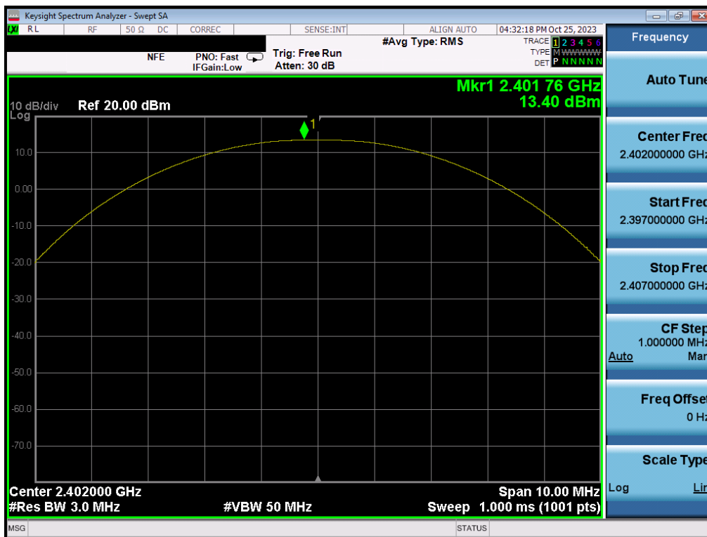
Plot 7-67. Peak Power Plot (Bluetooth (LE), 1Mbps – Ch. 0) – MIMO ANT2
