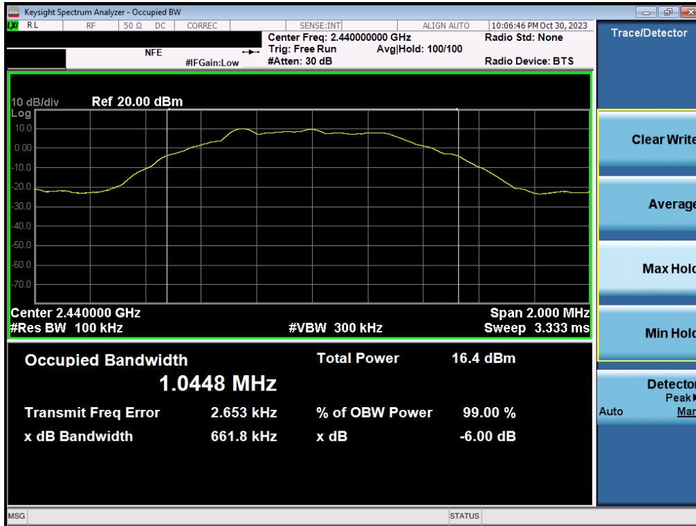
Plot 7-17. 6dB Bandwidth Plot (Bluetooth (LE), 500kbps – Ch. 19) – SISO ANT2
