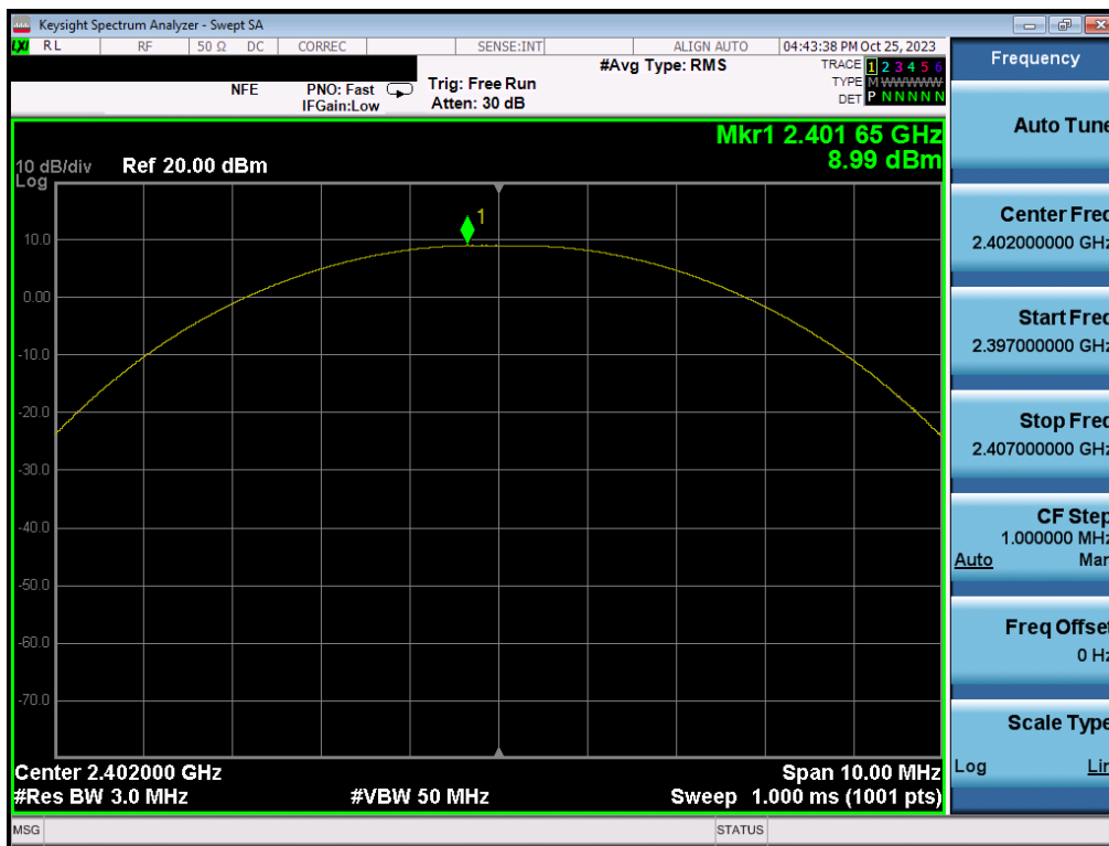
Plot 7-40. Peak Power Plot (Bluetooth (LE), 500kbps – Ch. 0) – SISO ANT1
