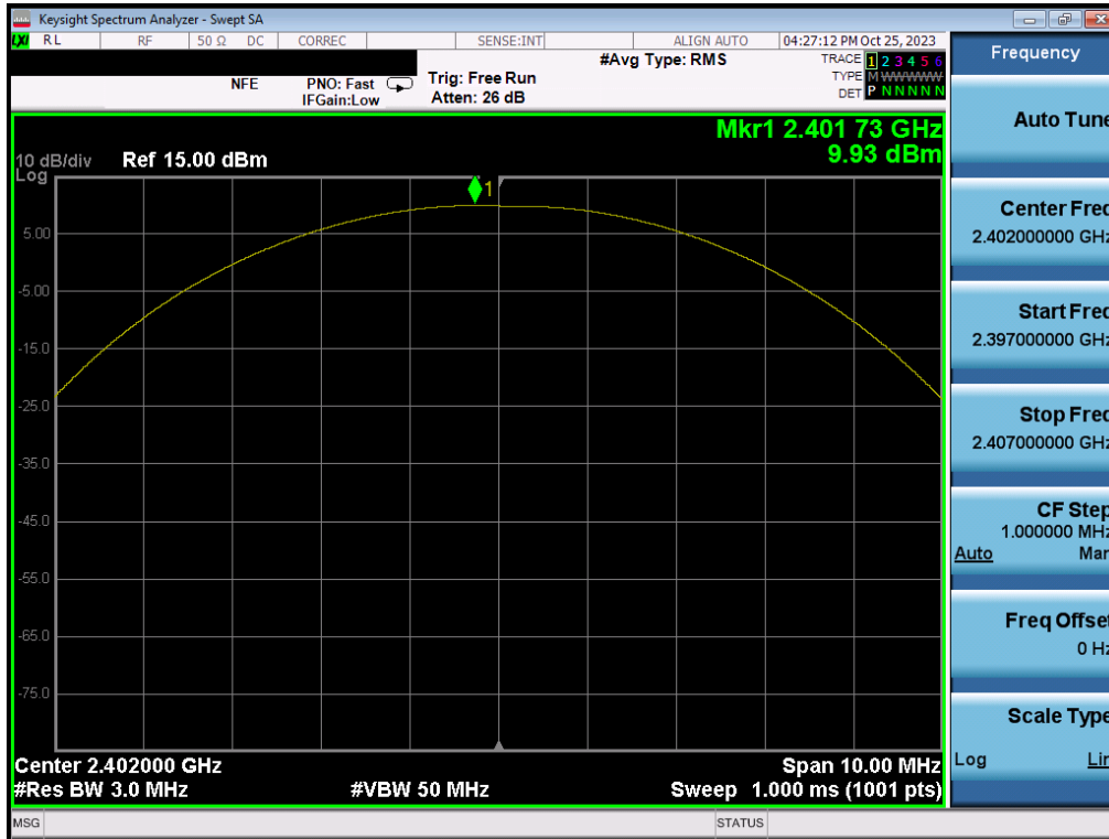
Plot 7-49. Peak Power Plot (Bluetooth (LE), 125kbps - Ch. 0) - SISO ANT2
