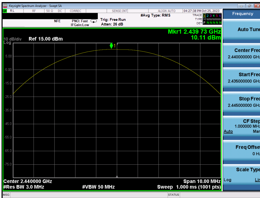
Plot 7-50. Peak Power Plot (Bluetooth (LE), 125kbps - Ch. 19) - SISO ANT2
