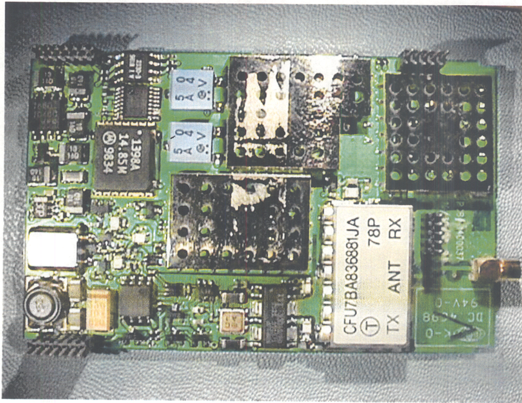
Figure3:ModemInternalView–RadioBoardTopSide
