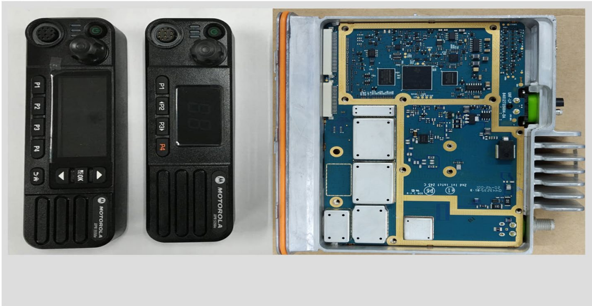
Colour Display Control Head For XPR 5550e Numeric Display Control Head For XPR 5350e
