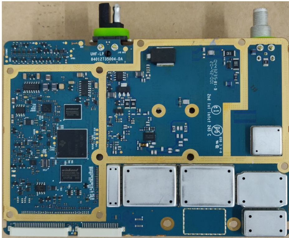
RF board with Shields (Bottom)
