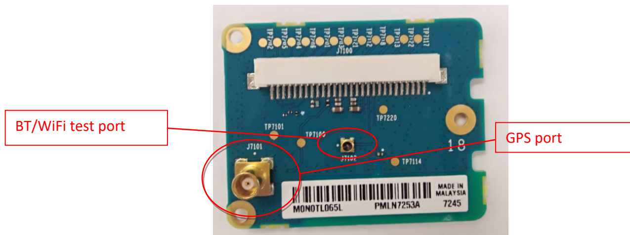
Expansion board (Top)
