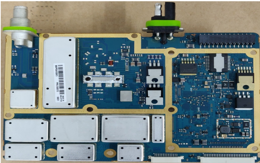
RF board with Shields (Top)
