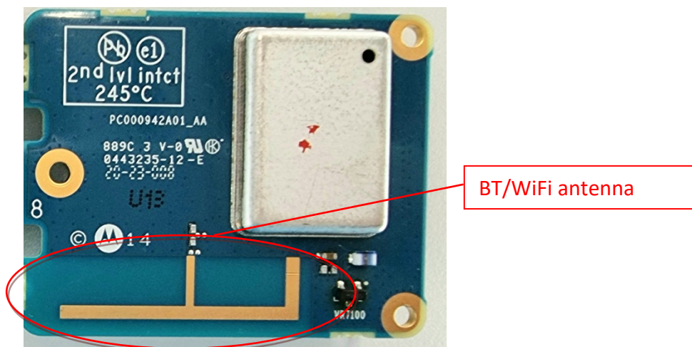
Expansion board with shield (Bottom)
