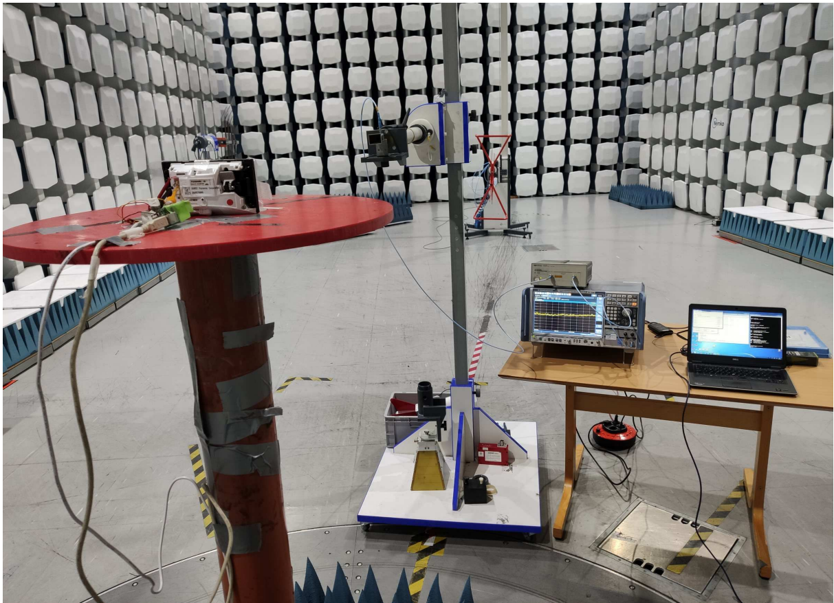
Radiated Emissions, 18 – 40 GHz
