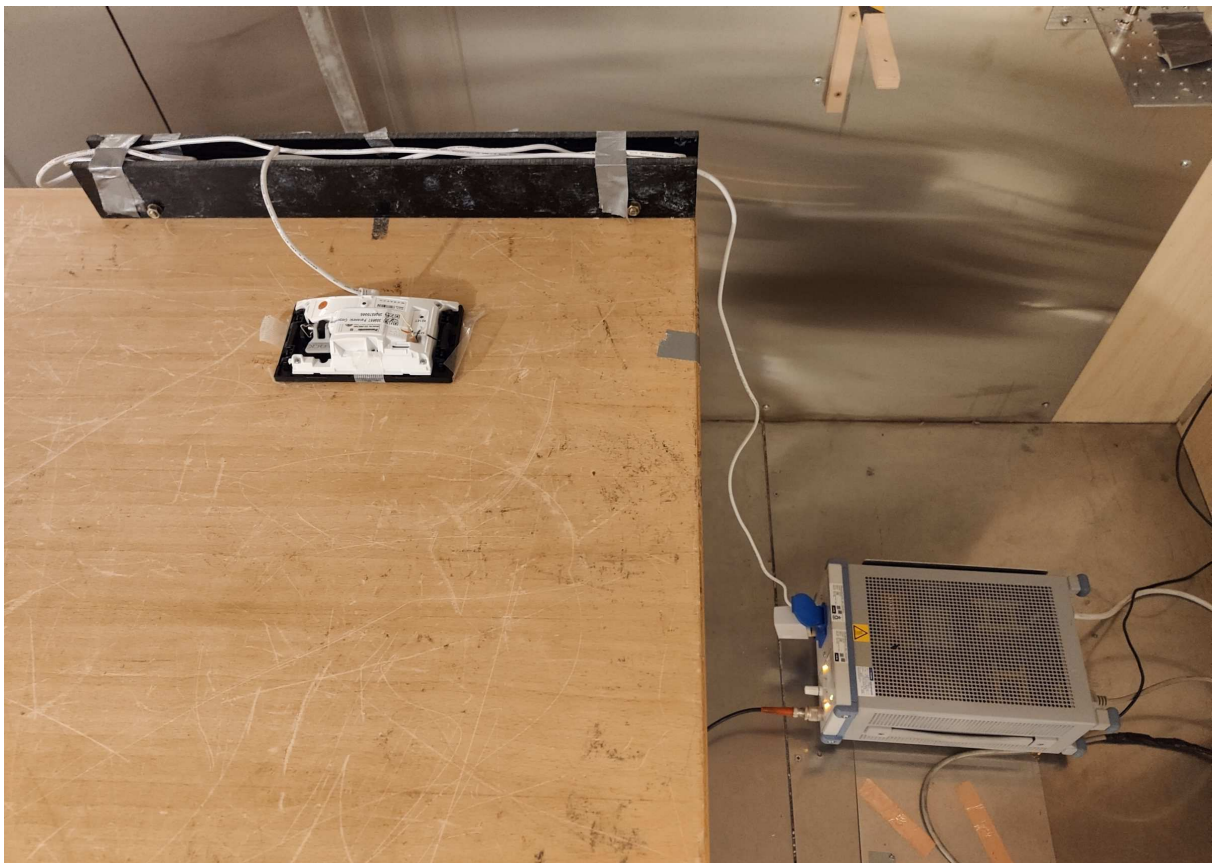
Power line Conducted Emissions Test
