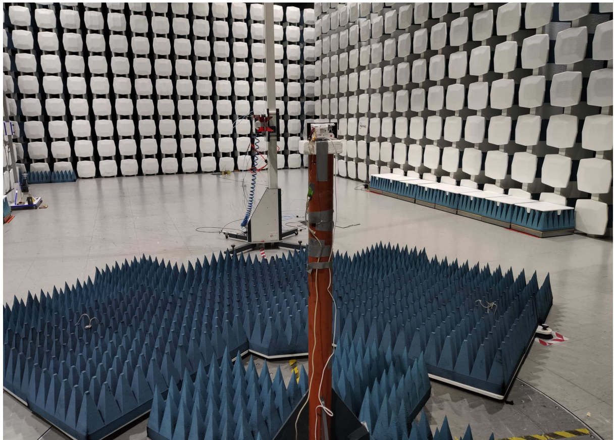
Radiated Emissions, 1 - 18 GHz
