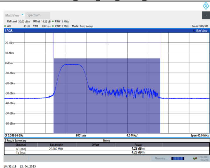
11AX20_Ant10_5600_106Tone_RU53
