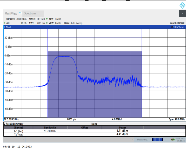
11AX20_Ant10_5200_106Tone_RU53
