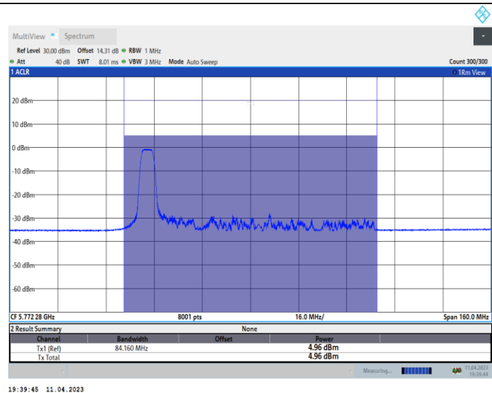
11AX80_Ant9_5775_106Tone_RU53
