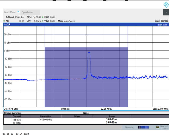
11AX160_Ant9_5250_UNII-1_106Tone_RU53
