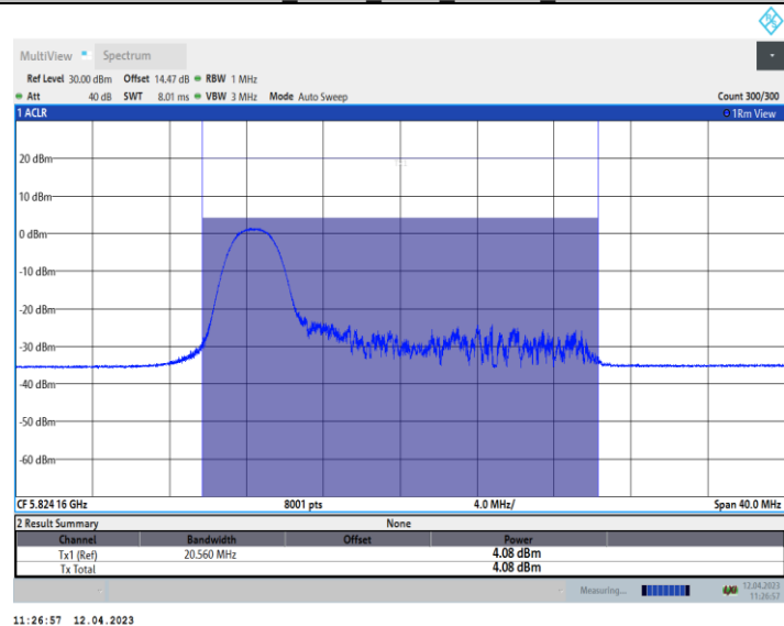
11AX20_Ant10_5825_52Tone_RU37
