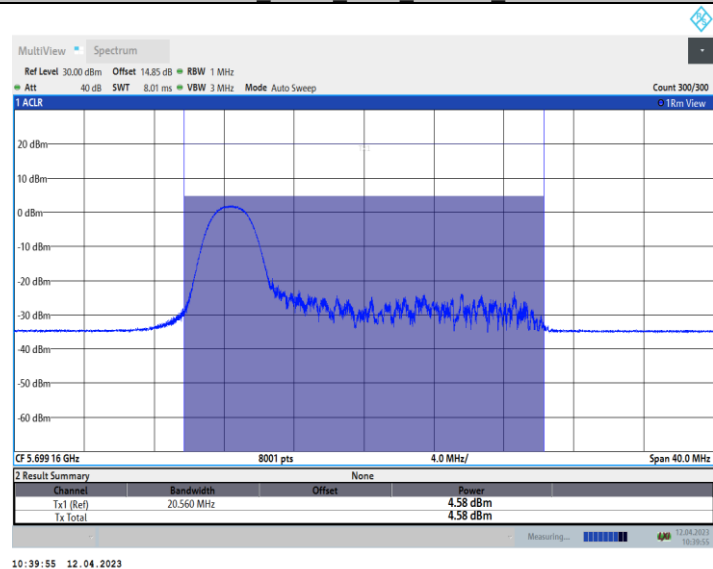
11AX20_Ant10_5700_52Tone_RU37
