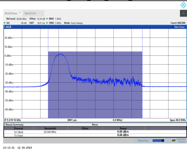
11AX20_Ant10_5320_52Tone_RU37
