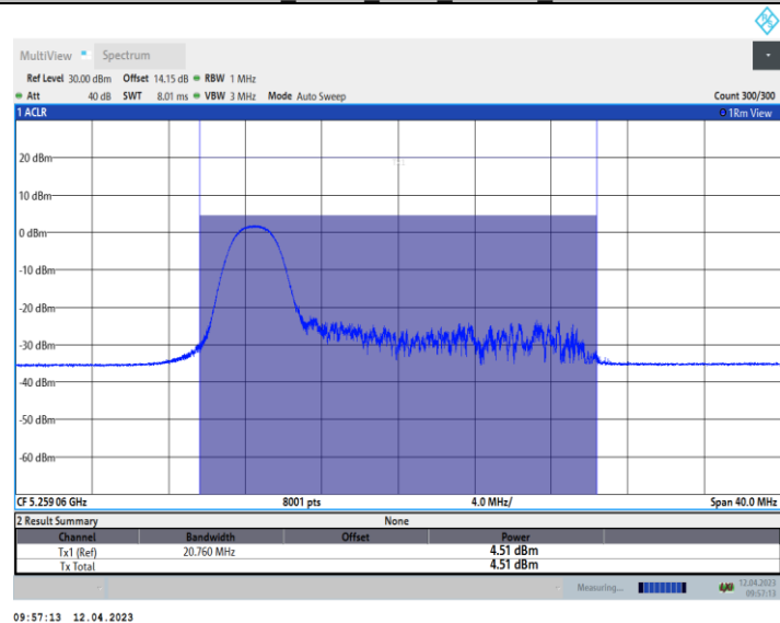
11AX20_Ant10_5260_52Tone_RU37
