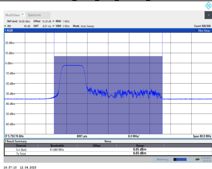
11AX40_Ant10_5755_242Tone_RU61
