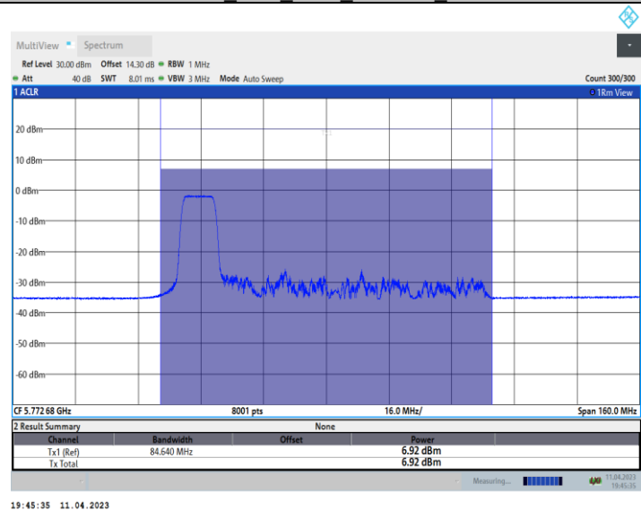
11AX80_Ant9_5775_242Tone_RU61
