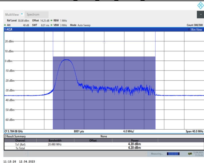
11AX20_Ant10_5785_52Tone_RU37
