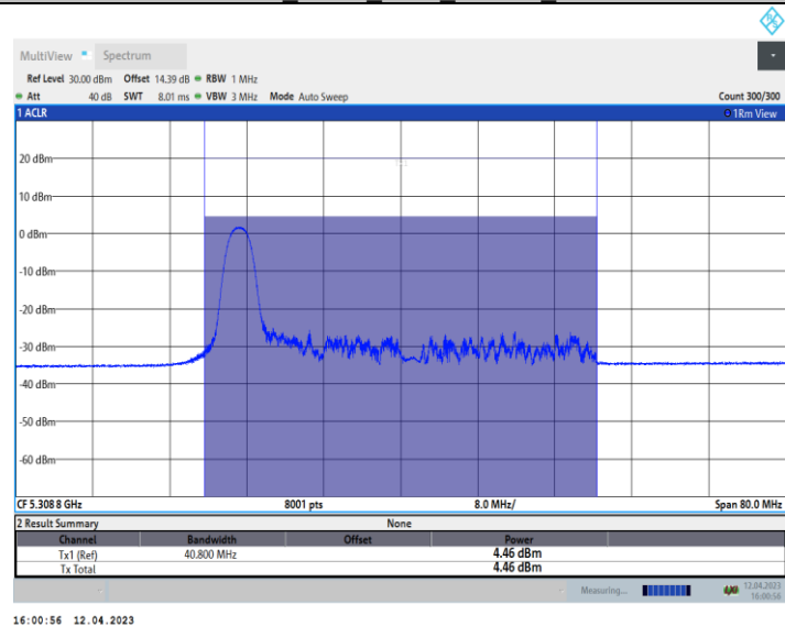
11AX40_Ant10_5310_52Tone_RU37
