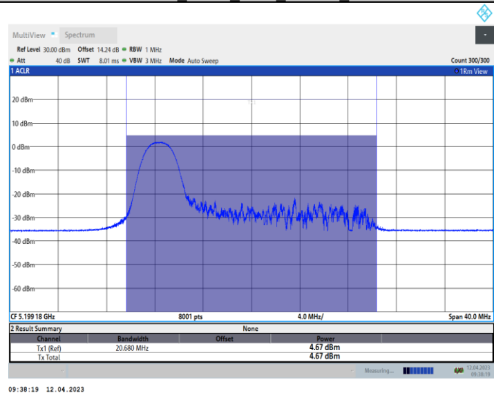
11AX20_Ant10_5200_52Tone_RU37
