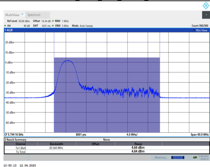
11AX20_Ant10_5745_52Tone_RU37
