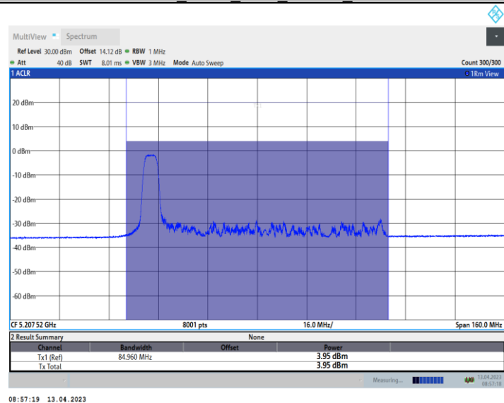
11AX80_Ant10_5210_106Tone_RU53
