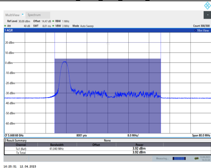
11AX40_Ant10_5670_52Tone_RU37
