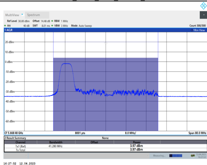
11AX40_Ant10_5670_106Tone_RU53
