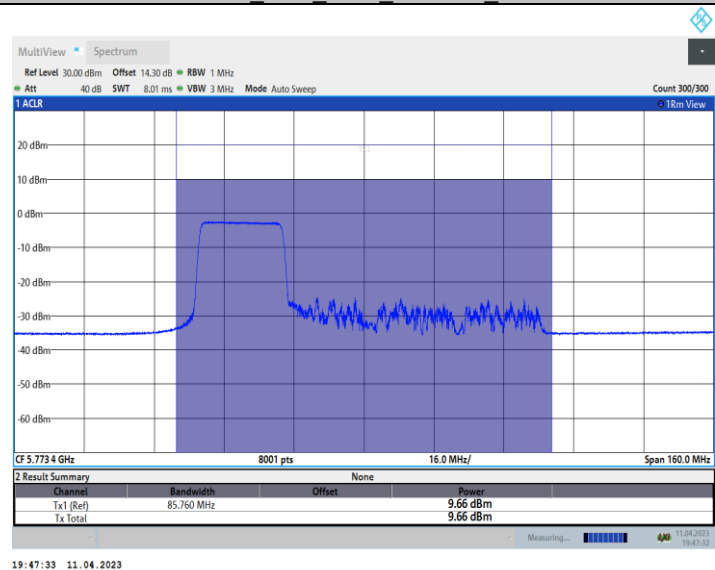
11AX80_Ant9_5775_484Tone_RU65
