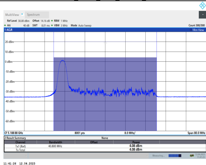
11AX40_Ant10_5190_52Tone_RU37
