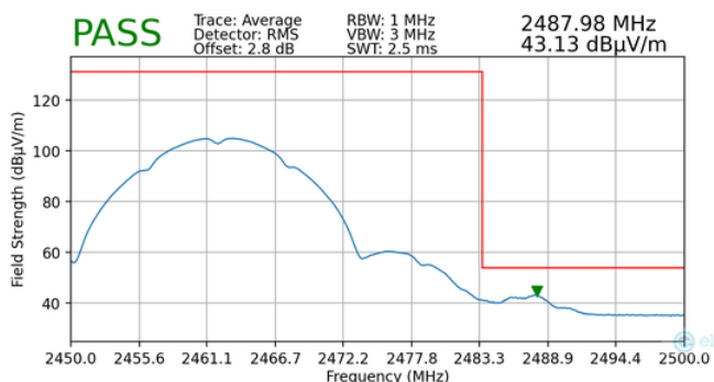
Plot 7-140. Radiated Restricted Upper Band Edge Measurement MIMO (Average)
