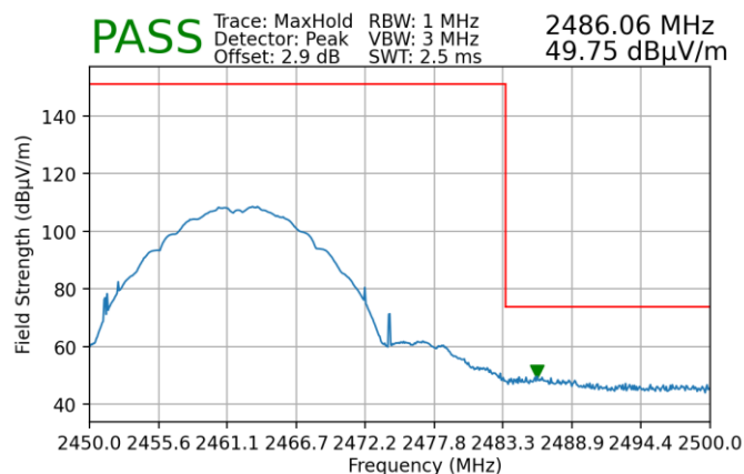
Plot 7-147. Radiated Restricted Band Edge Measurement MIMO with WCP (Peak)
