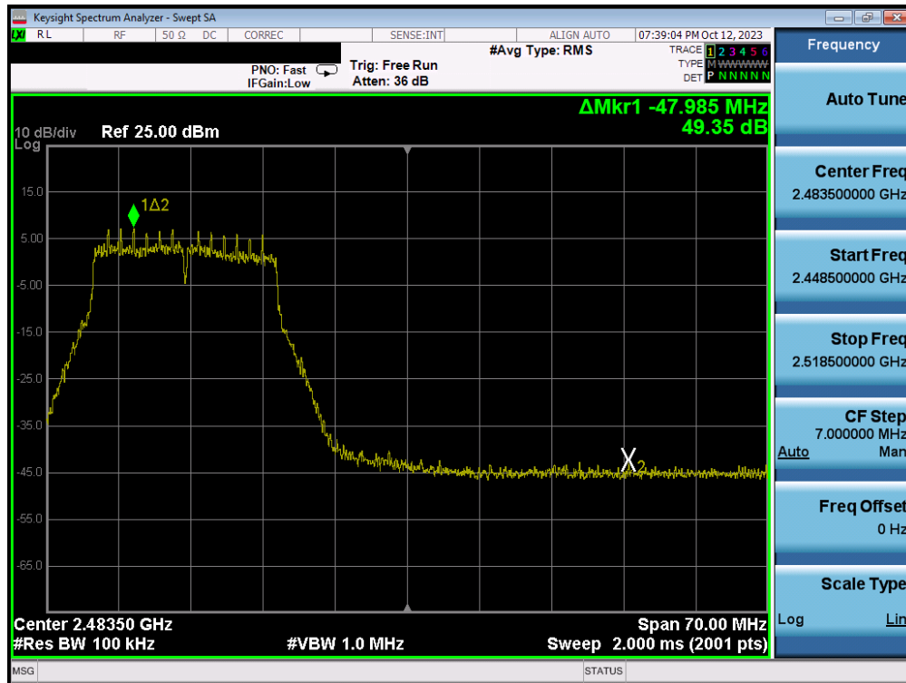
Plot 7-106. Band Edge Plot MIMO ANT2 (802.11n (2.4GHz) – Ch. 11)
