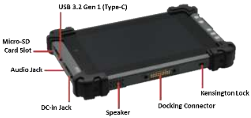
Side View (Bottom-Left)
