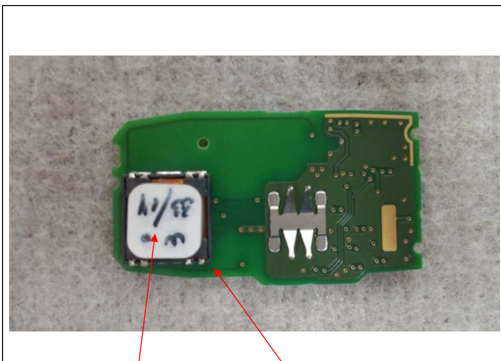
RX Antenna
