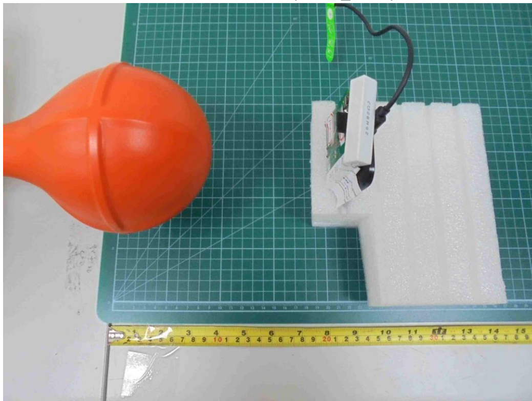
E-Field and H-Field (Z-axis_20cm)
