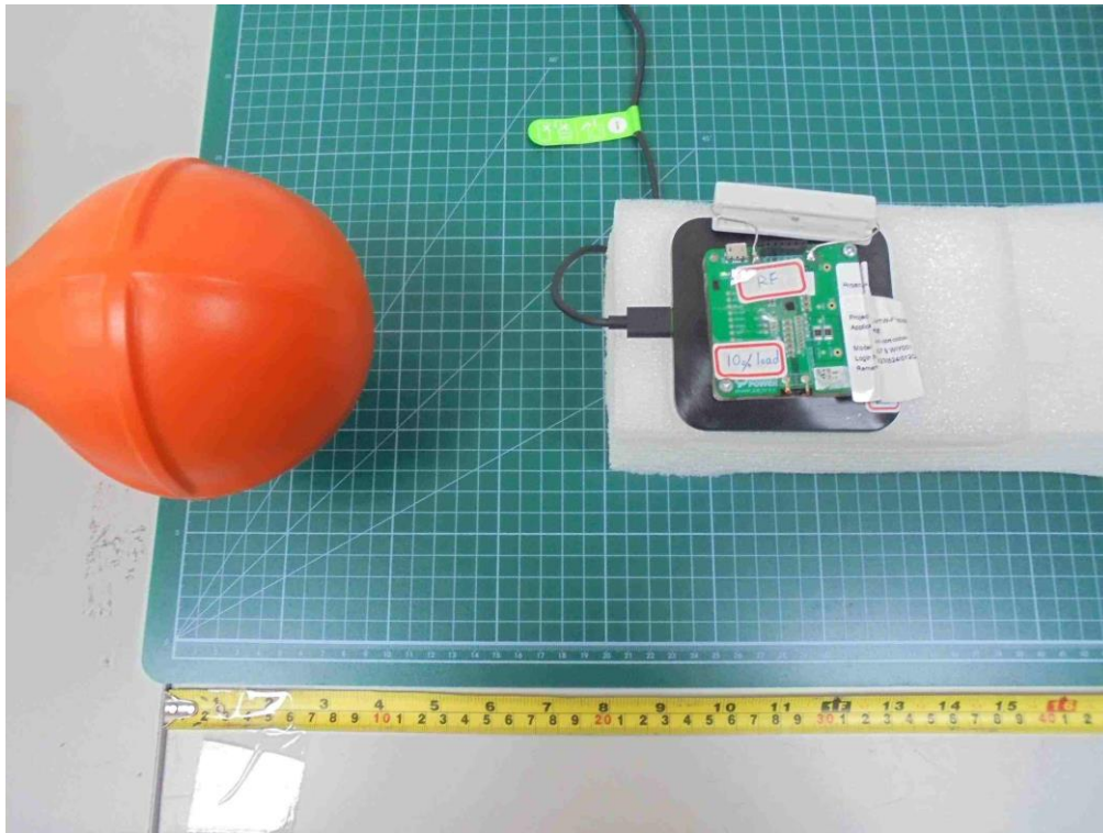
E-Field and H-Field (Left_20cm)
