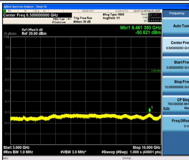
Band17_10MHz_16QAM_23780_1RB#0_3000~10000_3000~10000
