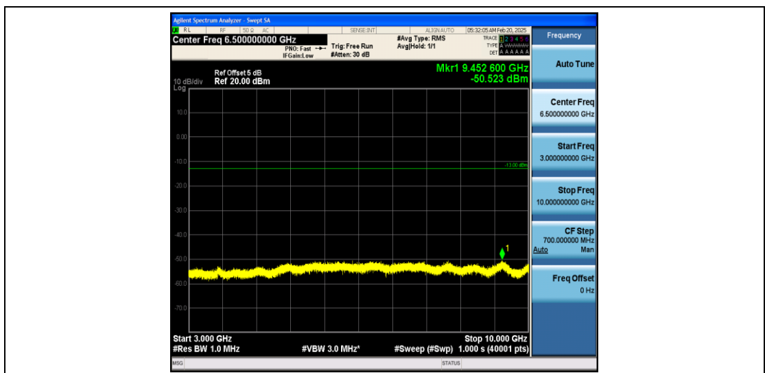
Band17_5MHz_QPSK_23755_1RB#0_3000~10000_3000~10000
