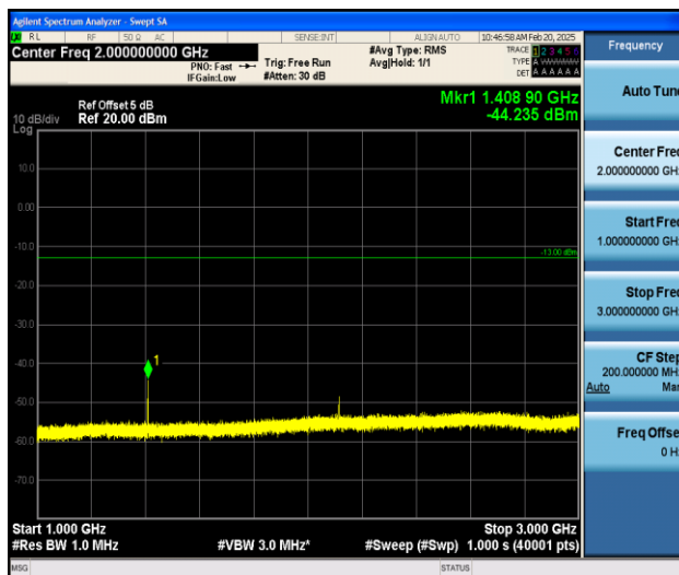
Band17_10MHz_16QAM_23780_1RB#0_1000~3000_1000~3000
