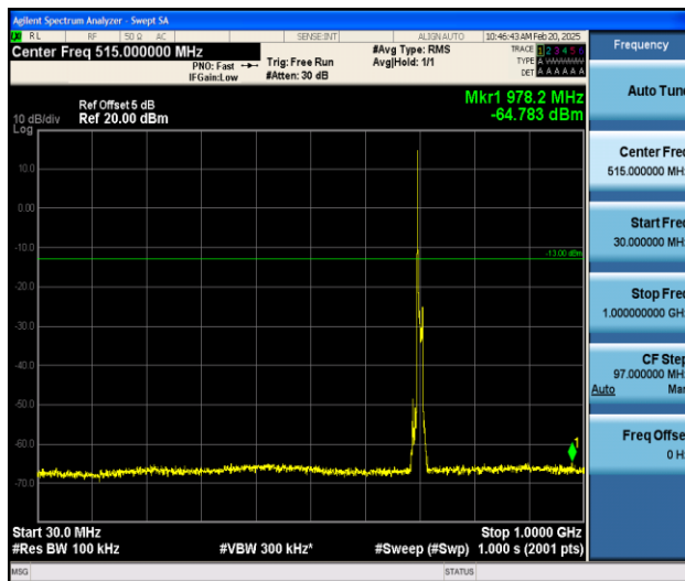
Band17_10MHz_16QAM_23780_1RB#0_30~1000_30~1000
