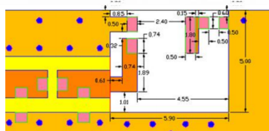
Antenna Layout Reference
