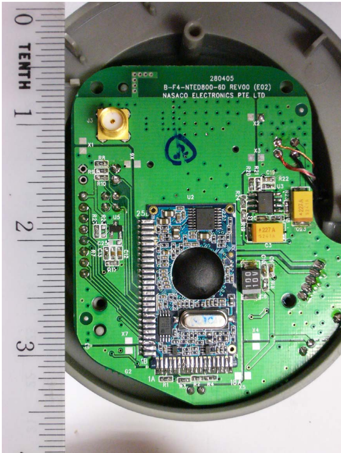
EUT Main Board - Top View
