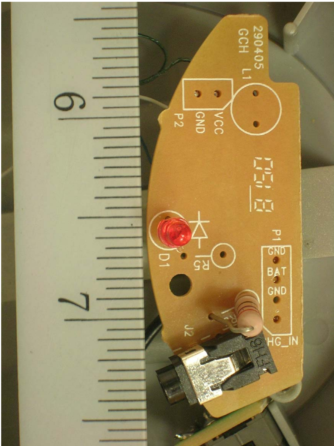
EUT Charger Circuit - Component Side
