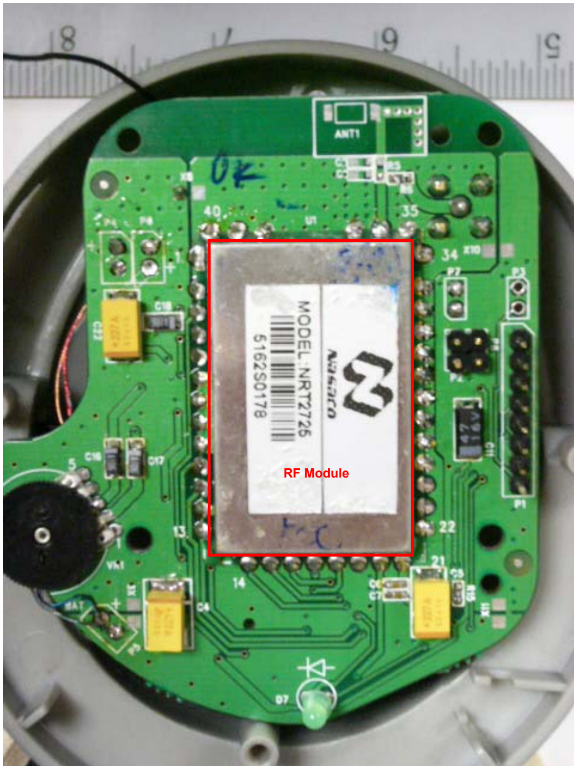
EUT Main Board - Bottom View
