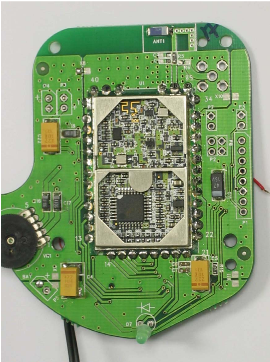
RF Module Circuit with RF Shield Removed
