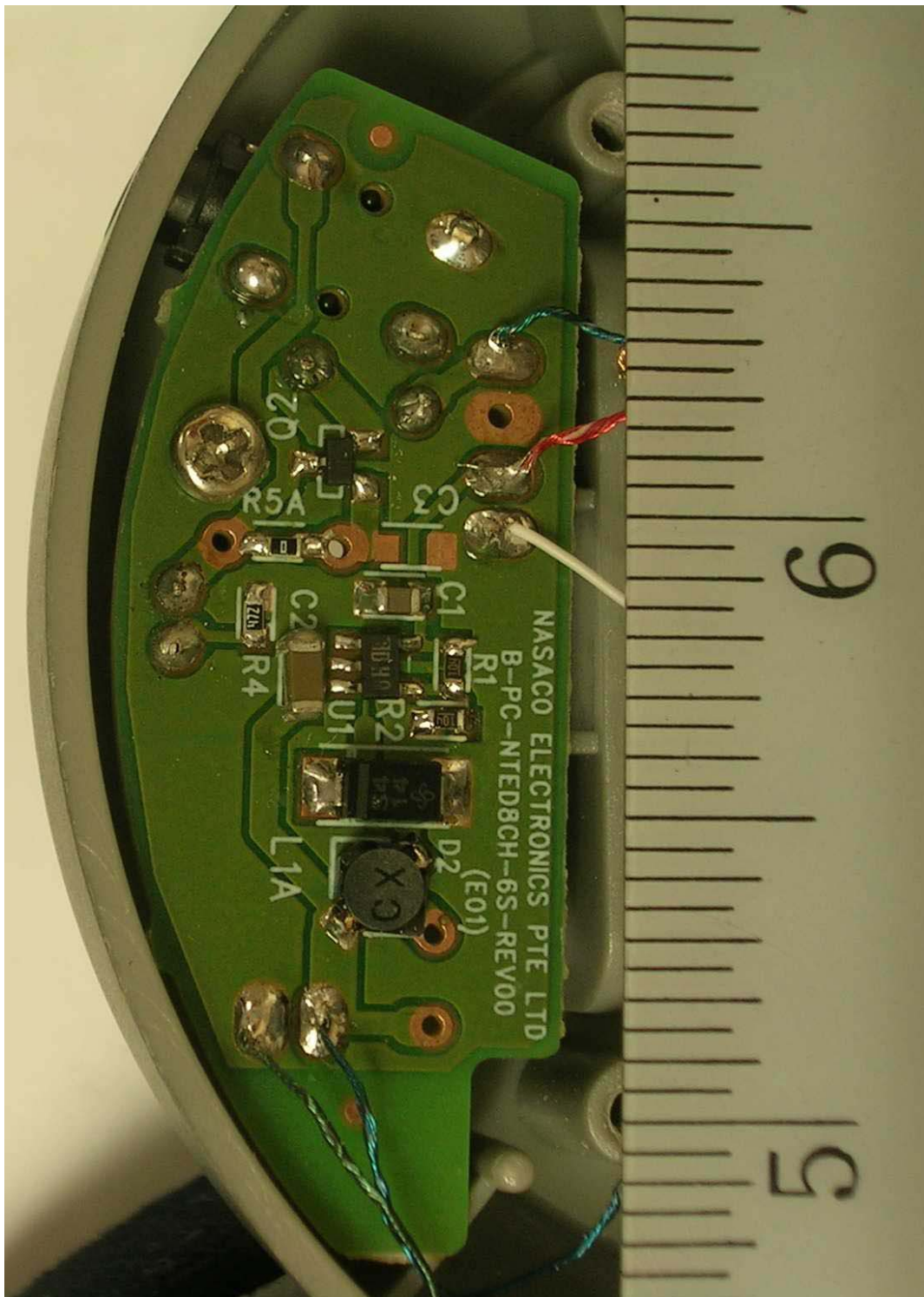
EUT Charger Circuit - Trace Side
